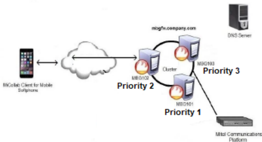
Figure 2: Softphone Resiliency in Cloud Deployment
