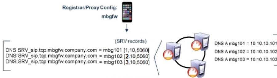
Figure 3: DNS SRV Entries for Resilient Softphones in Cloud Deployment
