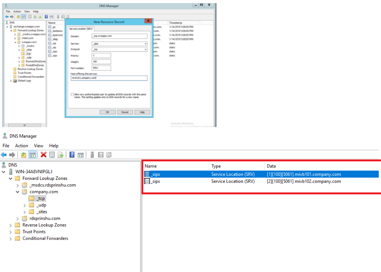
Figure 10: DNS Server Configuration Settings
