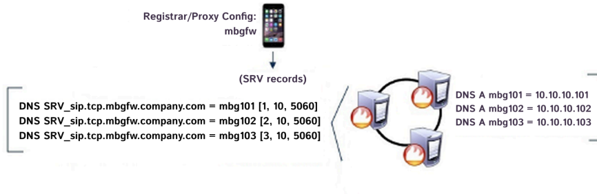
Figure 2: DNS SRV Entries for Resilient Softphones in Cloud Deployment
