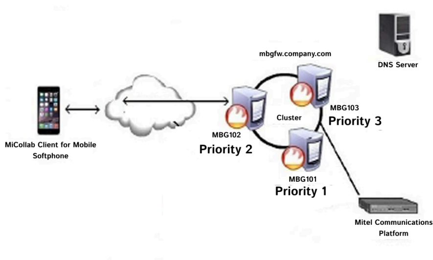
Figure 1: Softphone Resiliency in Cloud Deployment
