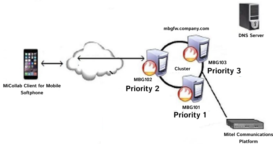
Figure 1: Softphone Resiliency in Cloud Deployment
