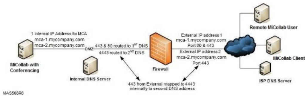
Figure 6: AWV Firewall Configuration
