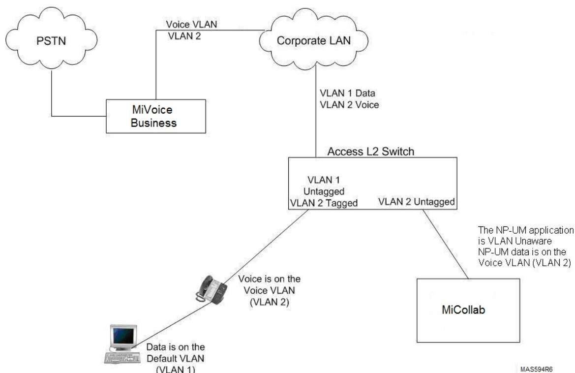
Figure 15: NP-UM LAN Integration
