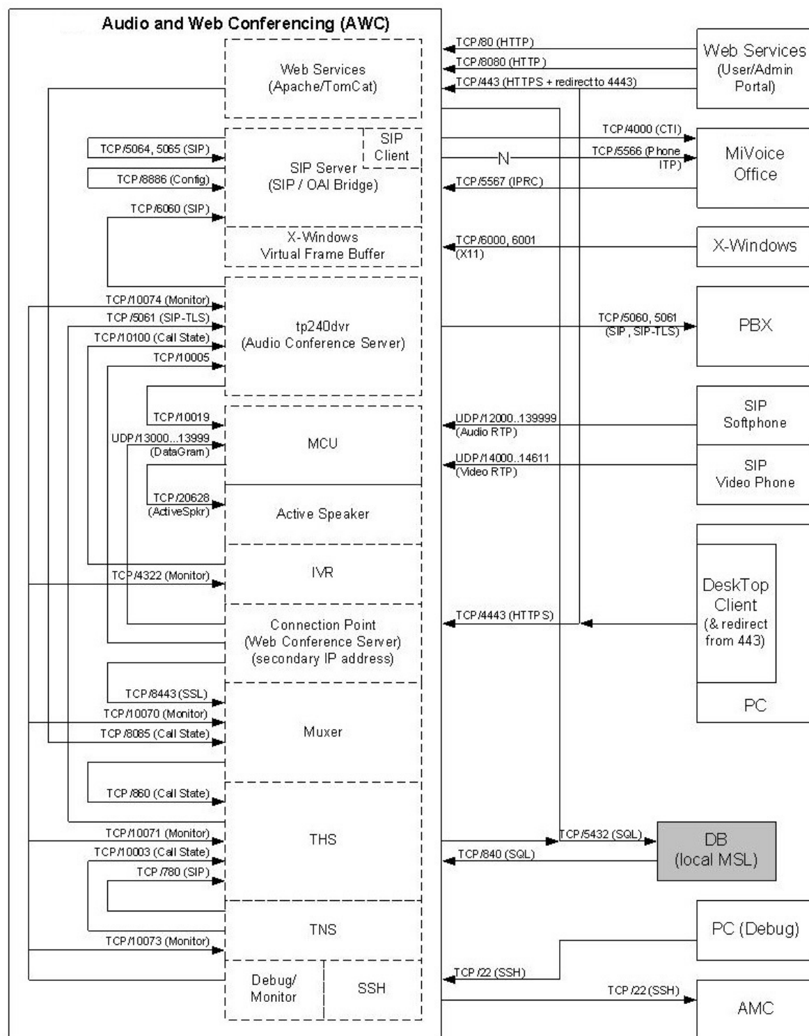
Figure 29: Audio, Web and Video Ports
