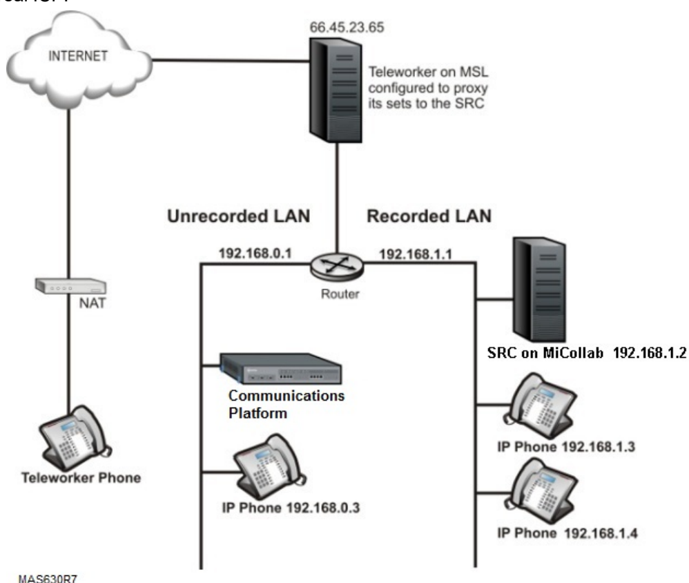
Figure 19: Recording Teleworker Sets
