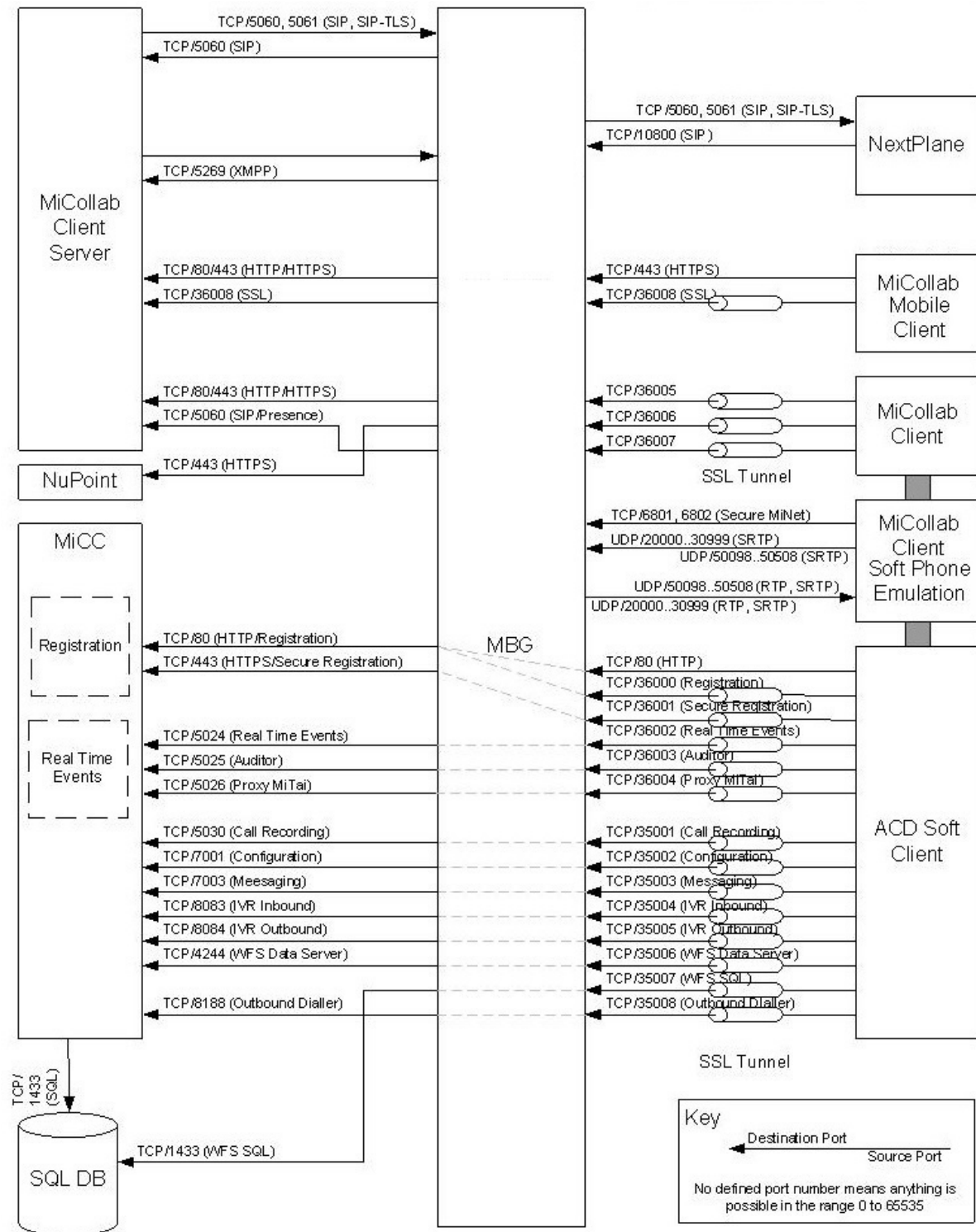
Figure 28: MiVoice Border Gateway Ports (Diagram 3)
