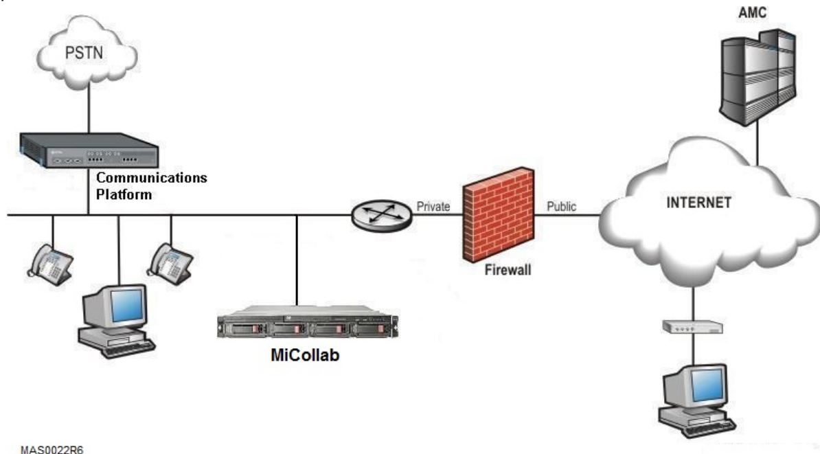
Figure 5: MiCollab Server in LAN Mode
