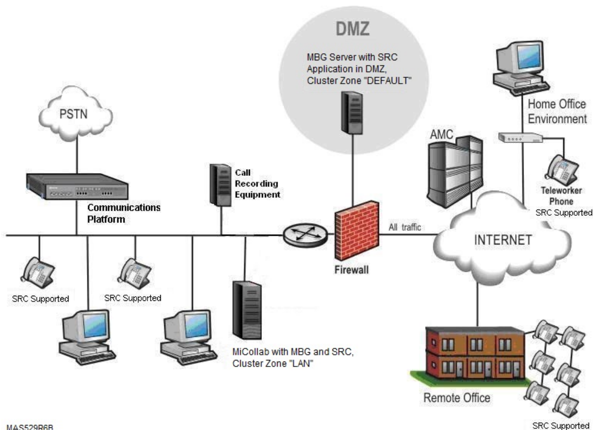
Figure 8: MiCollab/MiCollab Virtual Appliance with SRC in LAN Mode with MBG Server with SRC in DMZ
