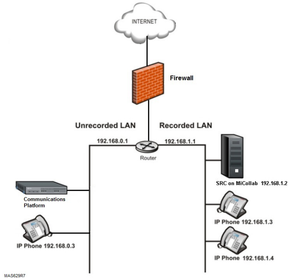
Figure 18: Sample Call Recording Deployment
