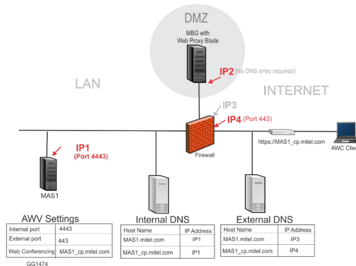
Figure 2: MiCollab AWW External IP address Handling with Web Proxy (two external IPs)
