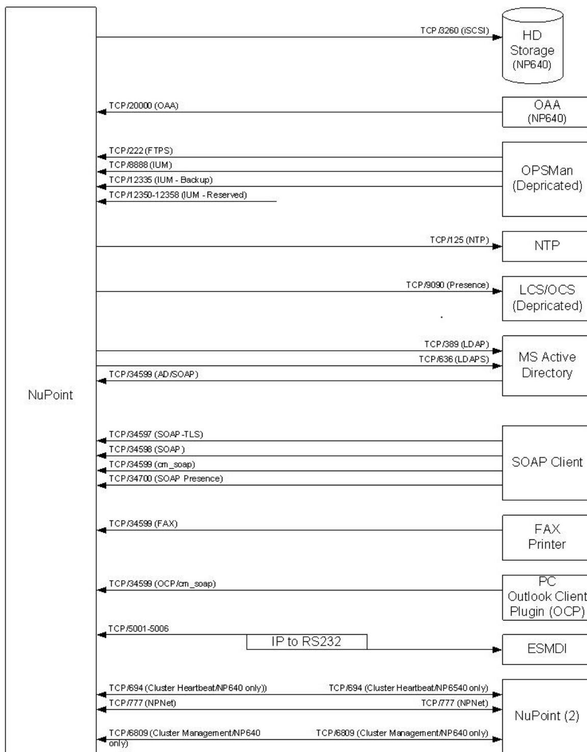
Figure 25: NuPoint Unified Messaging Ports (Diagram 2)
