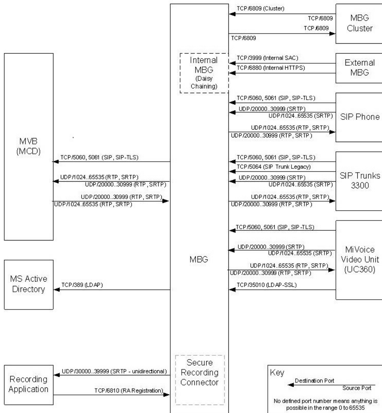
Figure 27: MiVoice Business Gateway (Diagram 2)
