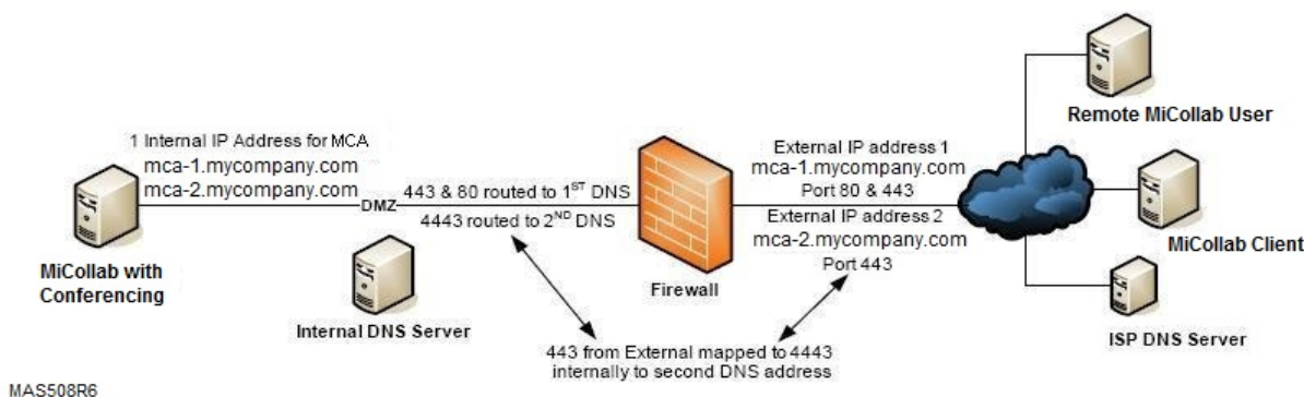
Figure 6: AWW Firewall Configuration
