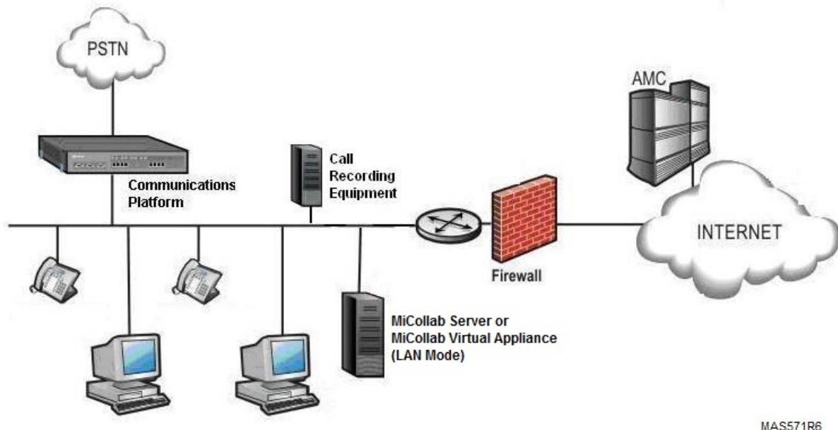
Figure 7: MiCollab Server or MiCollab Virtual Appliance with SRC in LAN Mode
