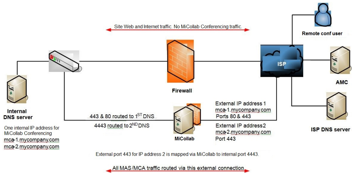
Figure 22: AWV (Network Edge)
