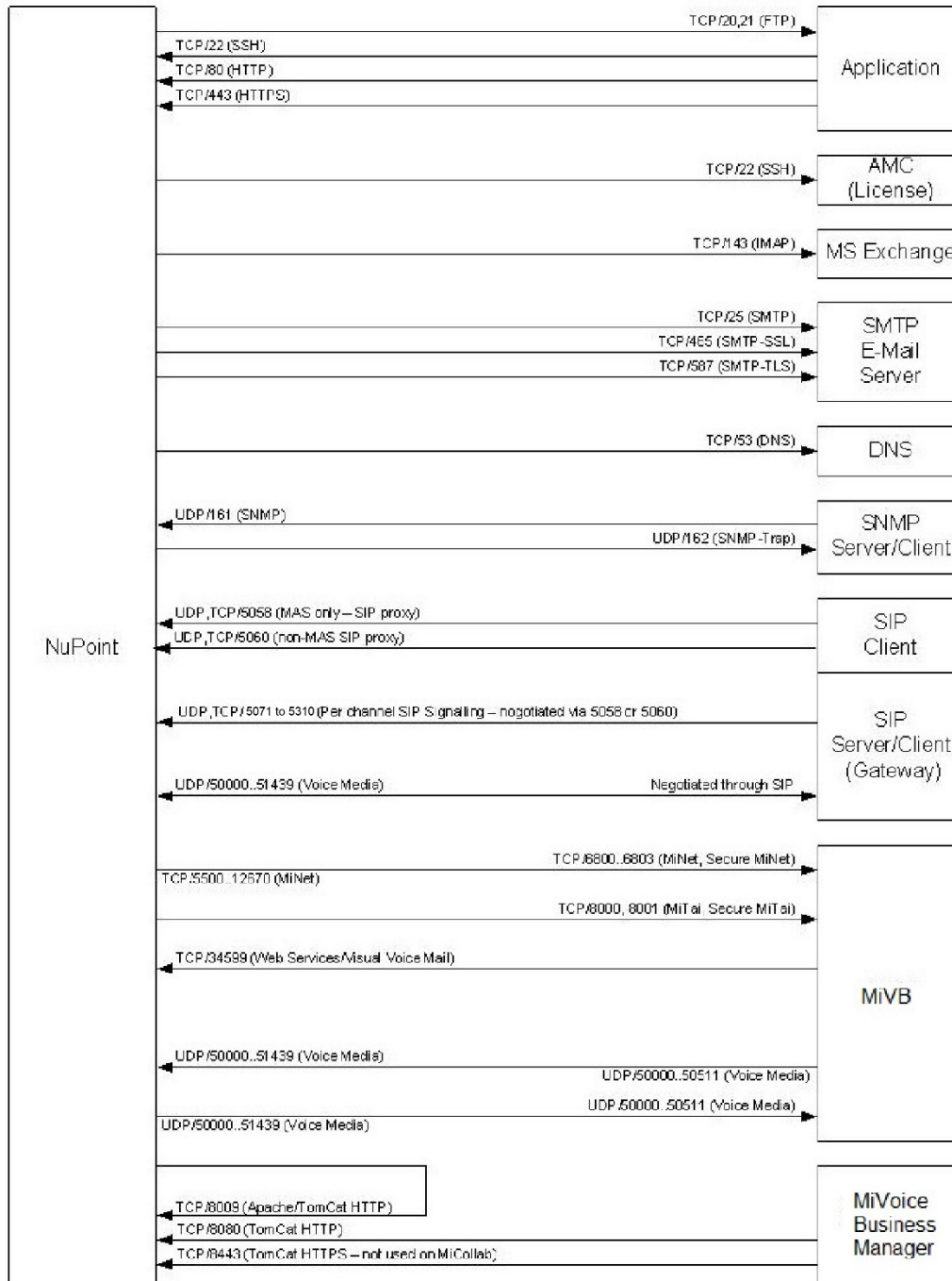
Figure 24: NuPoint Unified Messaging Ports (Diagram 1)
