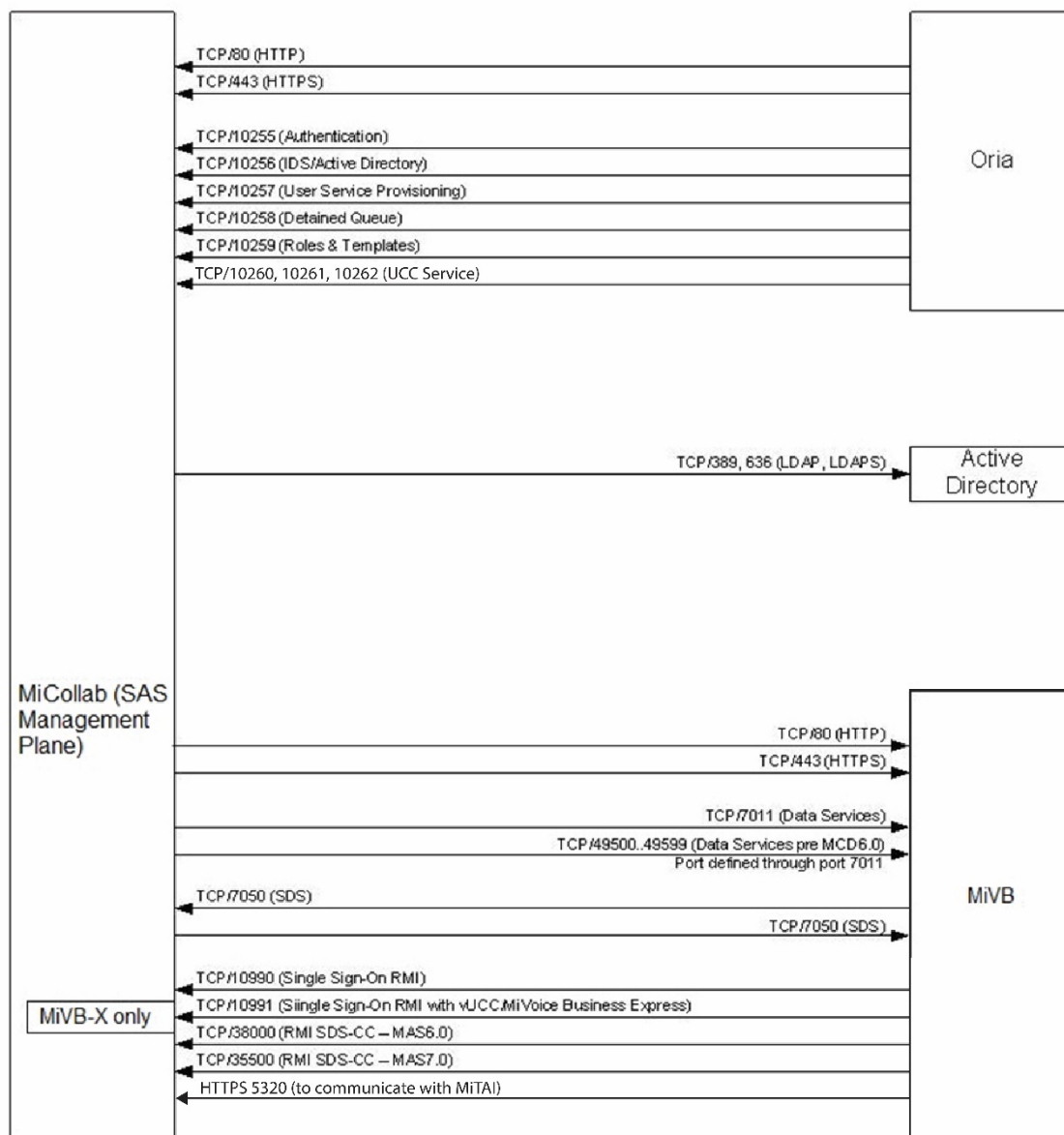
Figure 23: MiCollab Port Usage
