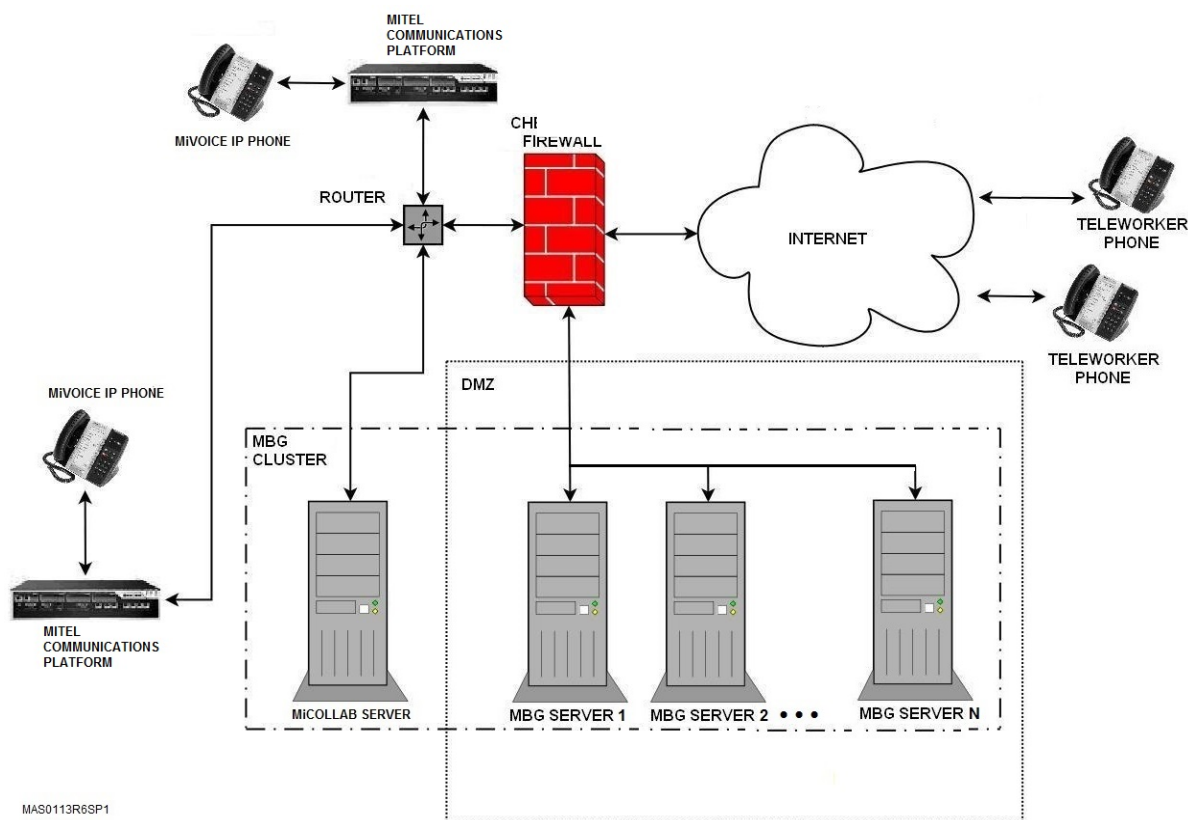
Figure 4: MiCollab with MBG Teleworker & Web Proxy
