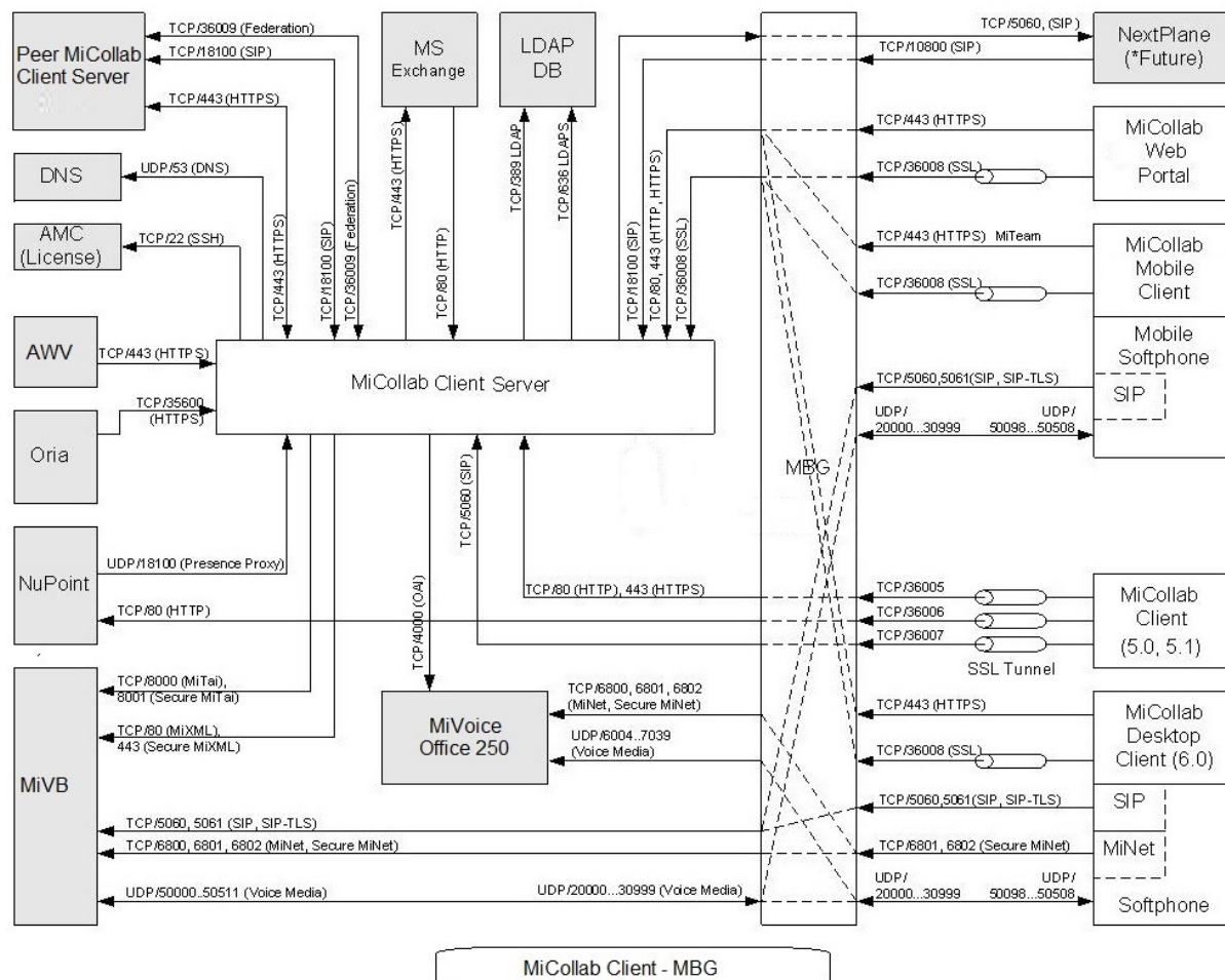
Figure 31: MiCollab Client Ports (LAN Mode)
