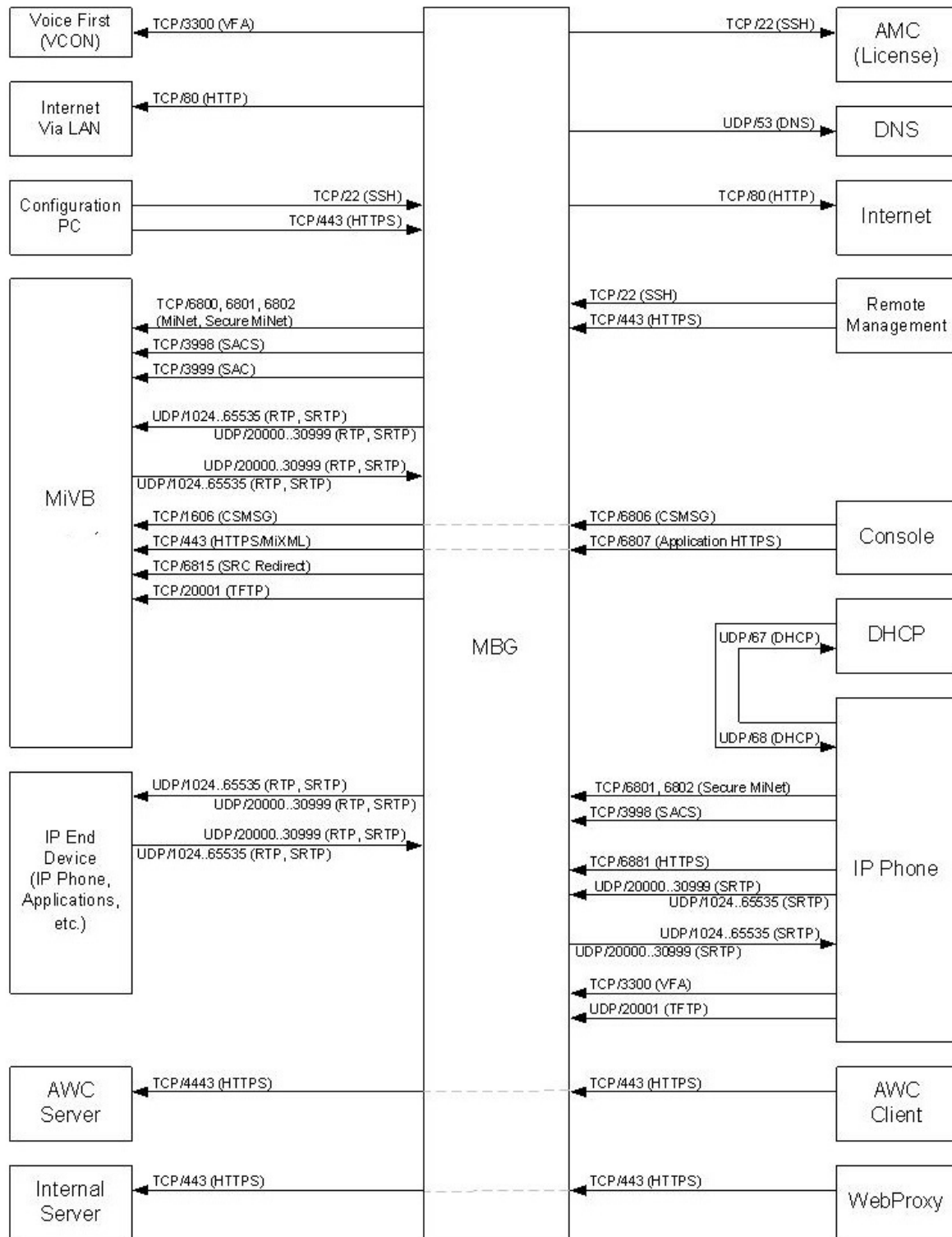
Figure 26: MiVoice Business Gateway Port Usage (Diagram 1)
