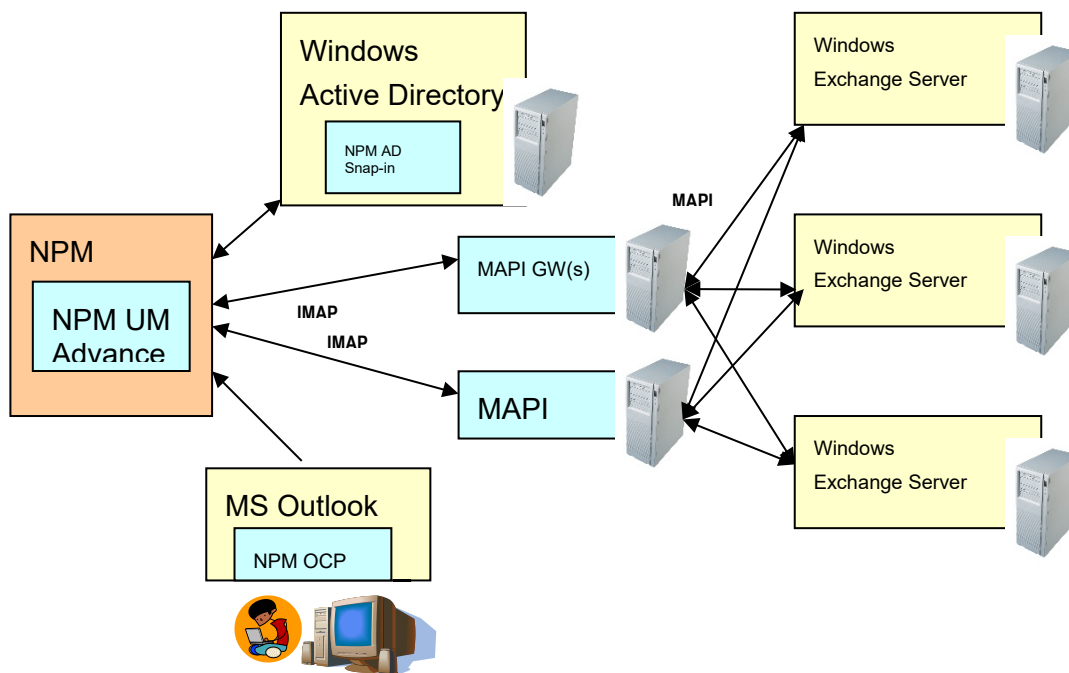
Figure 17: NP-UM Advanced UM with MAPI Integration
