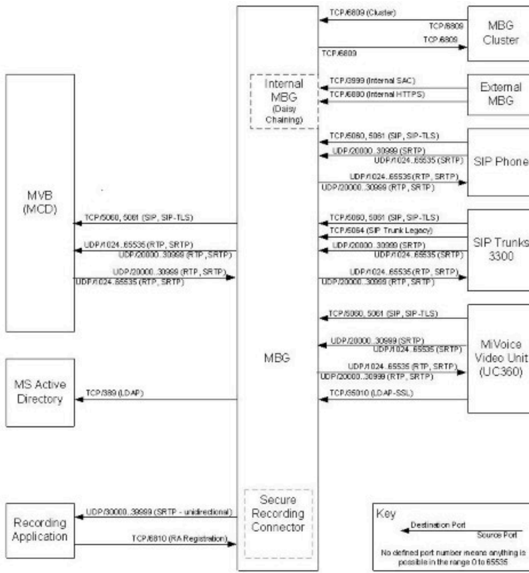
Figure 24: MiVoice Border Gateway Ports (Diagram 3)
