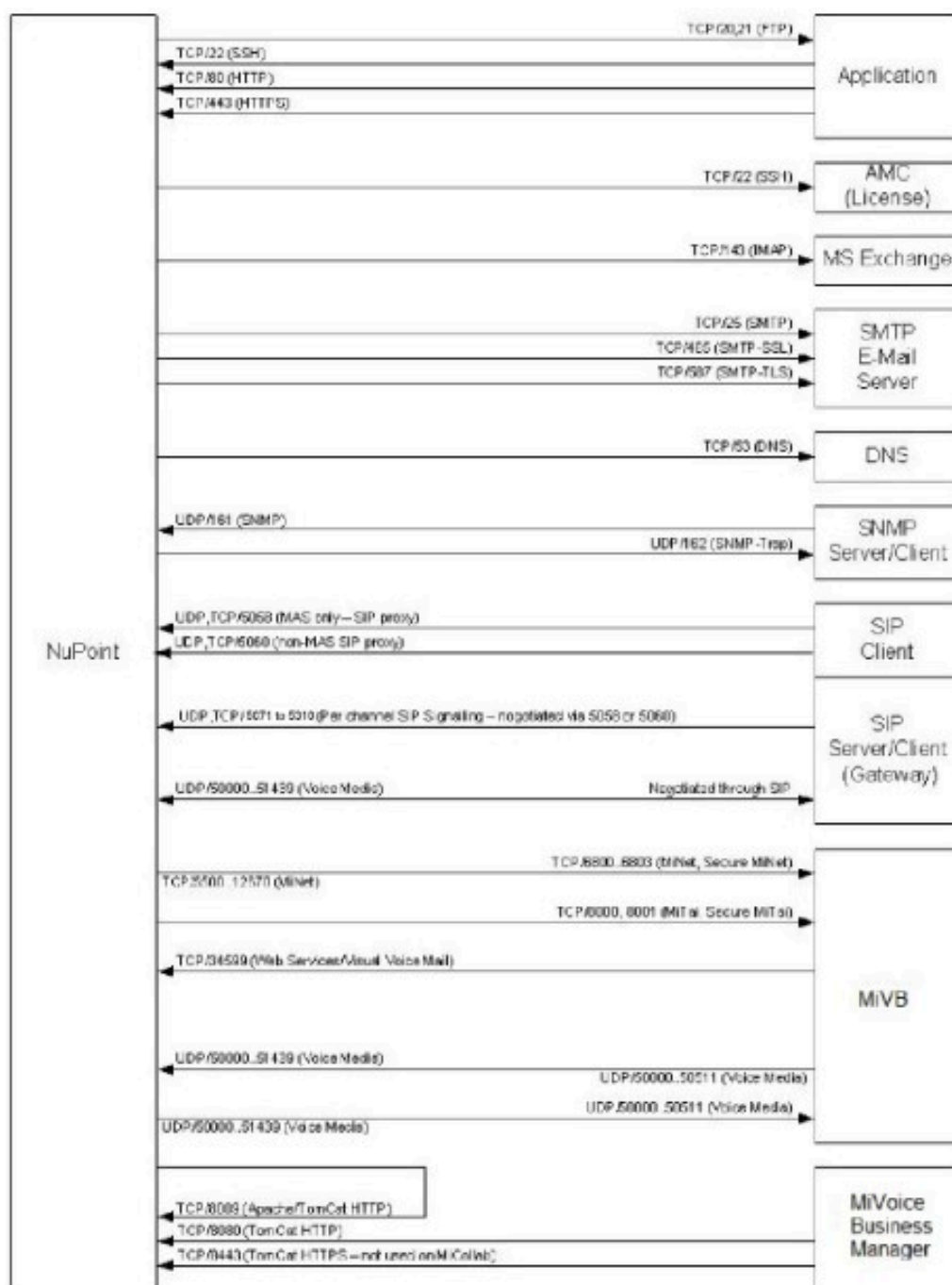
Figure 21: NuPoint Unified Messaging Ports (Diagram 2)
