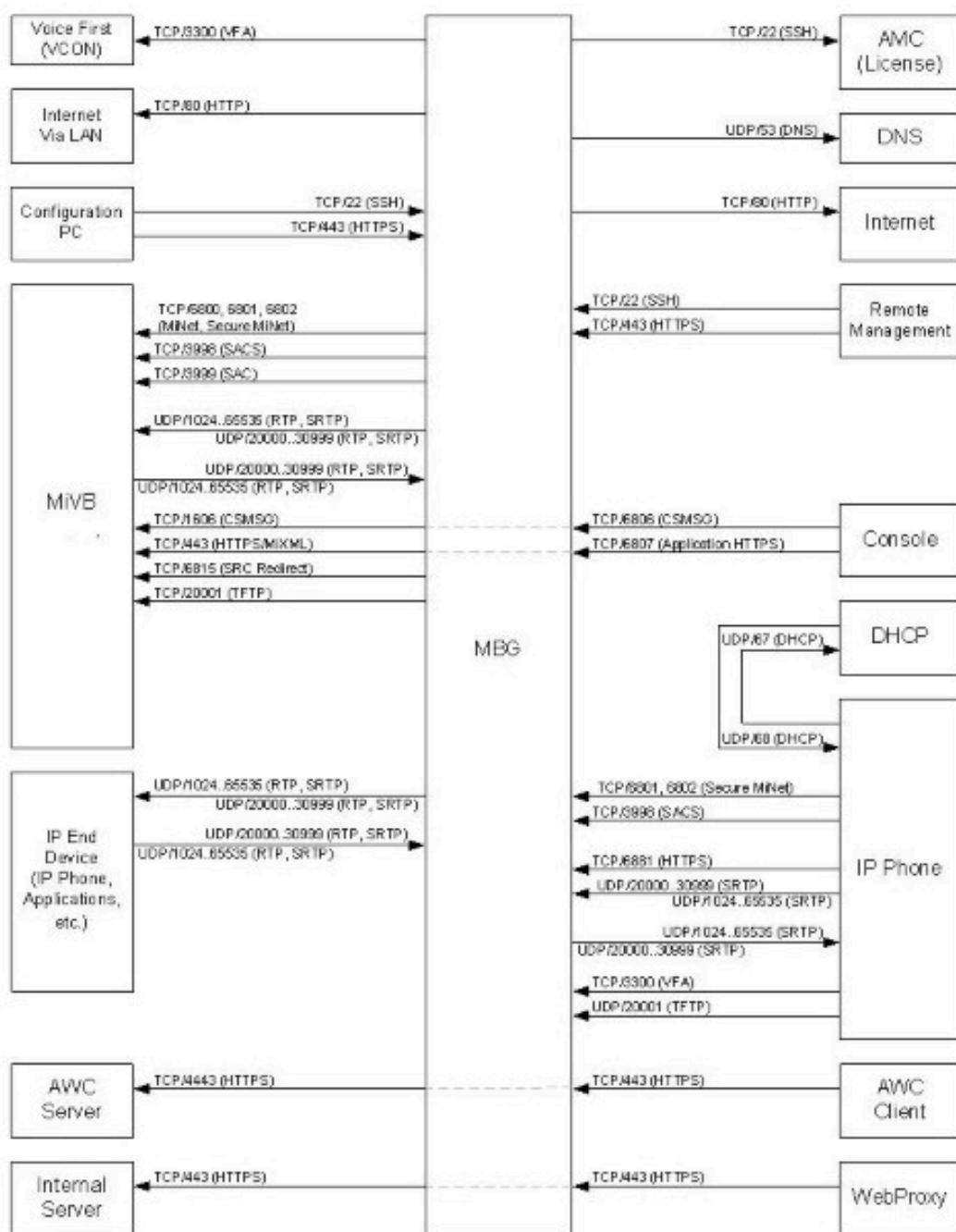
Figure 23: MiVoice Business Gateway (Diagram 2)
