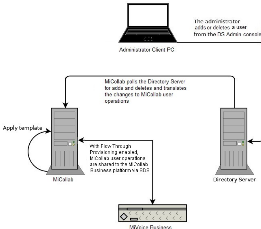
Figure 9: MiCollab and MiVoice Business (s) with Flow Through Provisioning
