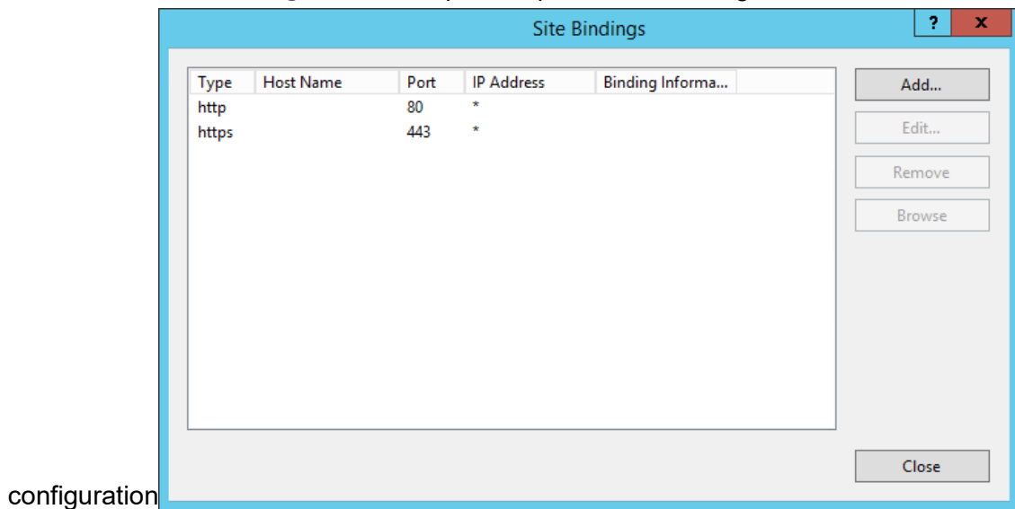
Figure 4.4: Sample completed site bindings
