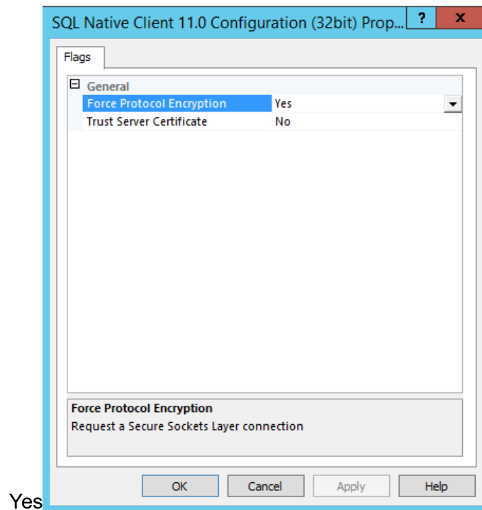
Figure 6.3: Native client protocol Force Protocol Encryption flag set to
