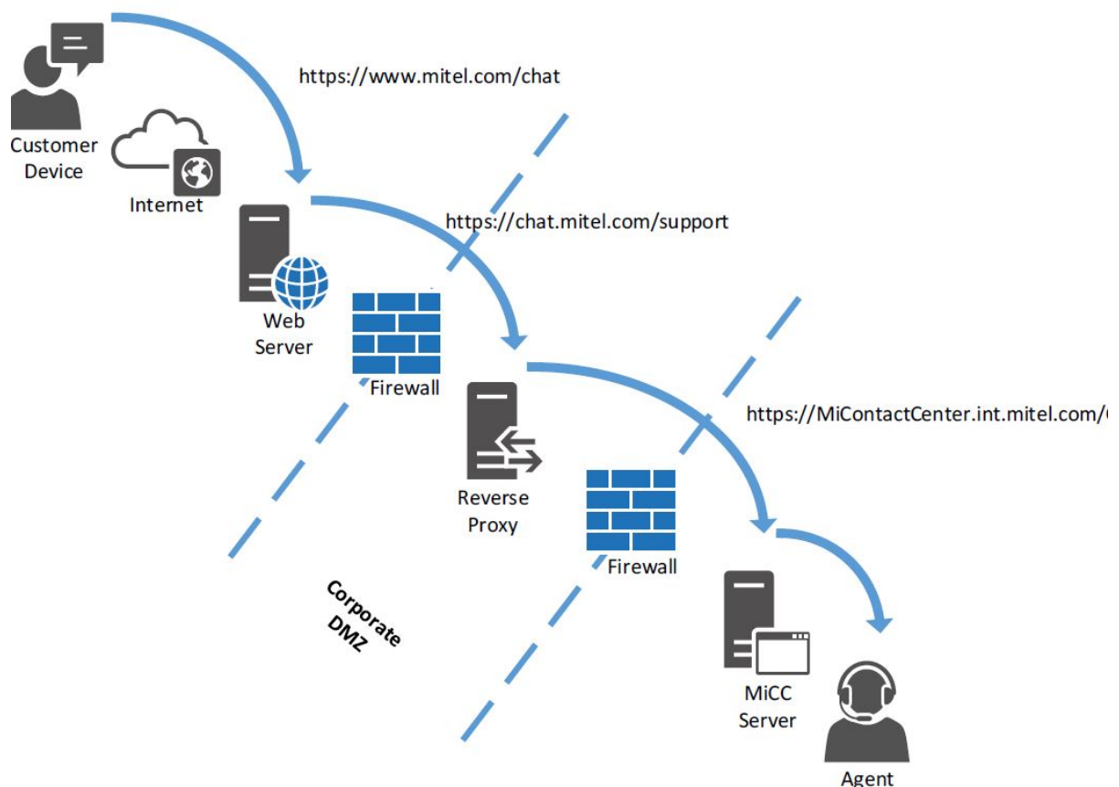
Figure 5.1: A sample reverse proxy with DMZ implementation
