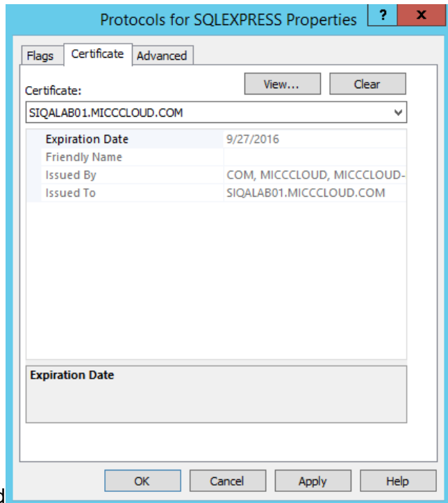
Figure 6.2: The server certificate applied
