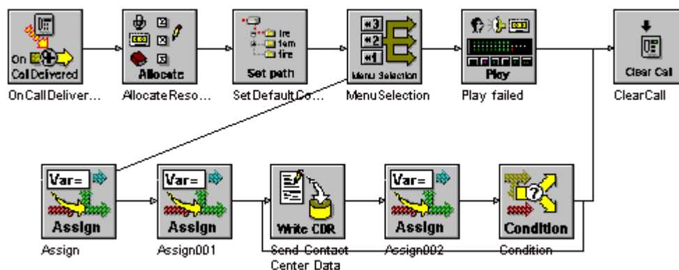
Figure 1: Logon Script
