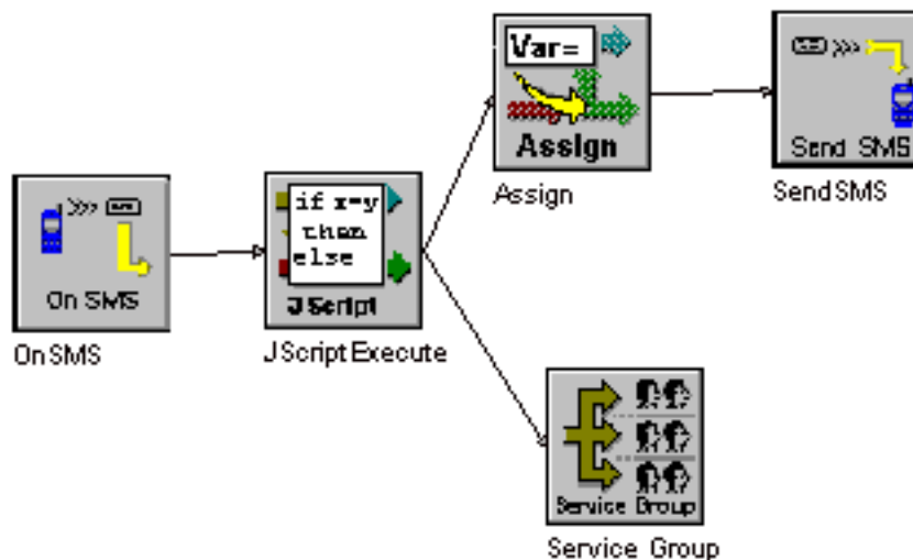
Figure 12: Incoming SMS
