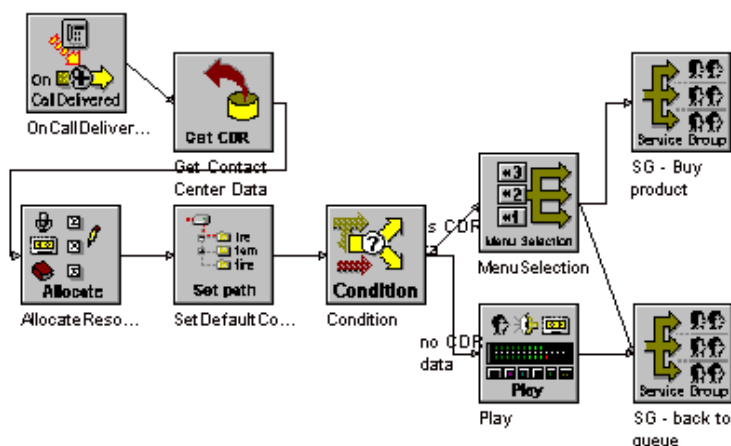
Figure 18: IVR Queue
