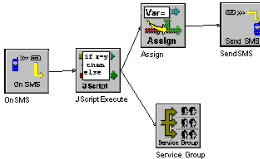
Figure 12: Incoming SMS
