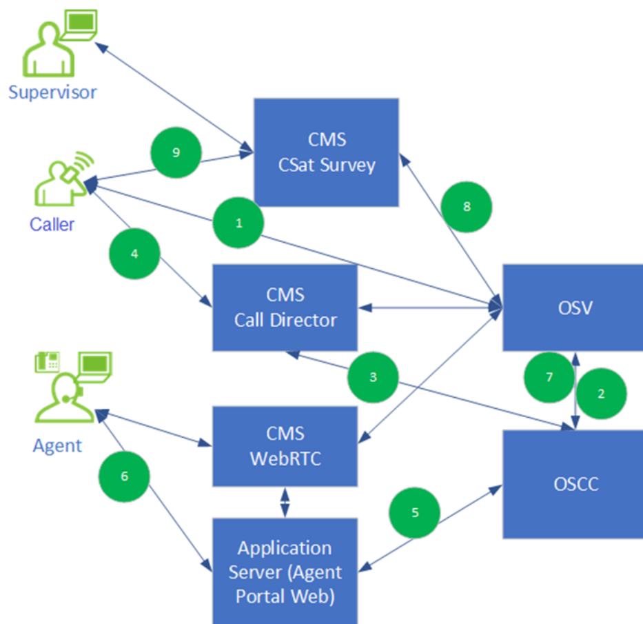
Figure 2: Operating mode with OSCC Call Director integration
