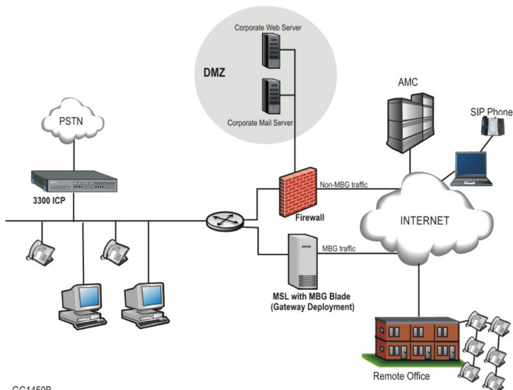
Figure 1. Server-Gateway Configuration
