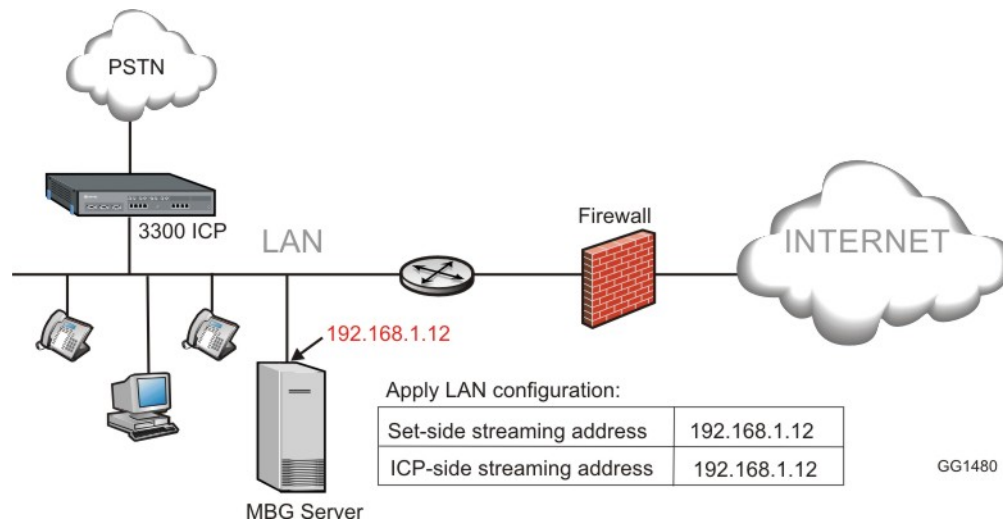
Figure 3. Server-only Configuration
