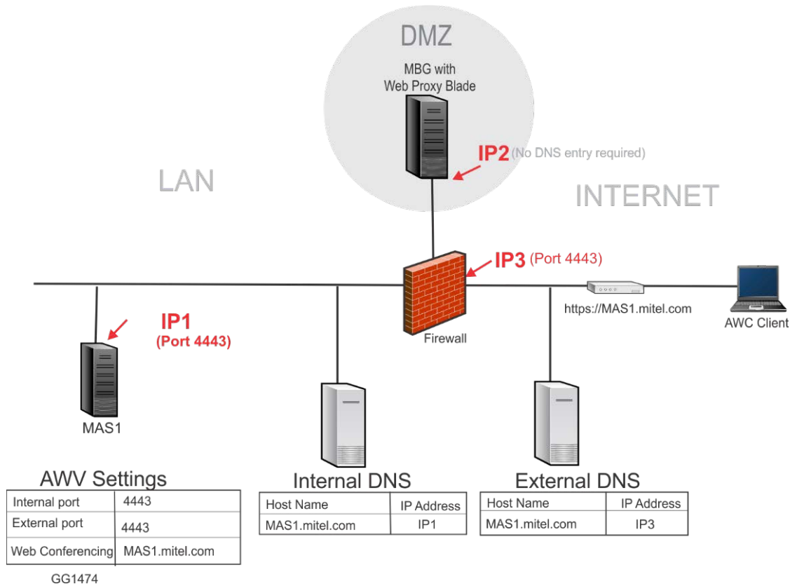
Figure 13: AWC Configuration with Dedicated TCP Port on Primary External IP Address
