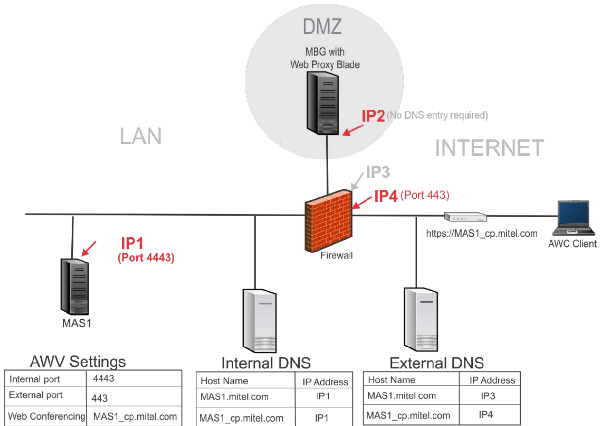
Figure 12. AWV Configuration with Additional Dedicated External IP Address
