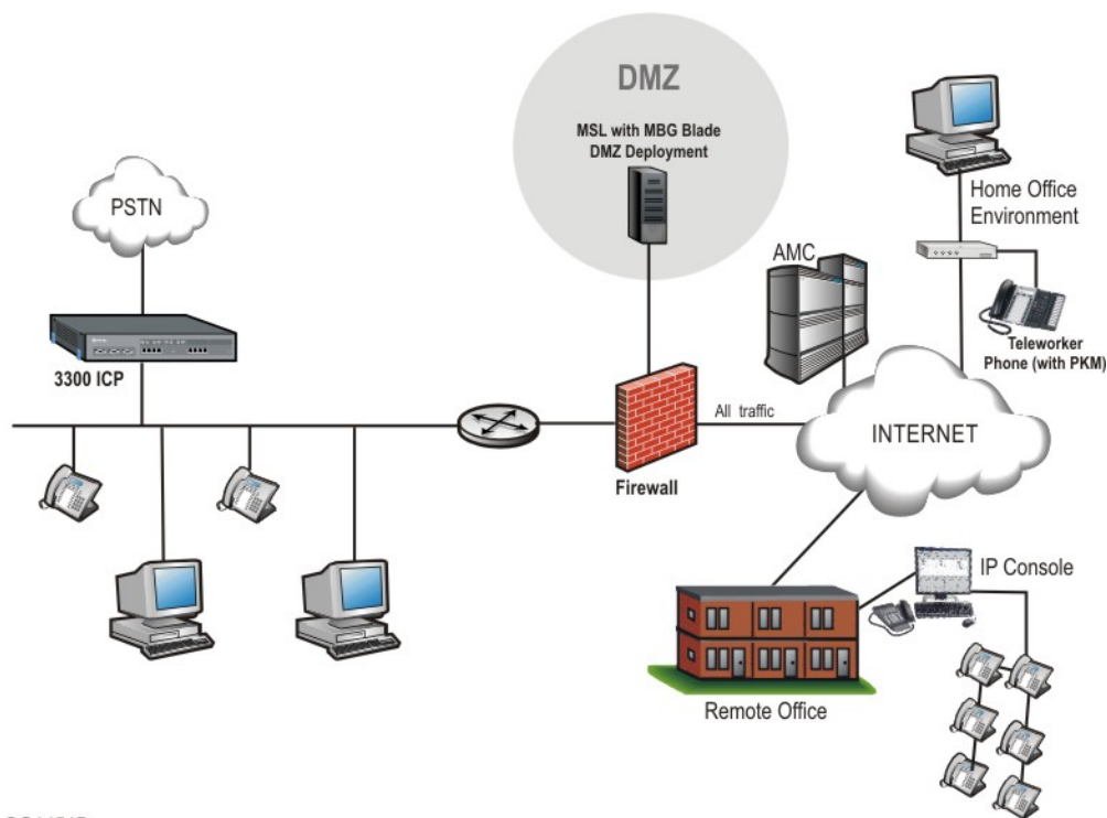
Figure 2. DMZ Configuration
