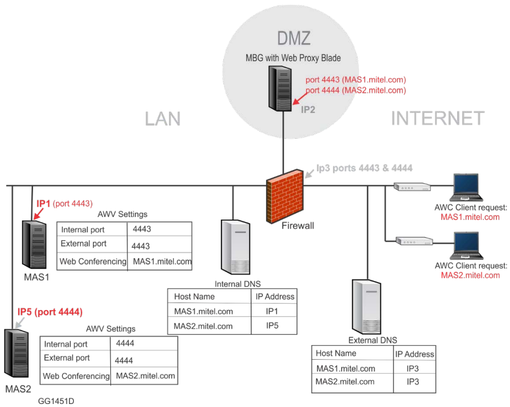
Figure 15. Multiple LAN Servers
