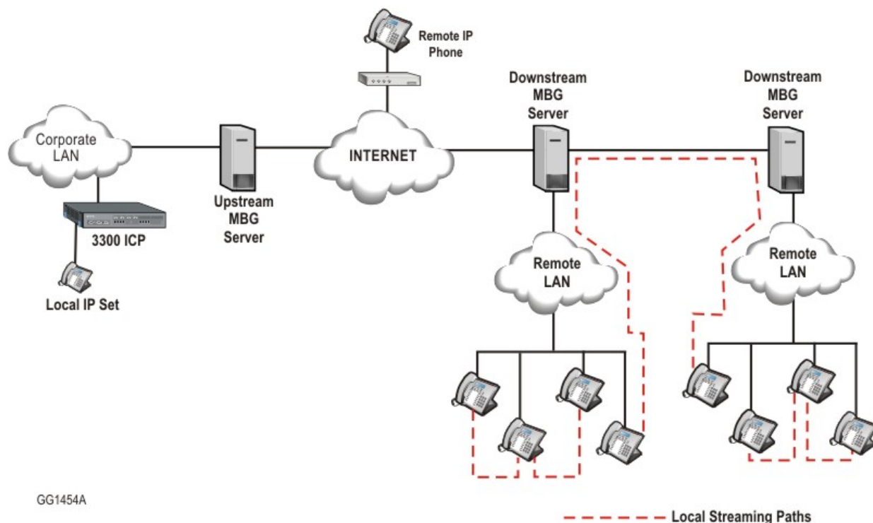
Figure 18. Daisy Chaining
