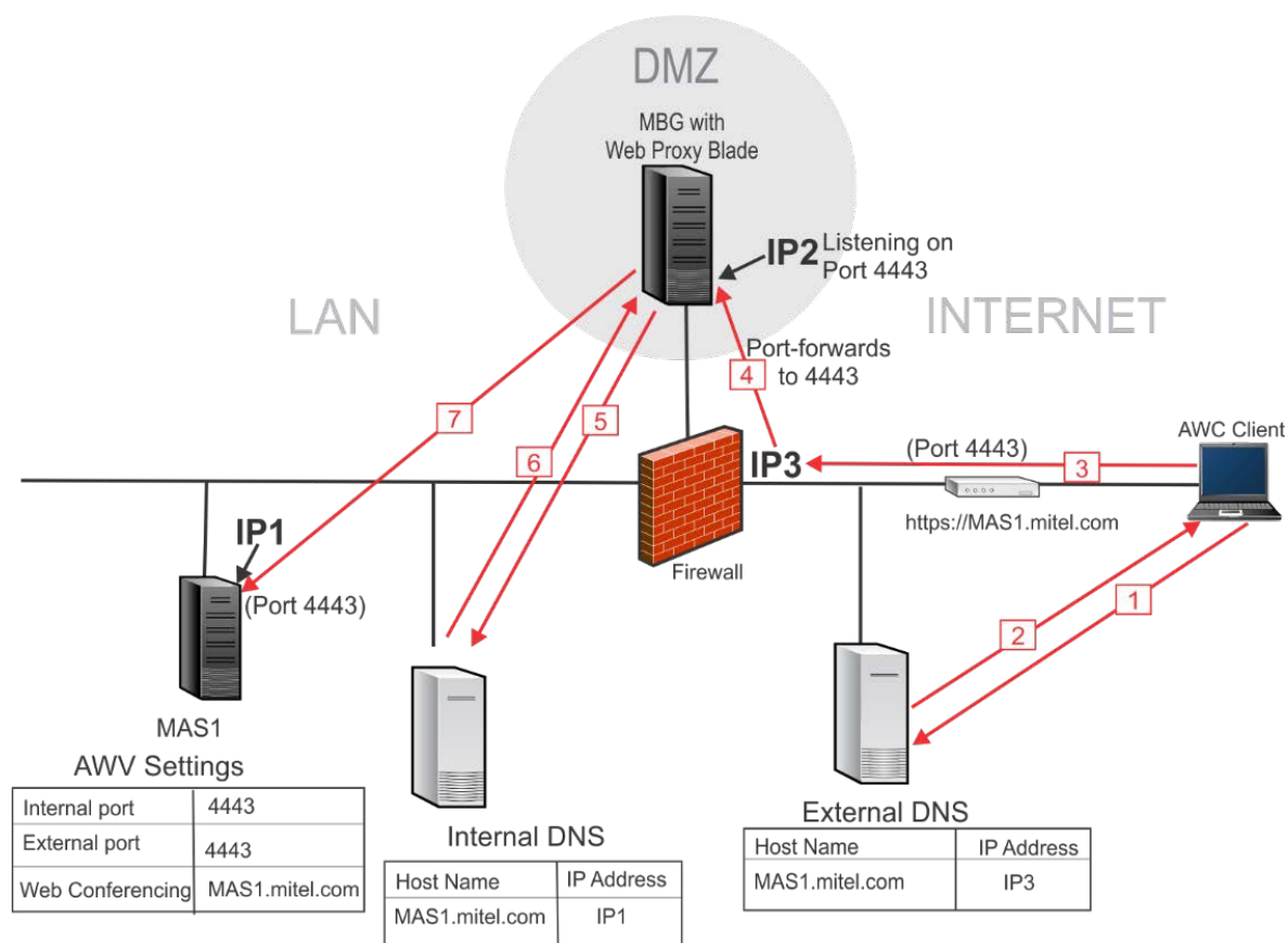
Figure 16. Message Flow for Web Conferencing Requests with One IP
