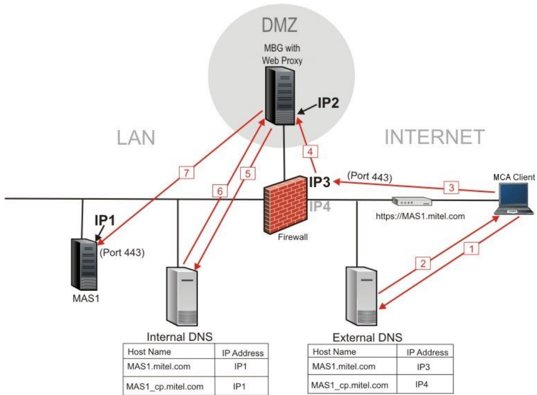
Figure 134. Message Flow for Web Traffic
