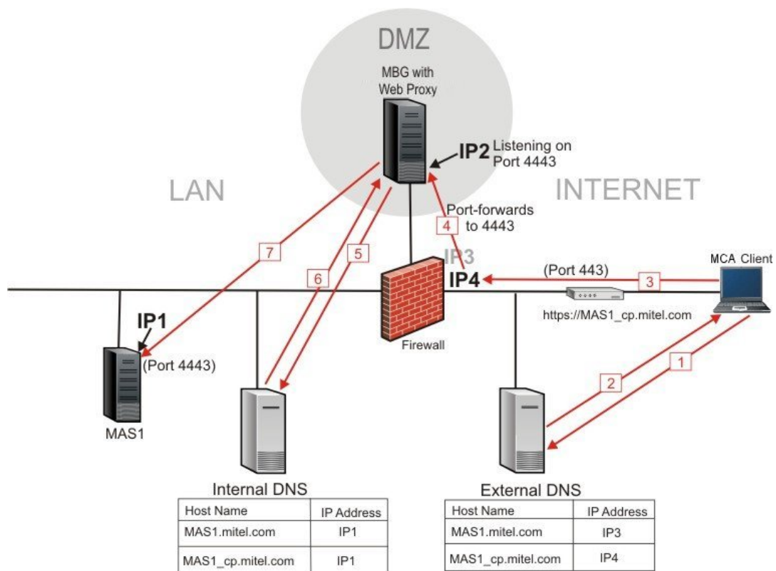
Figure 145. Message Flow for Web Conferencing Requests with Two IPs
