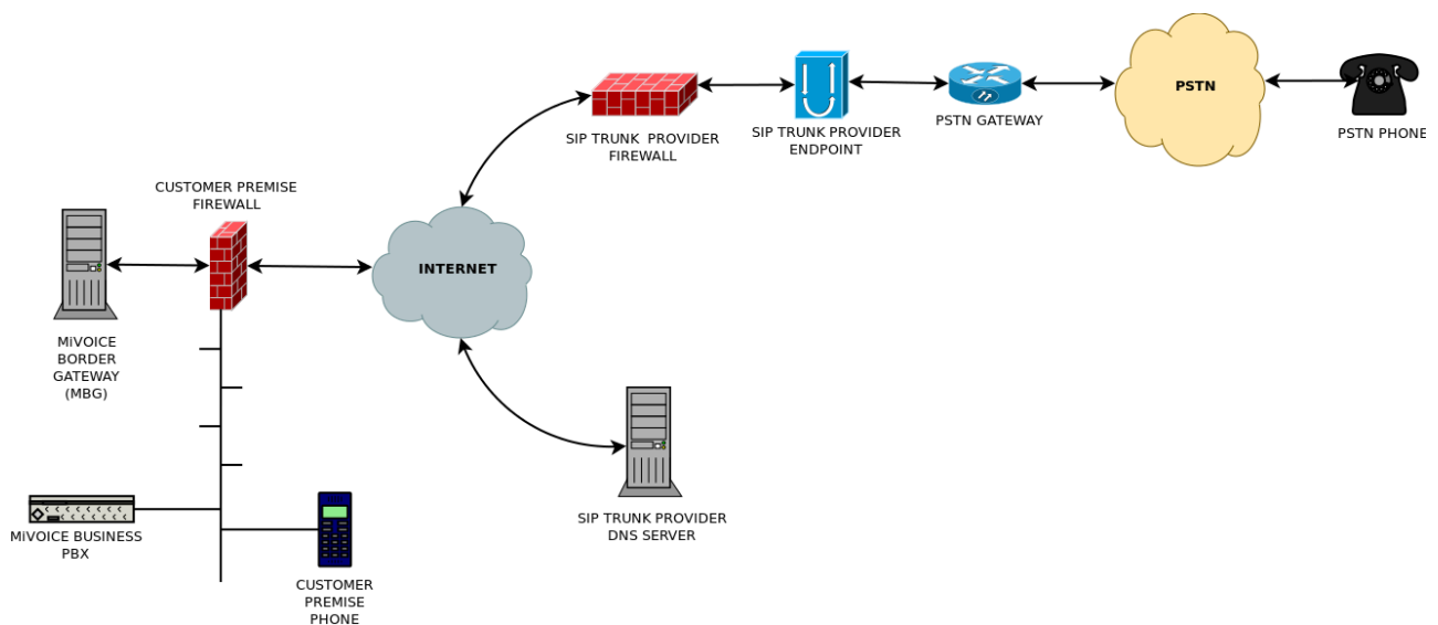
Figure 9: SIP Trunking
