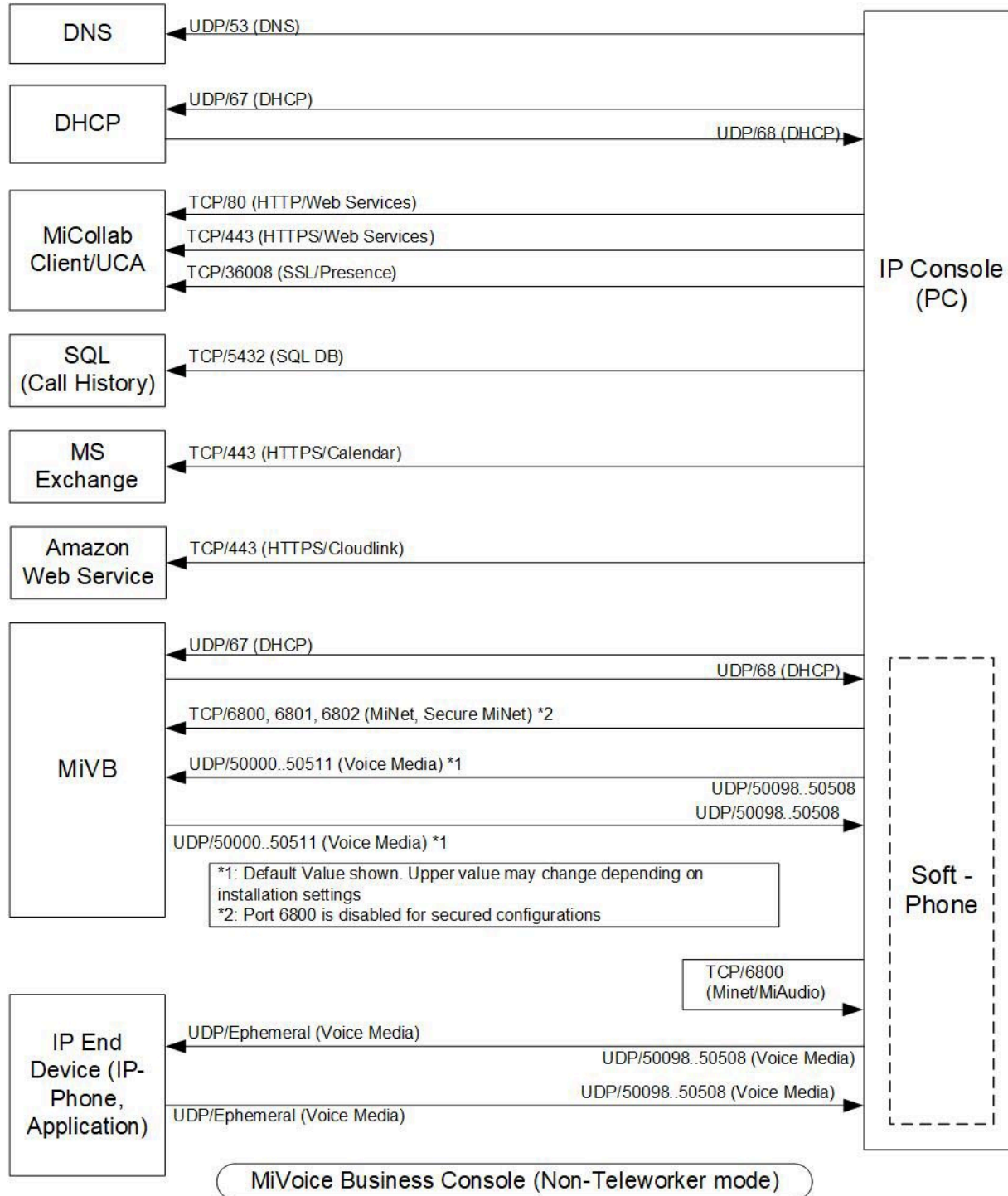
Figure 5: MiVoice Business Console - Non-Teleworker Mode
