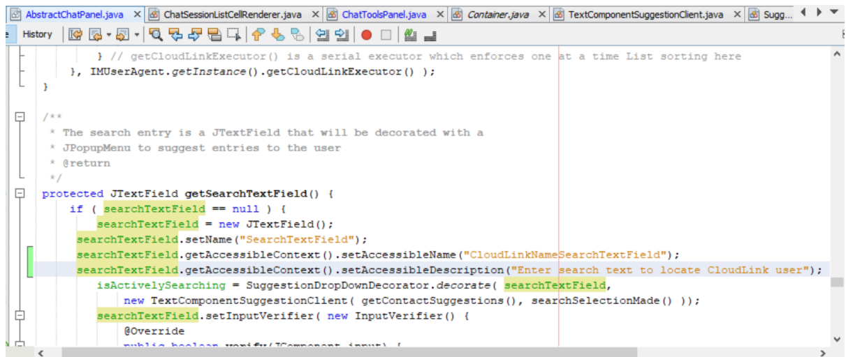
Figure 2: Adding Accessible Name and Description
