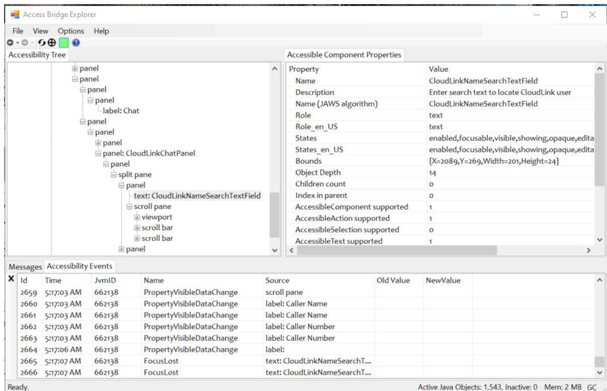
Figure 4: Accessible attributes for the Chat Search Text entry field
