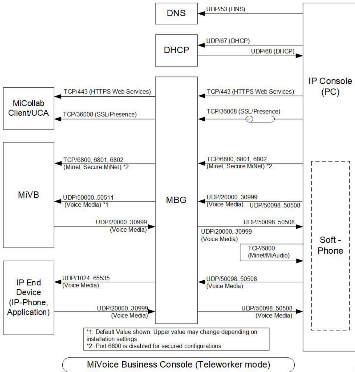
Figure 6: MiVoice Business Console - Teleworker Mode
