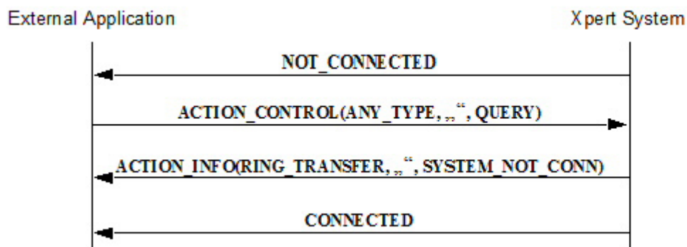
Figure 38: Disconnection in the Xpert System (OpenScape Xpert Client -> System)
