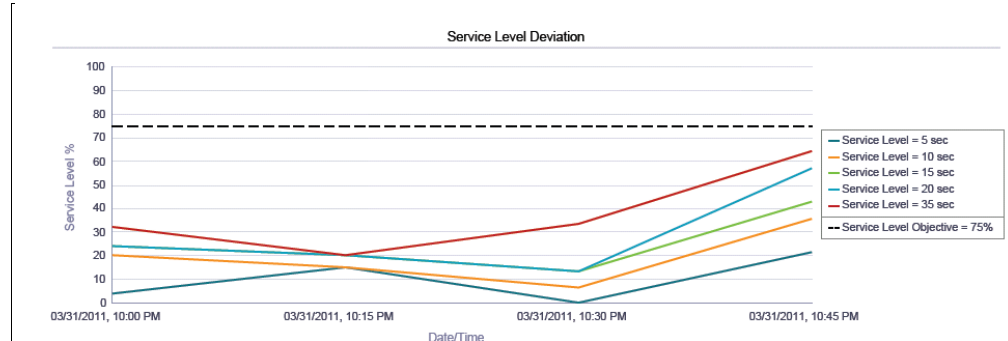
Figure 73 Service Level Report – Service Level Deviation Line Chart
