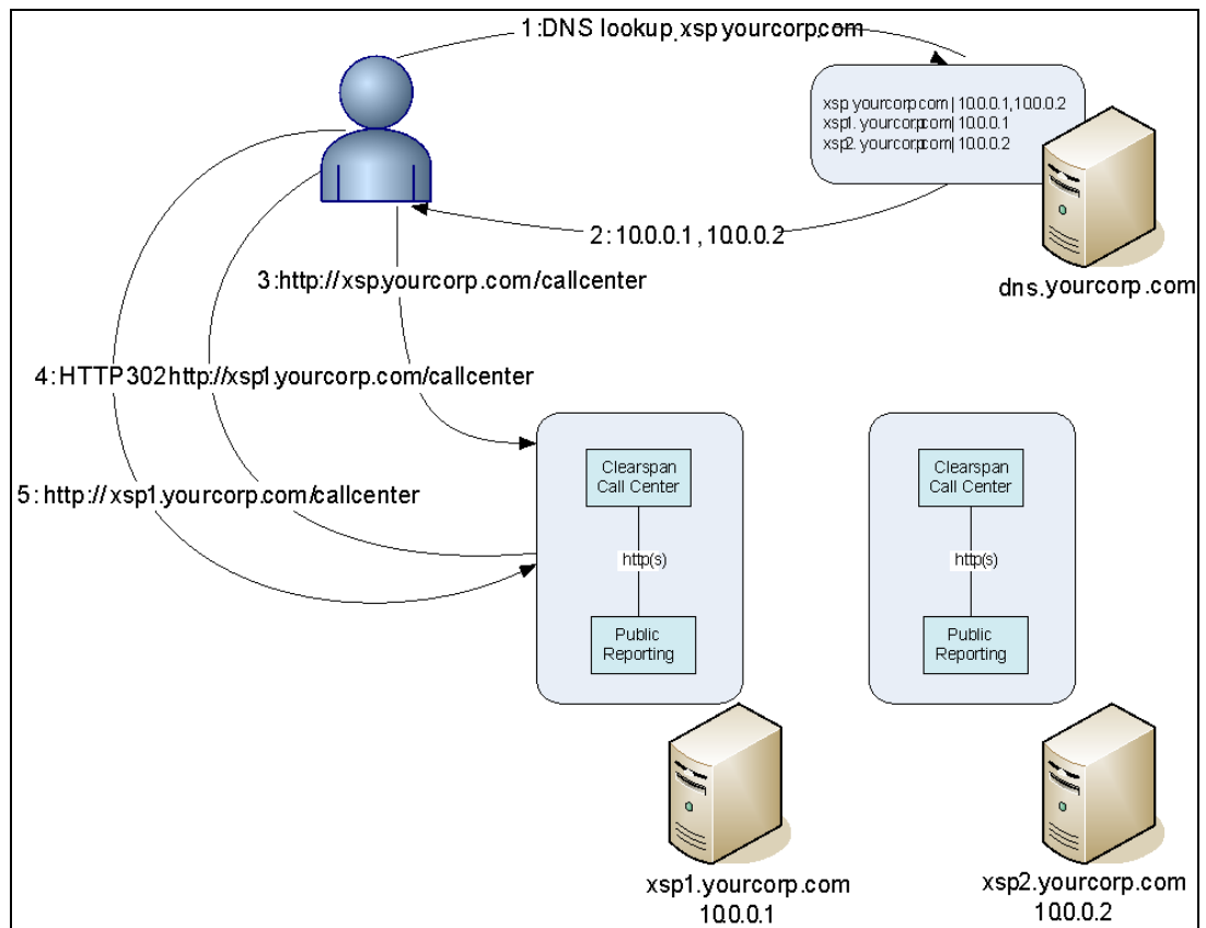
Figure 9 Redundant Configuration
