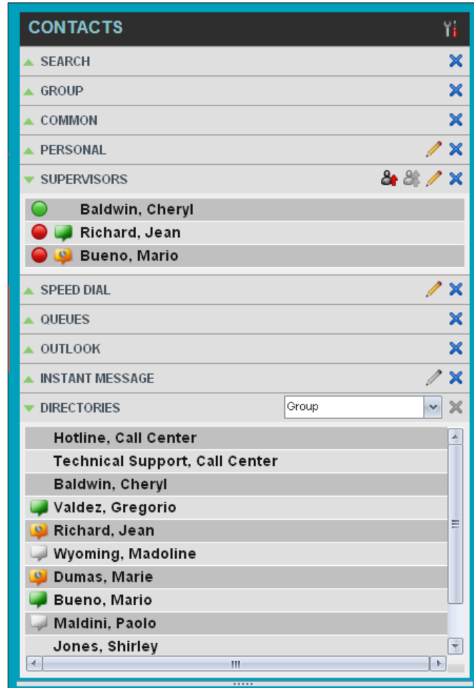
Figure 64 Contacts Pane
