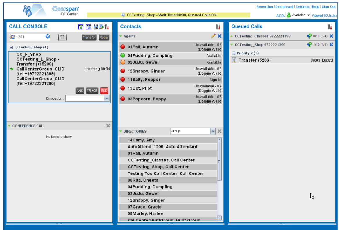
Figure 2 Call Center – Supervisor Main Interface
