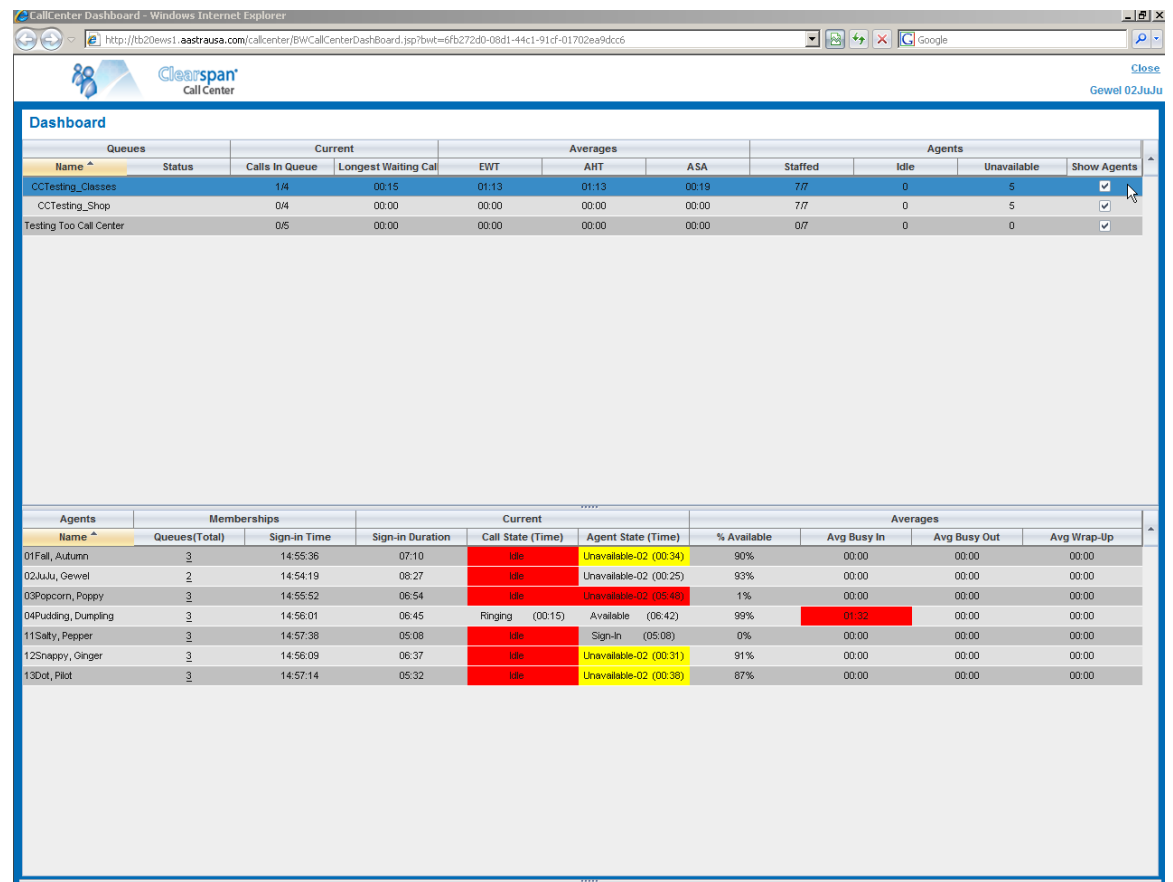
Figure 119 Dashboard
