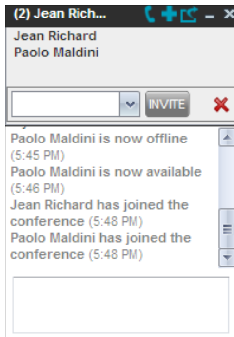
Figure 92 Multiuser Chat
