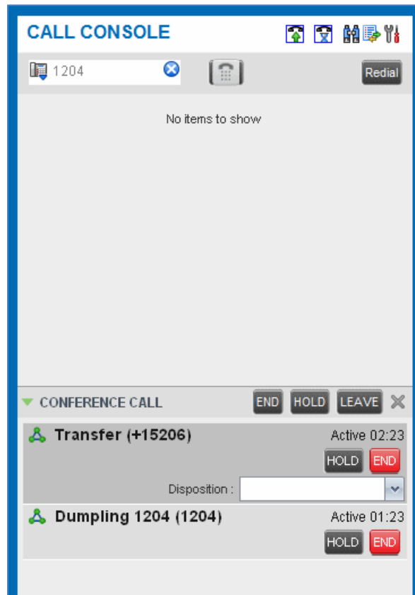
Figure 18 Call Console
