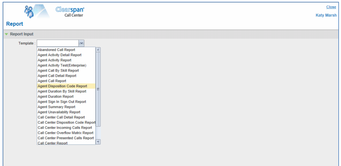
Figure 126 Report Window
