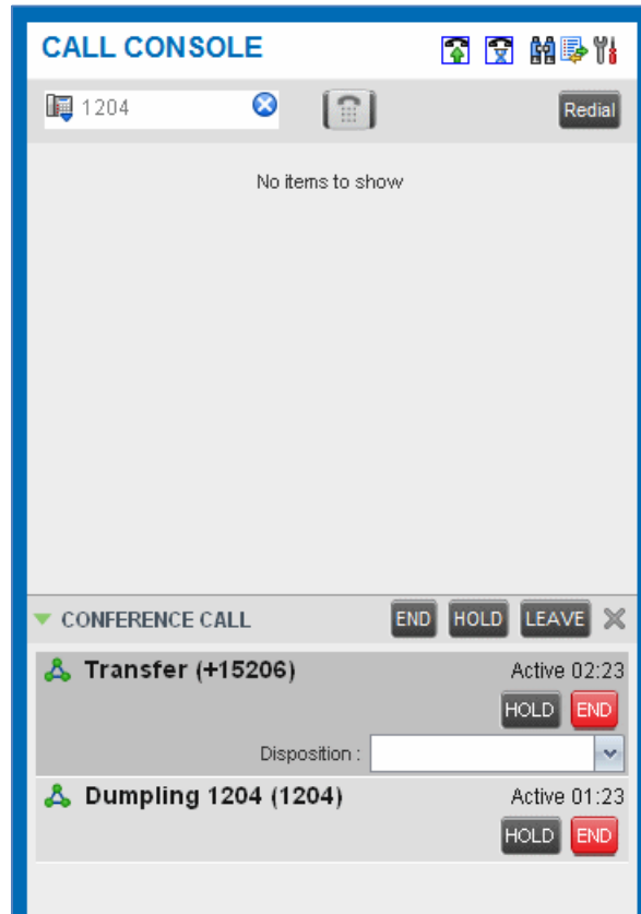
Figure 40 Call Console
