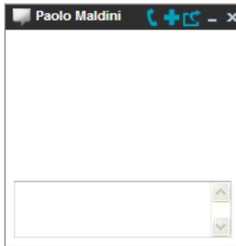
Figure 90 Chat Window
