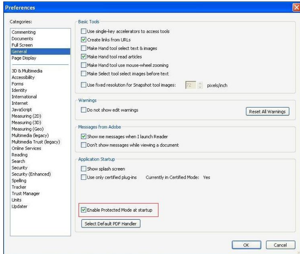
Figure 128 Preferences – General
