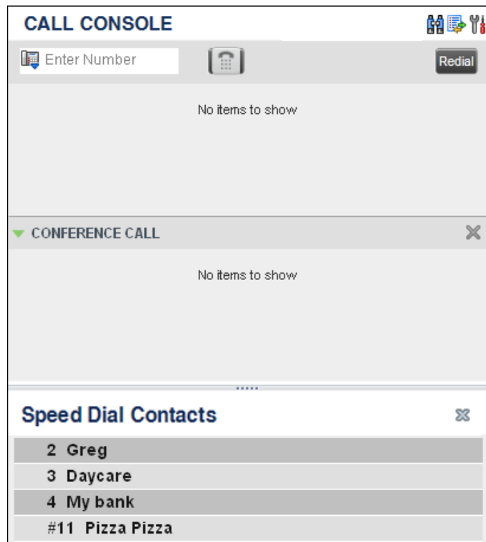
Figure 71 Custom Directory Displayed Below Call Console
