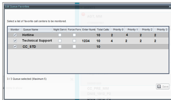
Figure 114 Edit Queue Favorites Dialog Box
