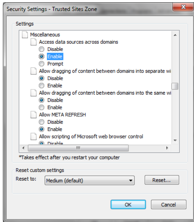
Figure 174 Internet Explorer – Security Settings – Trusted Sites Zone
