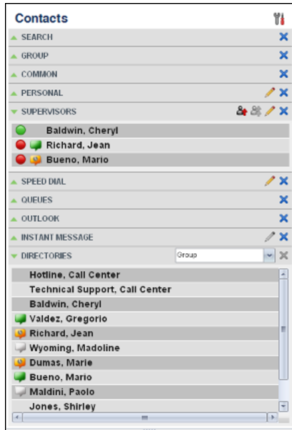
Figure 67 Contacts Pane
