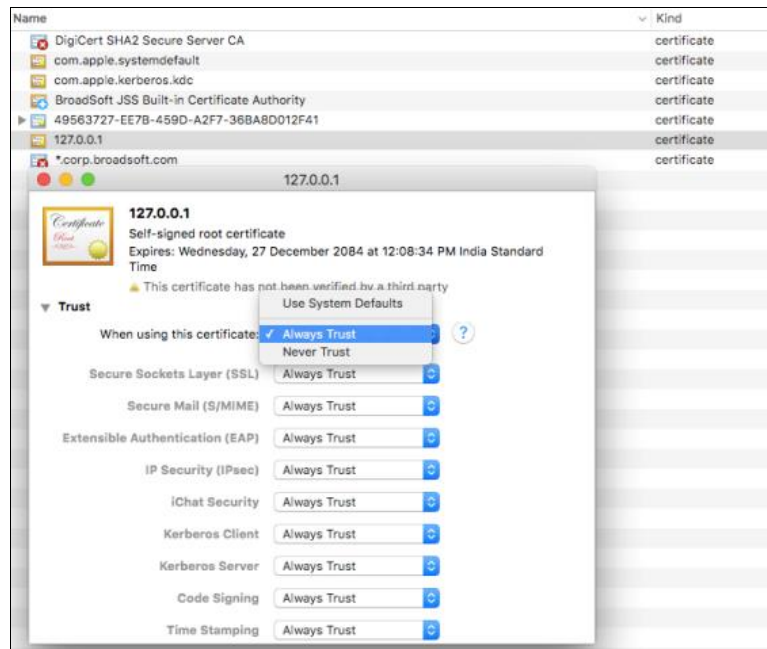
Figure 167 Certificate Window
