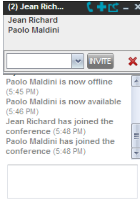
Figure 95 Multiuser Chat
