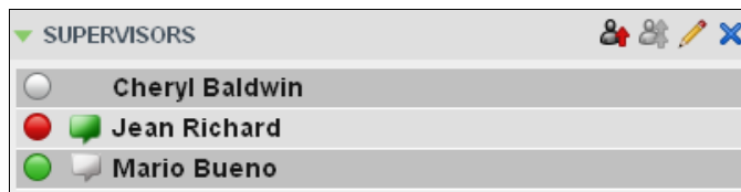
Figure 97 Supervisors Panel
