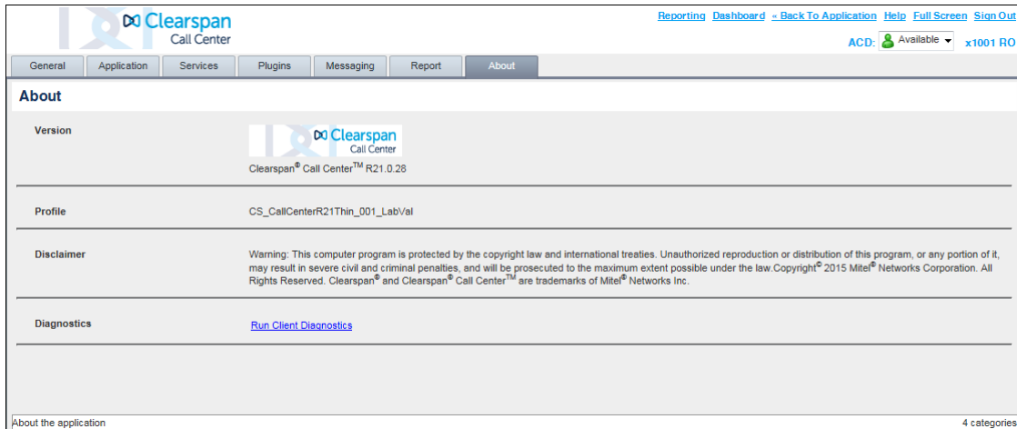
Figure 154 Settings – About
