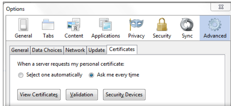
Figure 168 Firefox – Options
