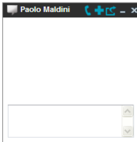
Figure 93 Chat Window
