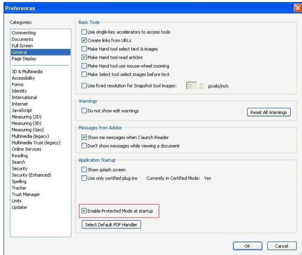
Figure 130 Preferences – General
