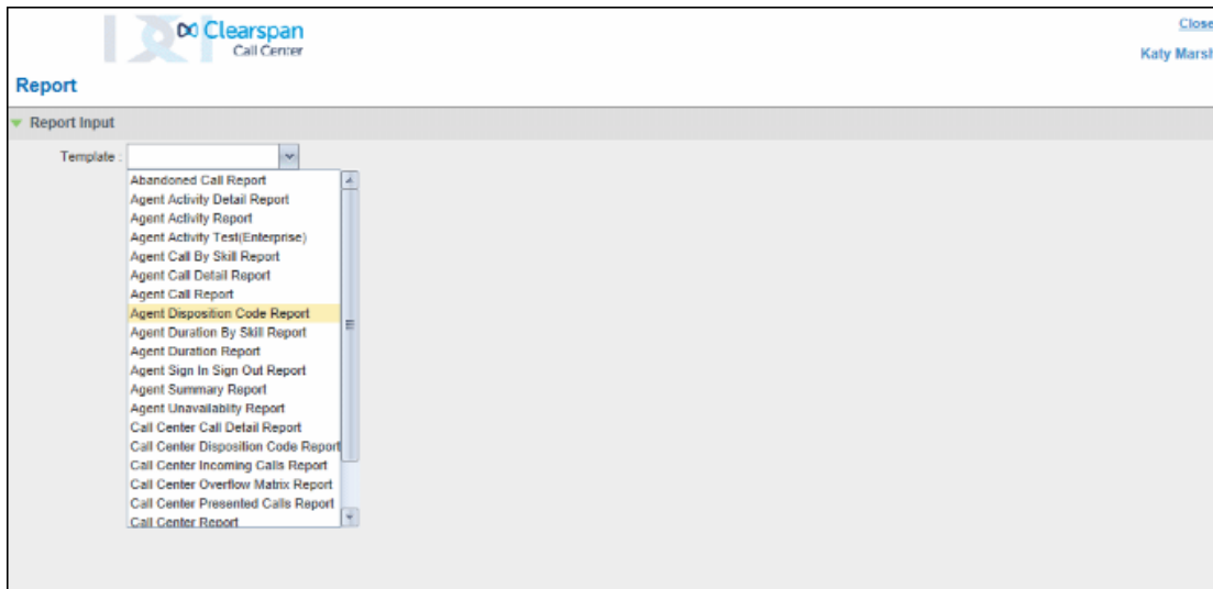
Figure 128 Report Window
