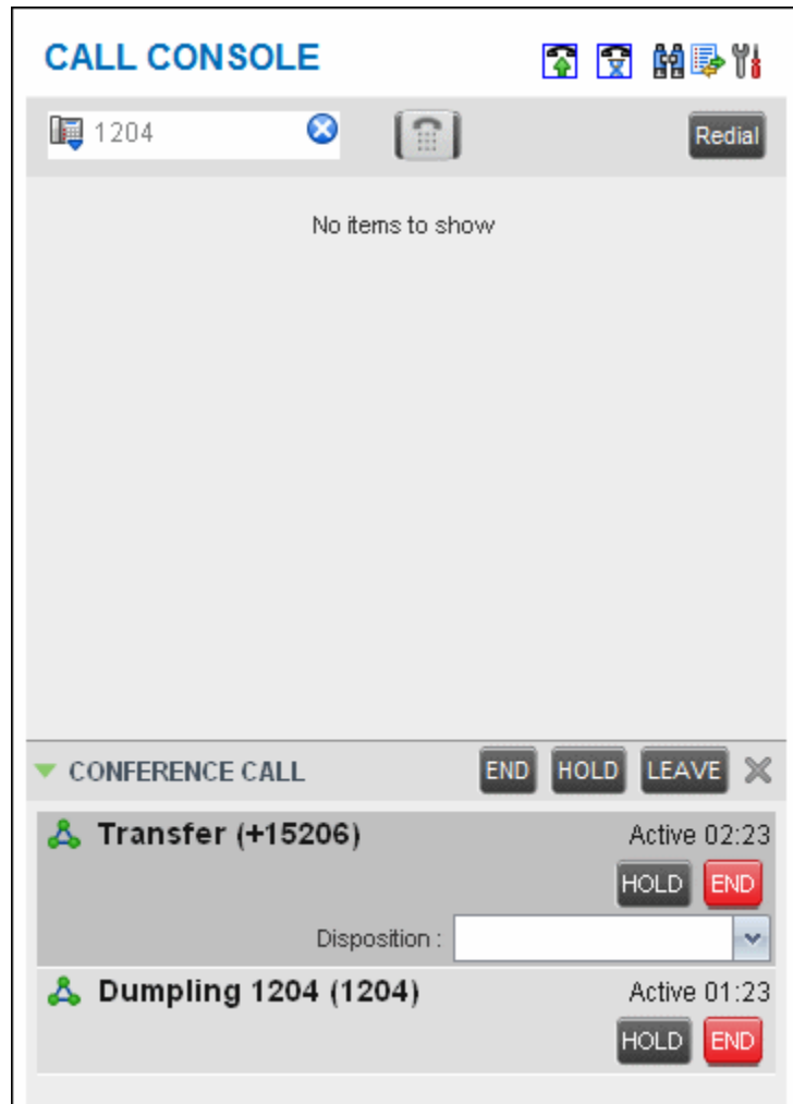
Figure 18 Call Console
