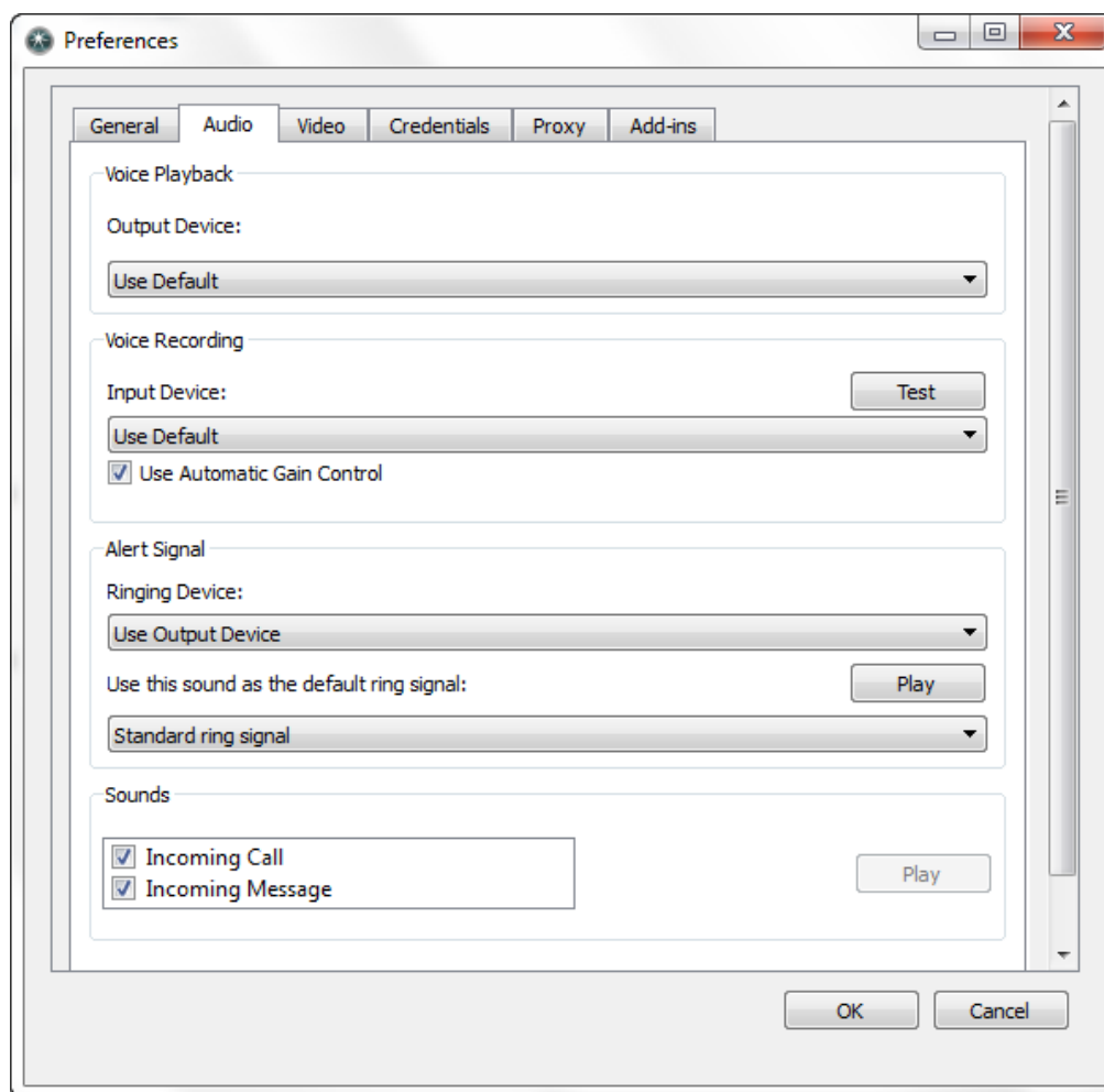
Figure 10 Preferences Window
