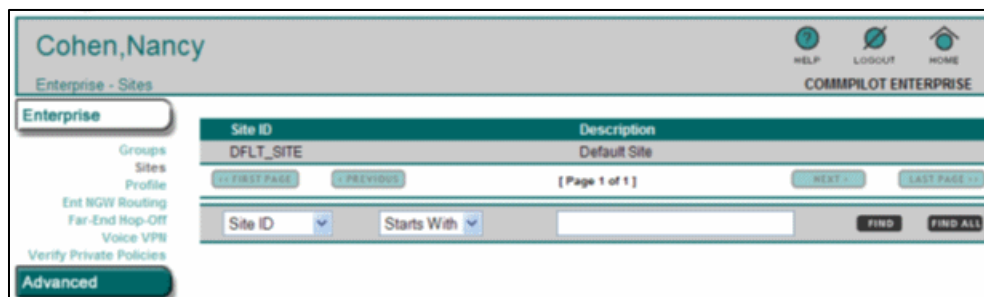
Figure 14 Enterprise – Sites
