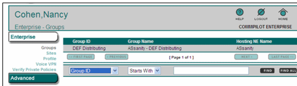
Figure 4 Enterprise – Groups
