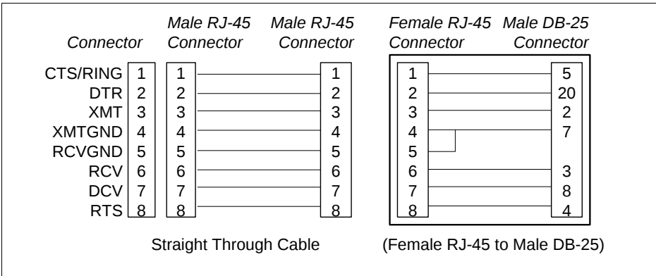
Figure 41 Connectors and Pin-out Diagram
