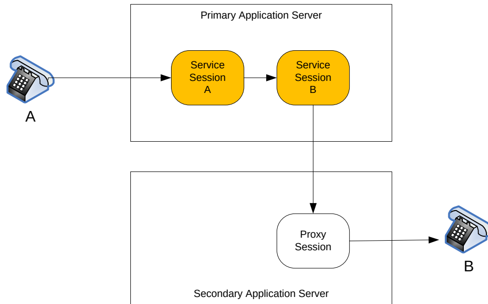
Figure 3 Call Termination Relayed by Secondary Application Server Proxy
