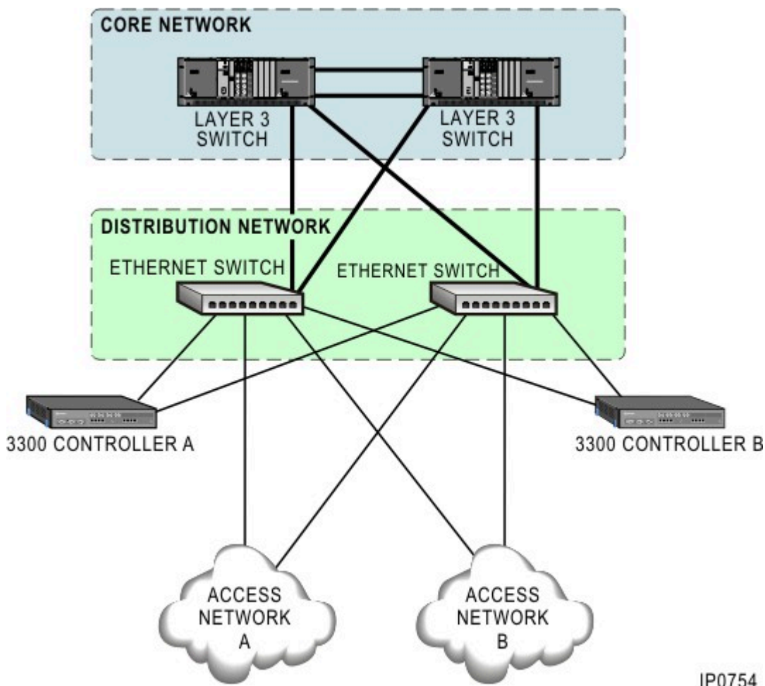
Figure 102: ICP (with STP/RSTP) to L2 Connection
