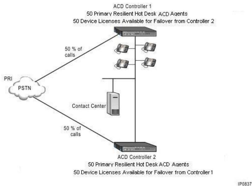
Figure 18: Basic Resiliency - Configuration 2
