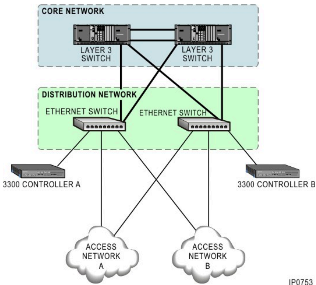
Figure 101: ICP (Without STP/RSTP) to L2 Connection
