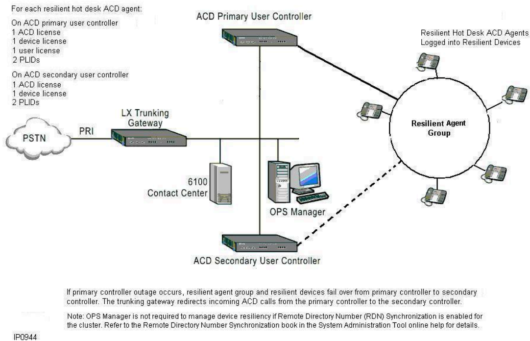
Figure 15: Resilient ACD Configuration
