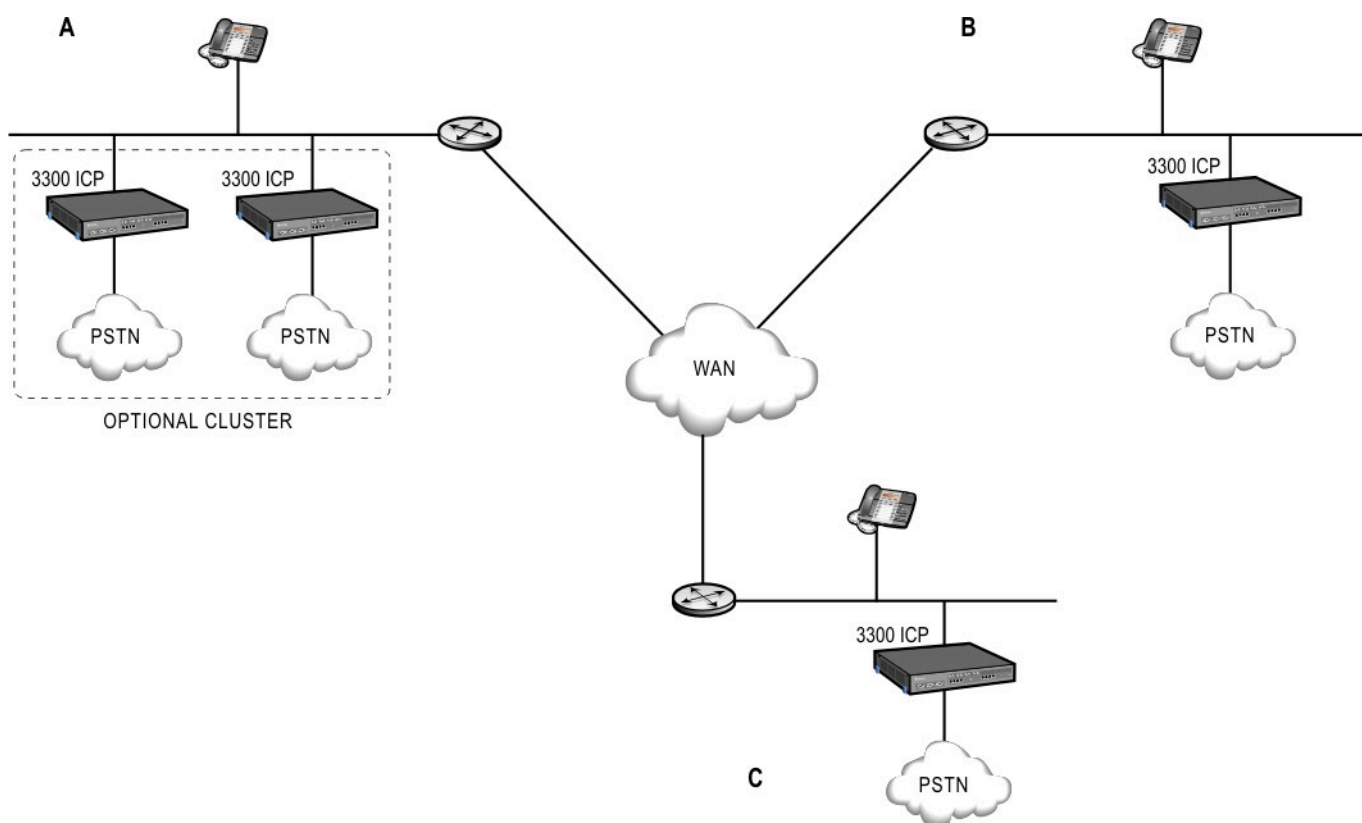
Figure 48: Scalable, Locally Dispersed Resilient Network
