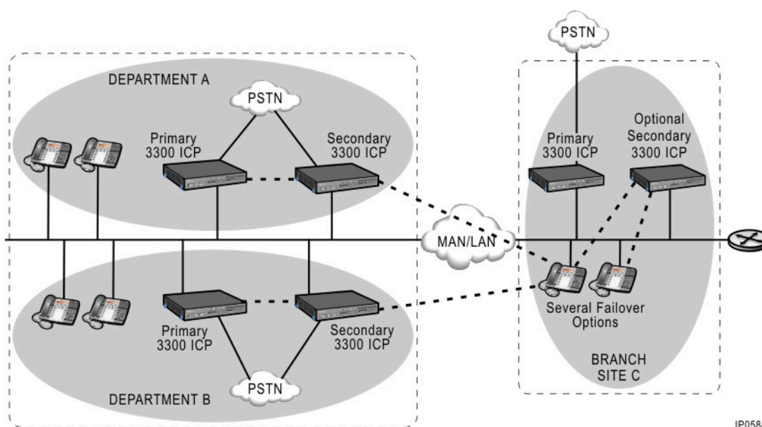
Figure 46: Resilient Hybrid Network
