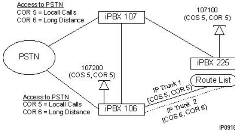
Figure 6: Dynamically Selected Service Profile (Solution)
