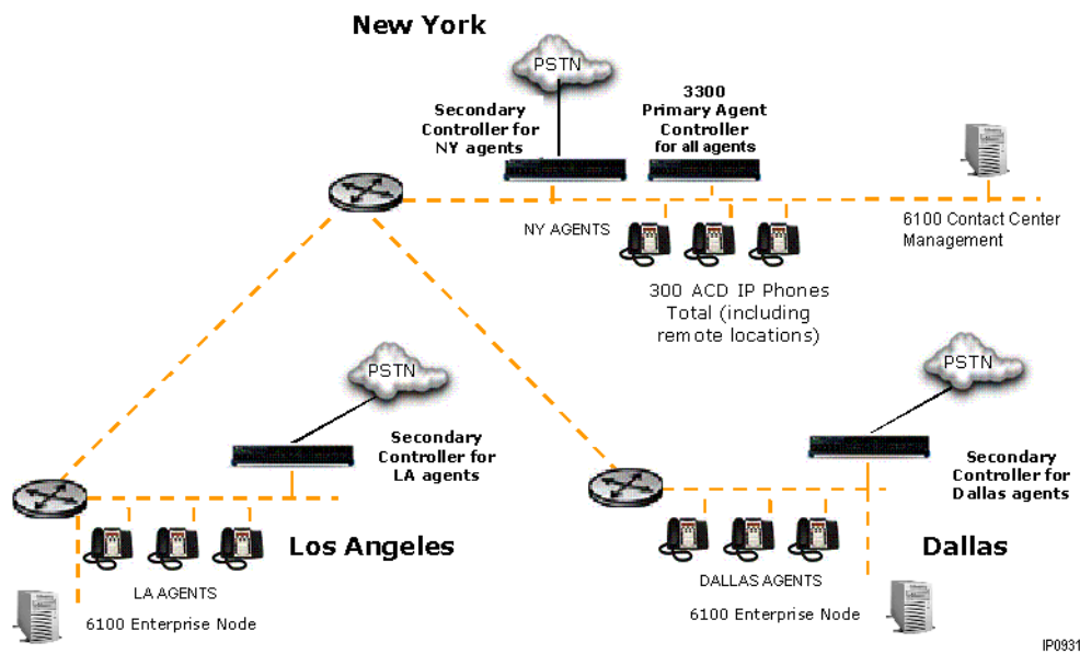
Figure 25: Resilient Virtual Contact Center - Configuration 1
