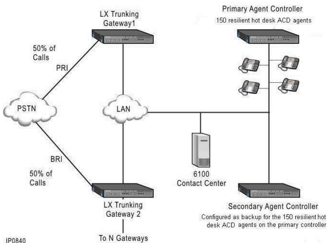
Figure 20: Full ACD Resiliency - Configuration 4
