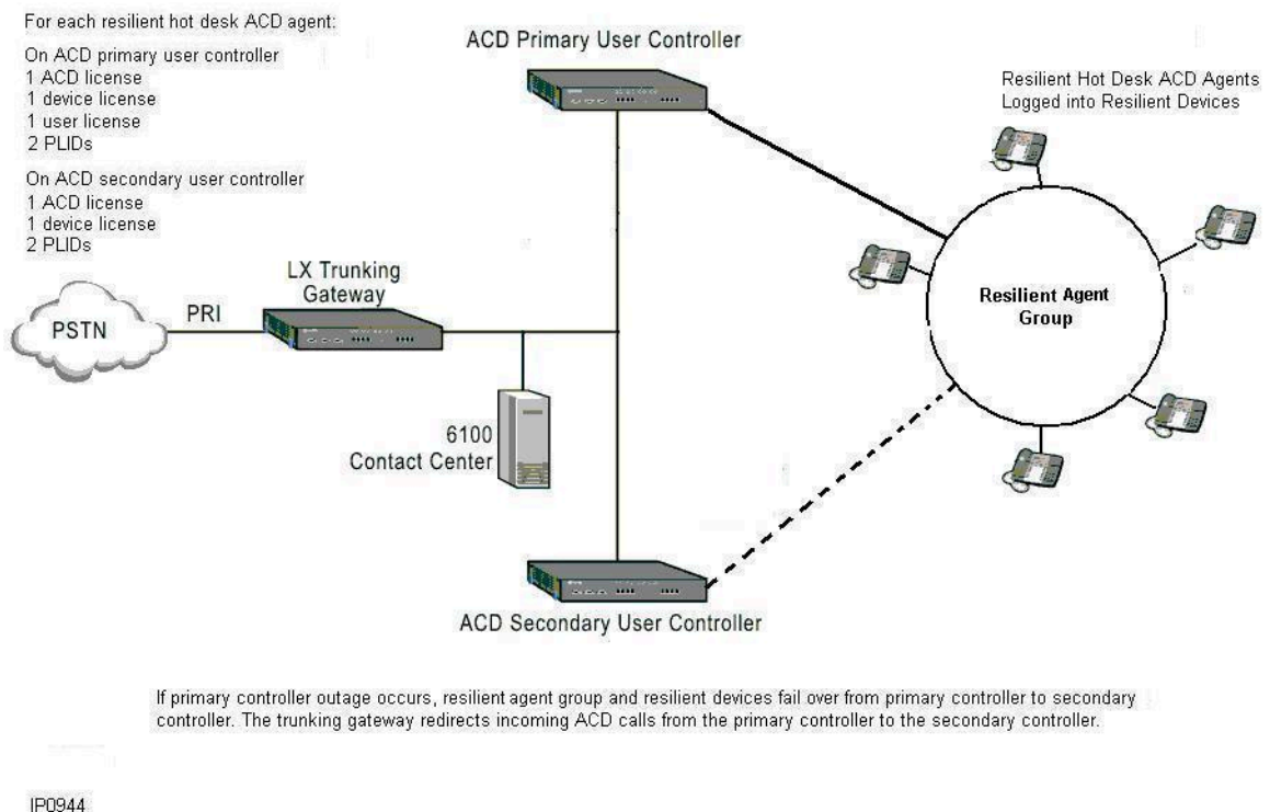
Figure 8: Resilient Hunt Group Configuration
