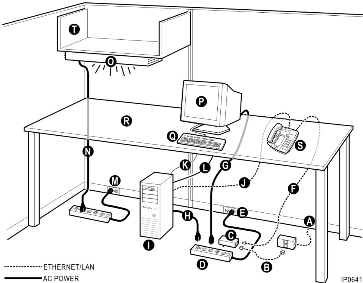
Figure 21: Desktop Cabling
