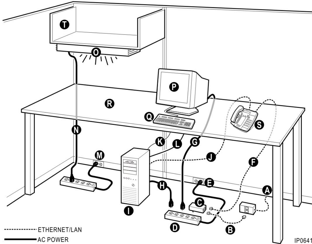
Figure 21: Desktop Cabling
