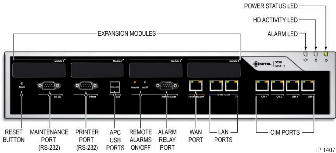
Figure 4: Mx e Controller Front View
