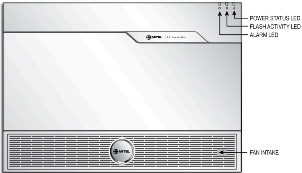
Figure 1: AX Controller
