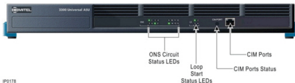
Figure 19: Universal Analog Services Unit Front Panel
