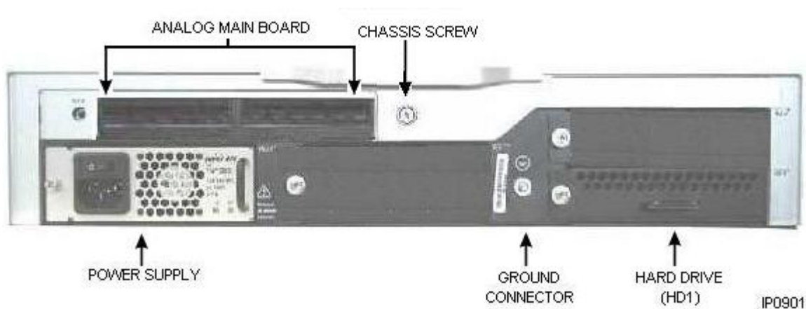
Figure 6: Mx e Controller Rear View
