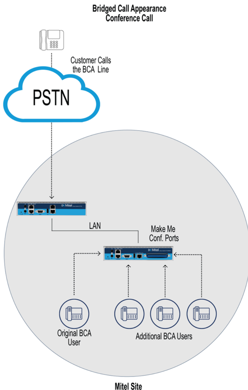
Figure 9: Bridged Call Appearance Conference Call
