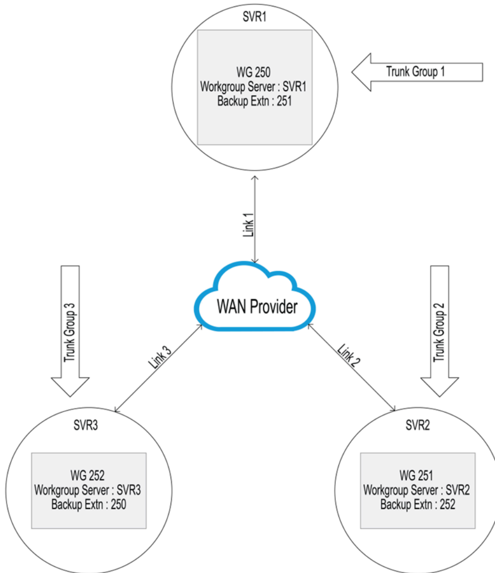
Figure 18: Lost Connectivity without a Distributed Work Group
