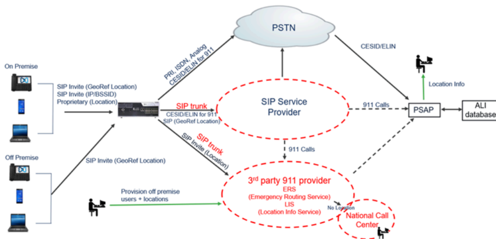
Figure 25: MiVoice Connect Deployment
