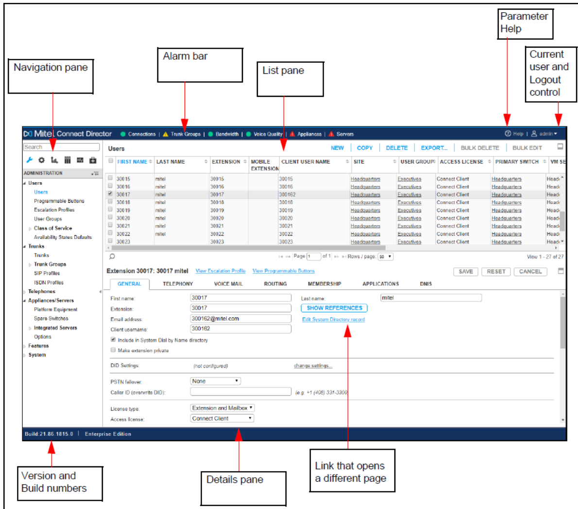
Figure 1: Connect Director Interface
