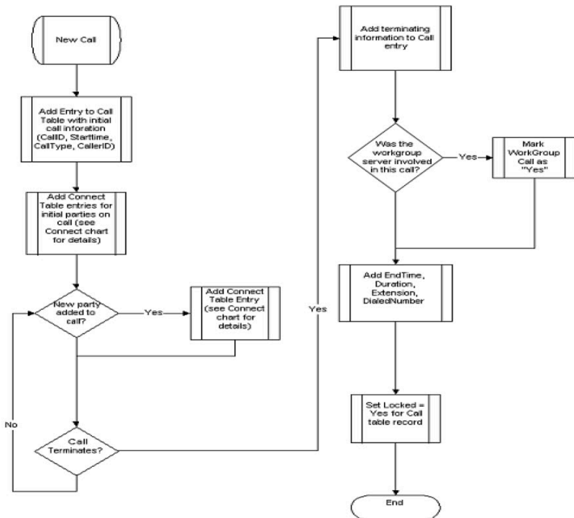
Figure 28: New Entries in the Call Table
