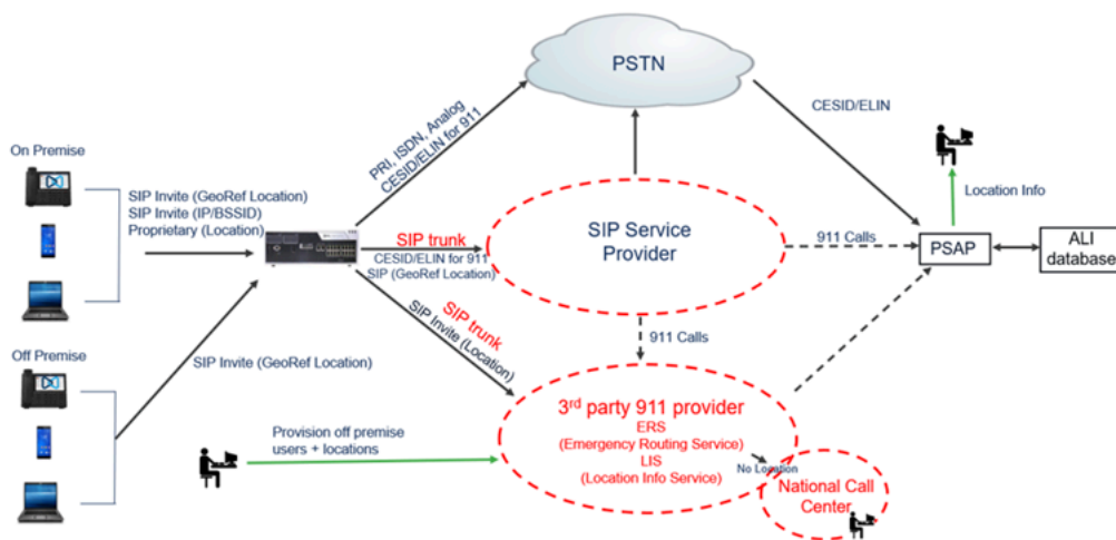
Figure 24: MiVoice Connect Deployment
