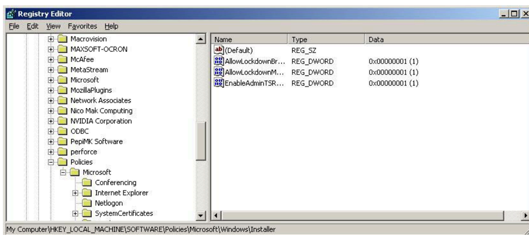
Figure 26: Registry Editor window
