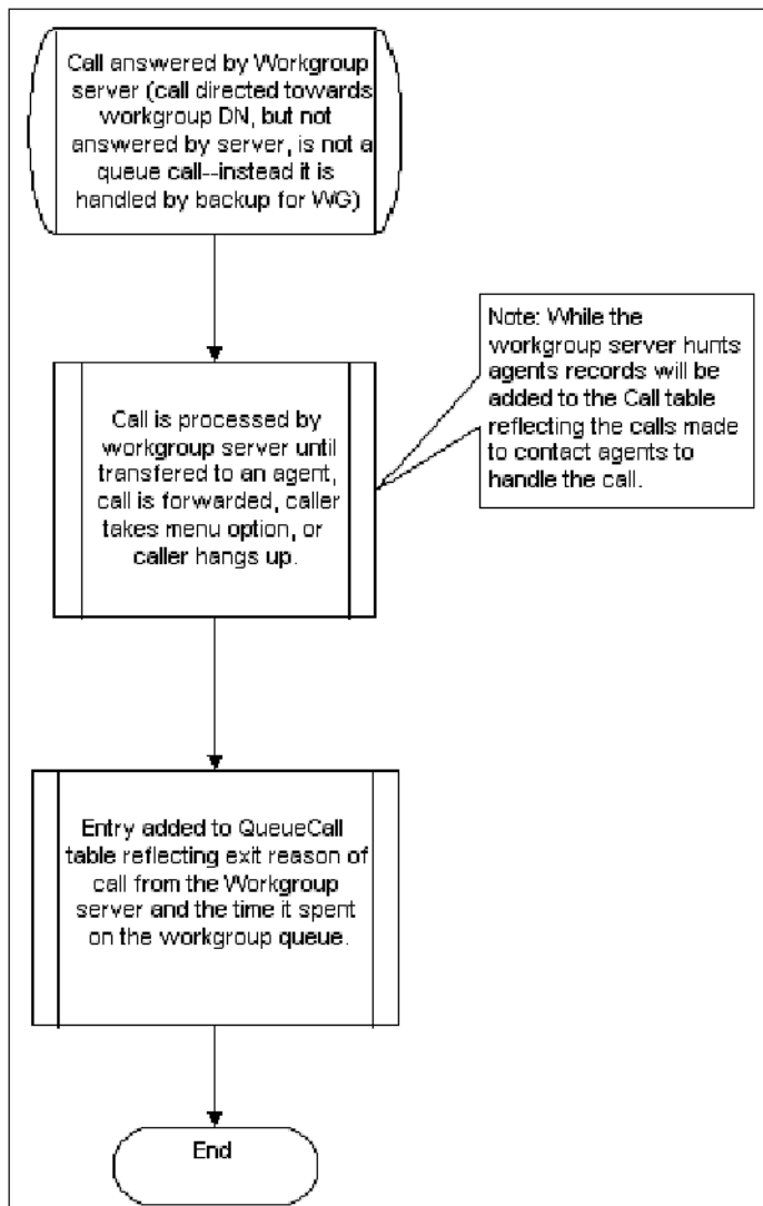
Figure 31: New Entries to the CallQueue Table
