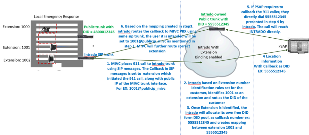
Figure 20: Intrado Extension Bind Flow
