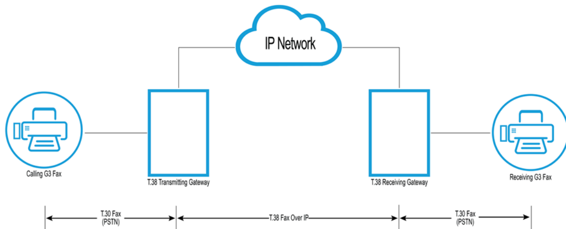
Figure 7: T.38 over IP Network Connecting to Fax Machines
