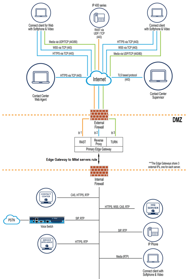
Figure 2: Network Architecture
