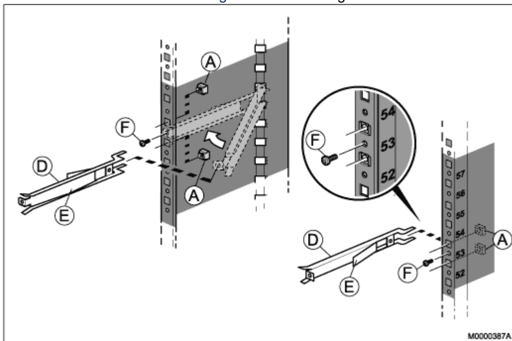
Figure 3.37: Installing Slides
