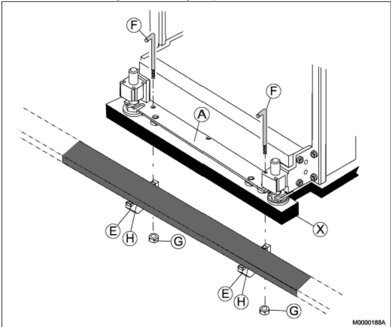
Figure 3.16: Installing the Tip Protection on a Raised Floor
