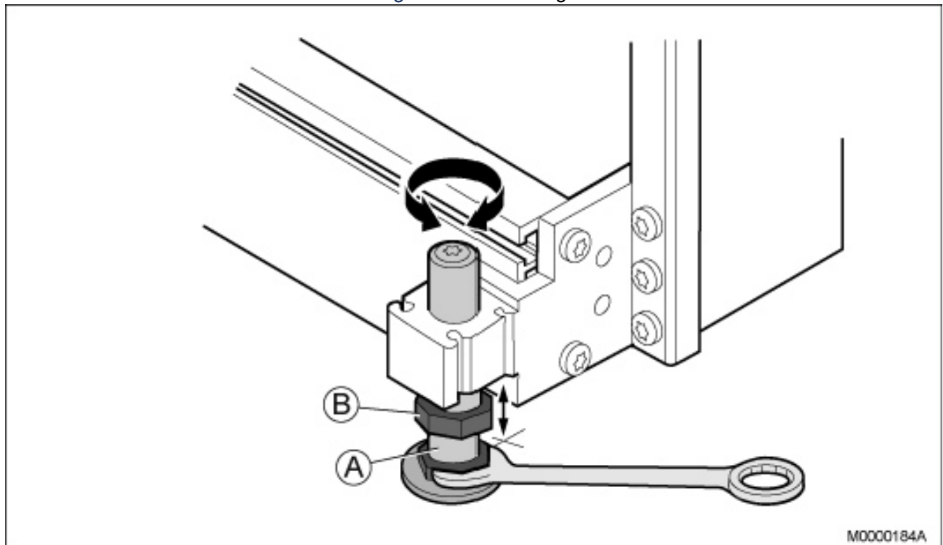
Figure 3.13: Leveling the Cabinet
