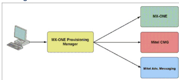
Figure 2.2: User and extension data flow in MX-ONE
