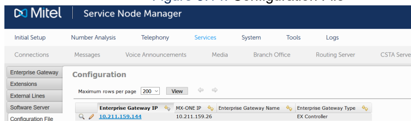
Figure 3.14: Configuration File
