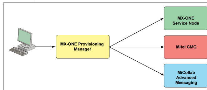
Figure 1.4: User and extension data flow in MX-ONE
