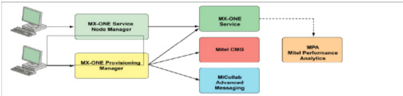
Figure 1.1: MX-ONE Manager
