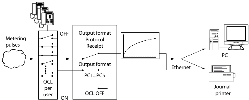
Fig. 146 Schematic sequence
