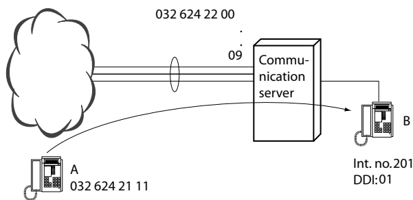
Fig. 160 Call to a free user and phone conversation
