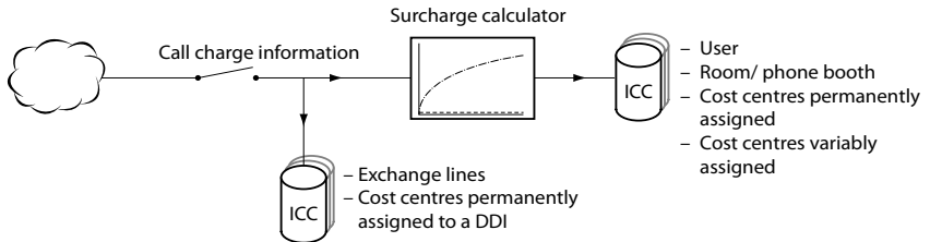
Fig. 134 Call charge allocation
