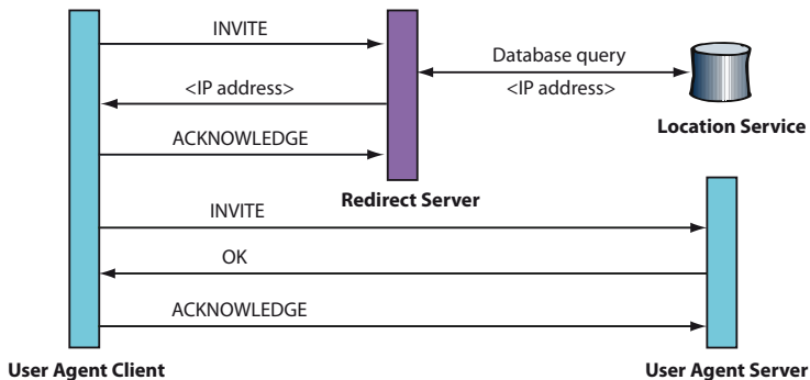
Fig. 14 Connection setup using a Redirect Server
