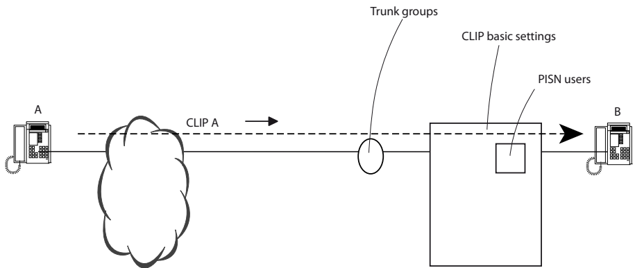
Fig. 38 CLIP incoming
