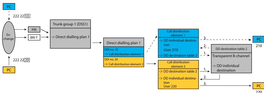
Fig. 128 Incoming data-service routing from the public network with direct dialling to a data-service individual destination
