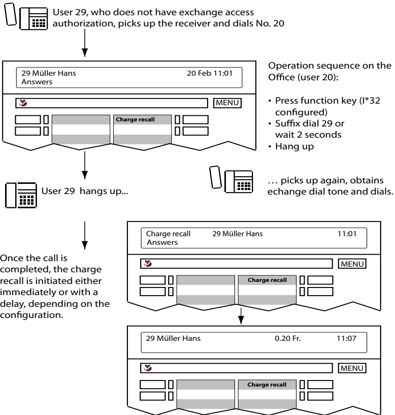
Fig. 217 Charge recall
