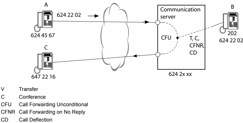
Fig. 108 Exchange-to-Exchange Connection
