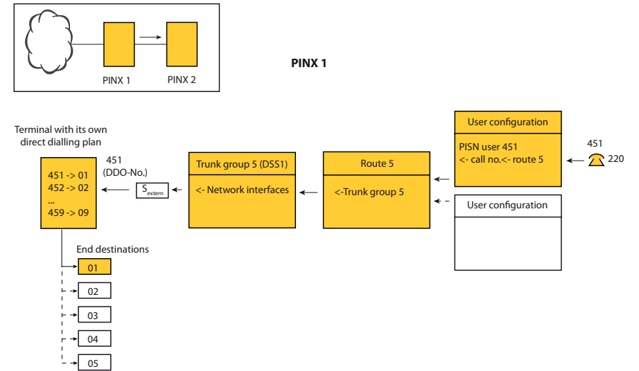
Fig. 99 Call to a terminal with its own direct dialling plan
