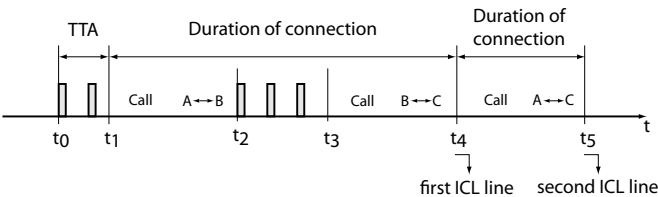
Fig. 167 Time phases for a transferred call with prior notice
