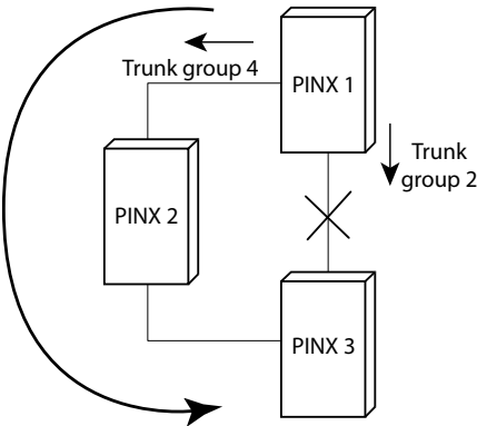
Fig. 122 Overflow routing in the private leased-line network using a sensible trunk group allocation in the route configuration
