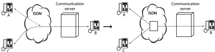
Fig. 115 Enquiry call and brokering, followed by three-party conference
