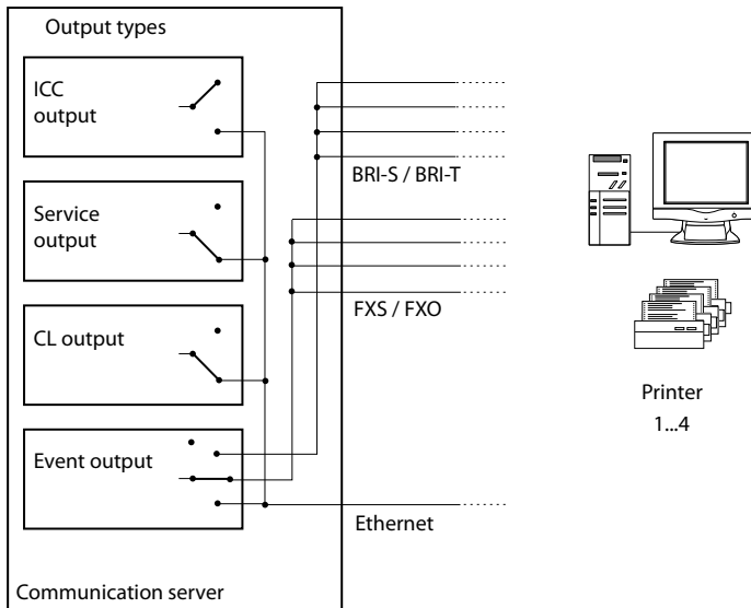
Fig. 154 Output concept
