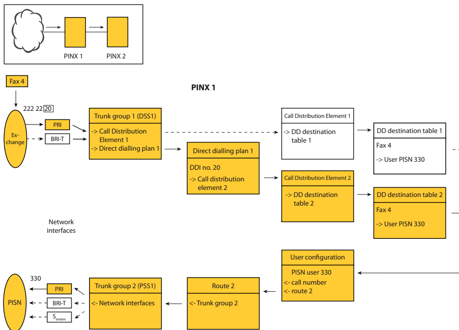
Fig. 130 Data-service routing transit from the public network with direct dialling to another PINX in the private leased-line network.
