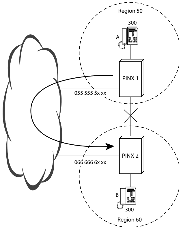
Fig. 124 Configuration example of overflow routing via the public network
