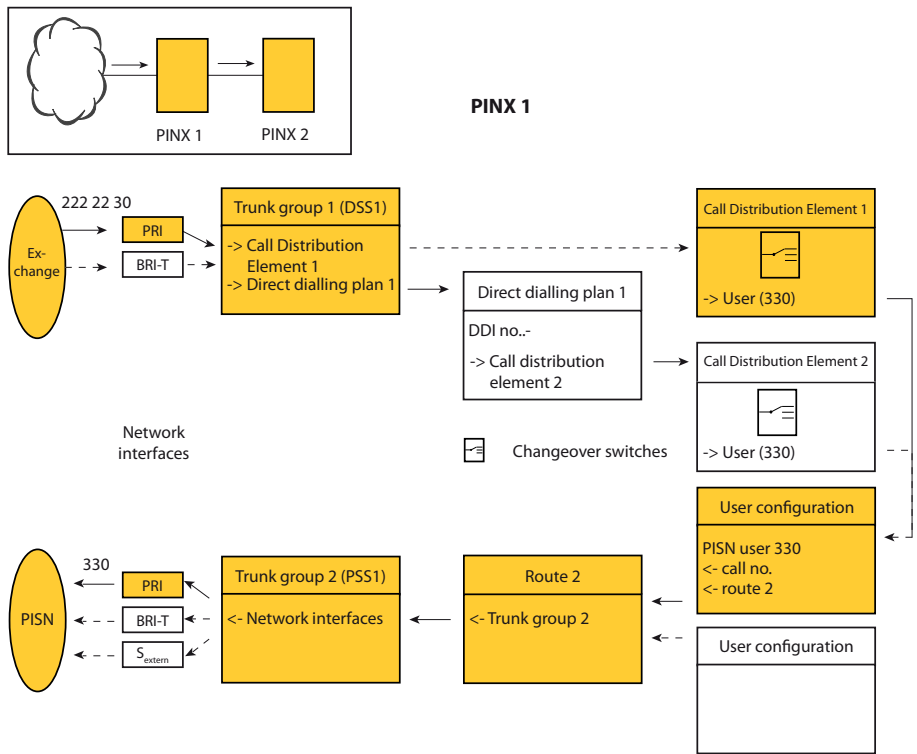
Fig. 117 Transit routing from the public network into the private leased-line network without direct dialling
