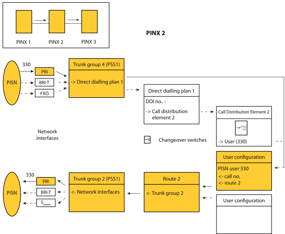
Fig. 120 Transit routing from the private leased-line network to another PISN user
