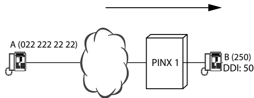
Fig. 171 User A calls user B (055 555 55 50)
