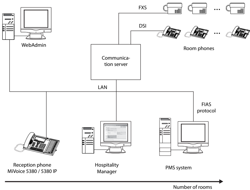
Fig. 245 Overview of configuration and operating possibilities
