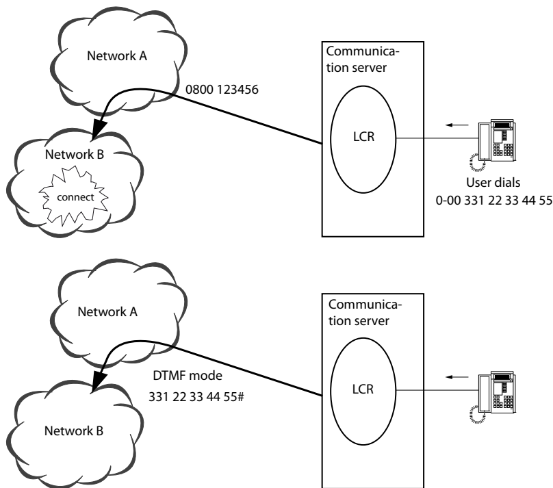
Fig. 107 Example 2: Network provider B is not integrated in the numbering plan of network provider A
