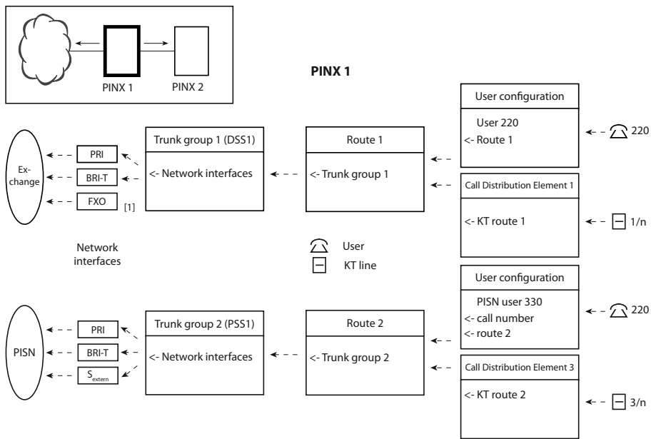
Fig. 90 Routing outgoing calls
