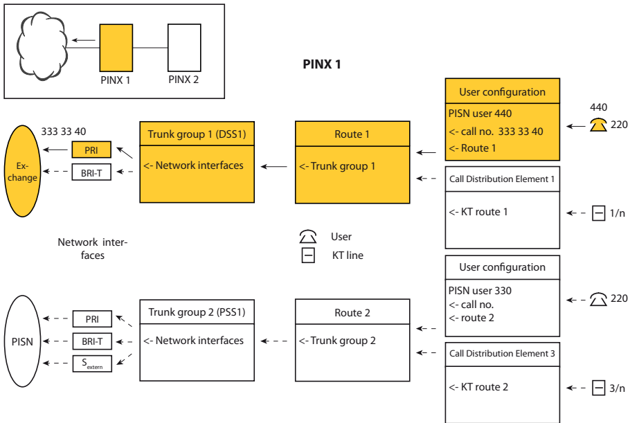
Fig. 95 Routing a call to a virtual network PISN user via the public network
