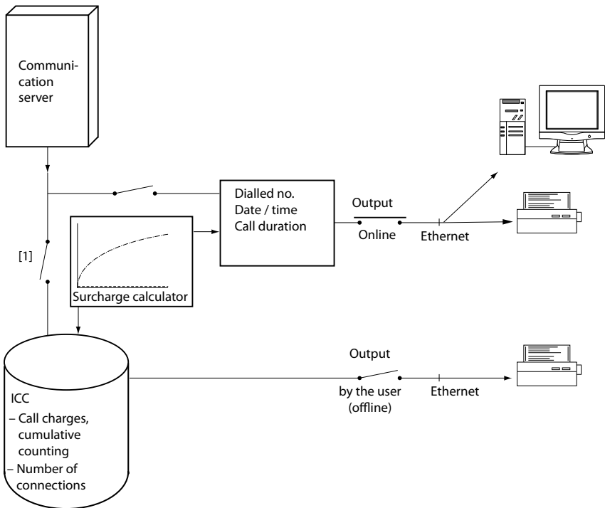
Fig. 132 Call logging and charge acquisition for outgoing traffic
