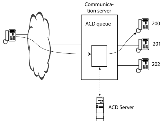
Fig. 79 Communication server call routing controlled by the ACD server
