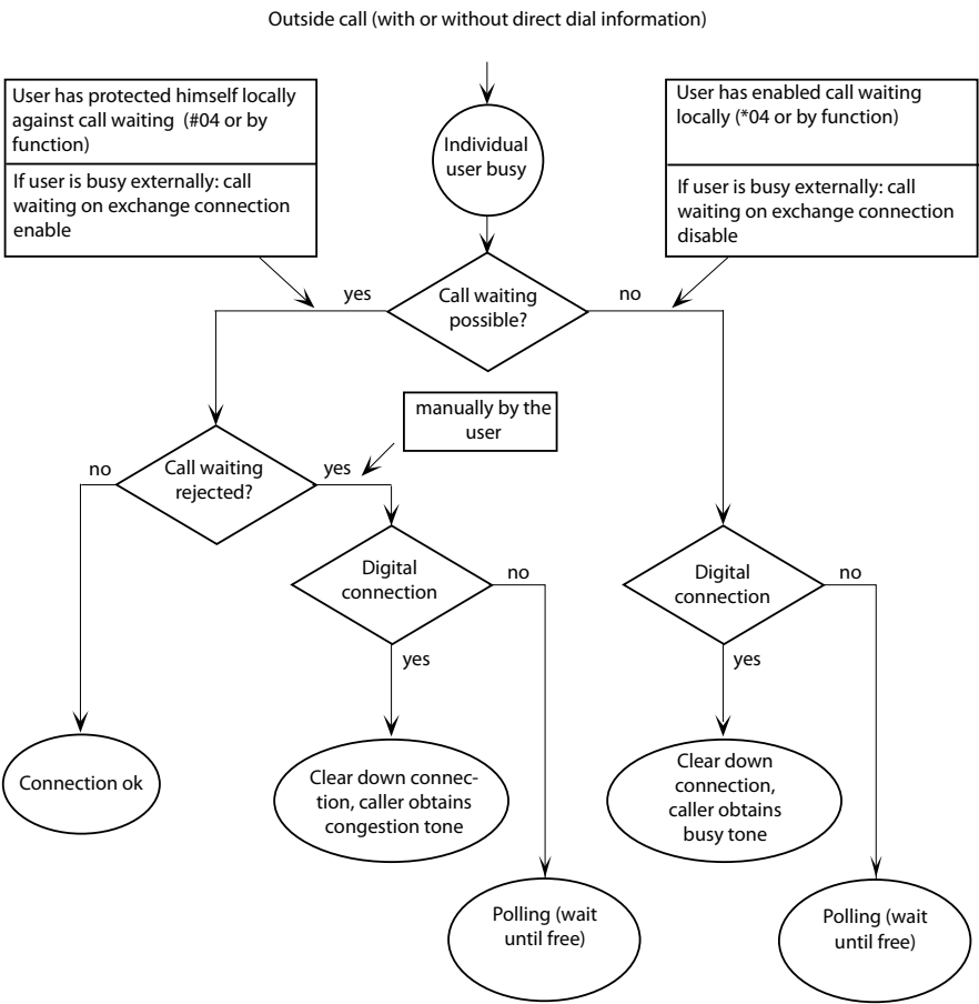
Fig. 88 Call distribution if user is busy
