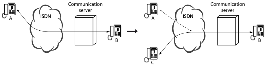
Fig. 113 External connection followed by hold and enquiry calls
