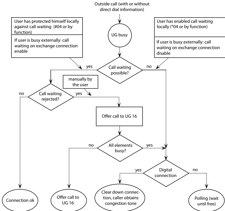
Fig. 89 Call distribution if user group busy
