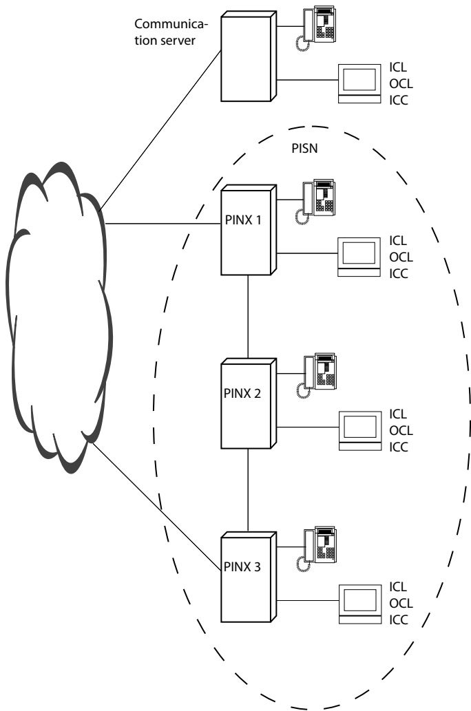
Fig. 133 Call logging in the PISN
