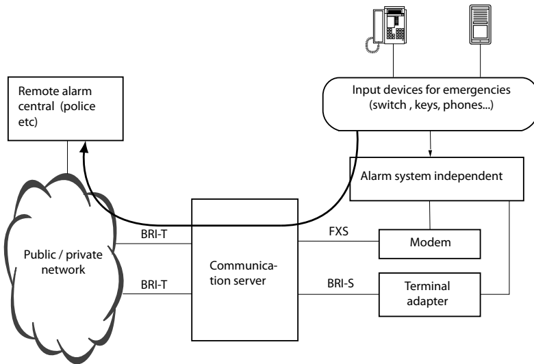
Fig. 97 Overview of a configuration for emergency applications
