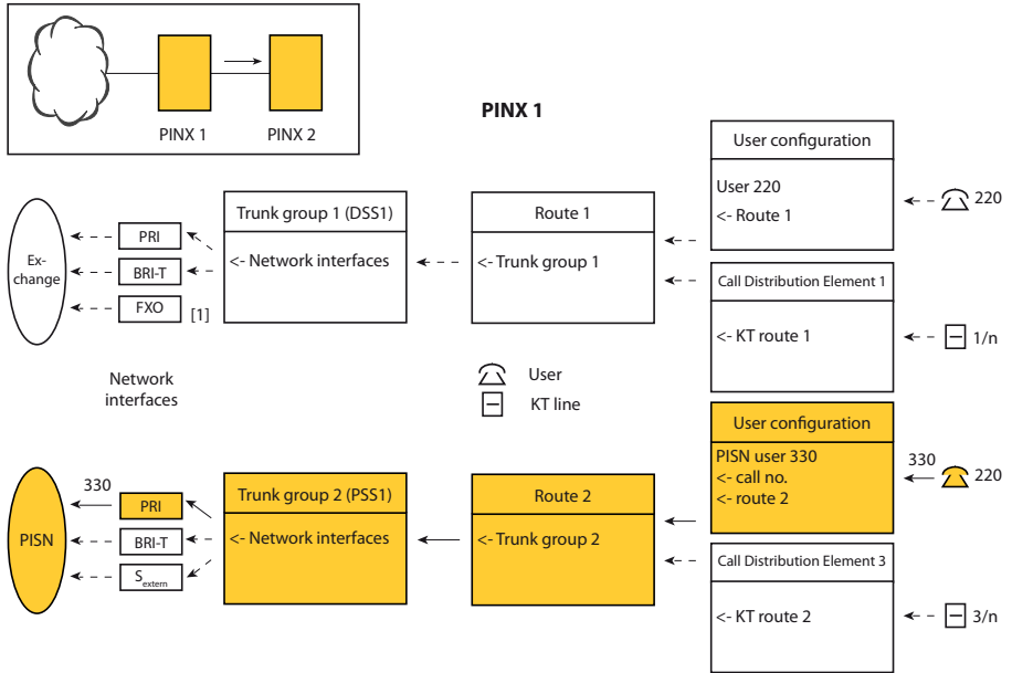
Fig. 98 Routing a call to the private leased-line network
