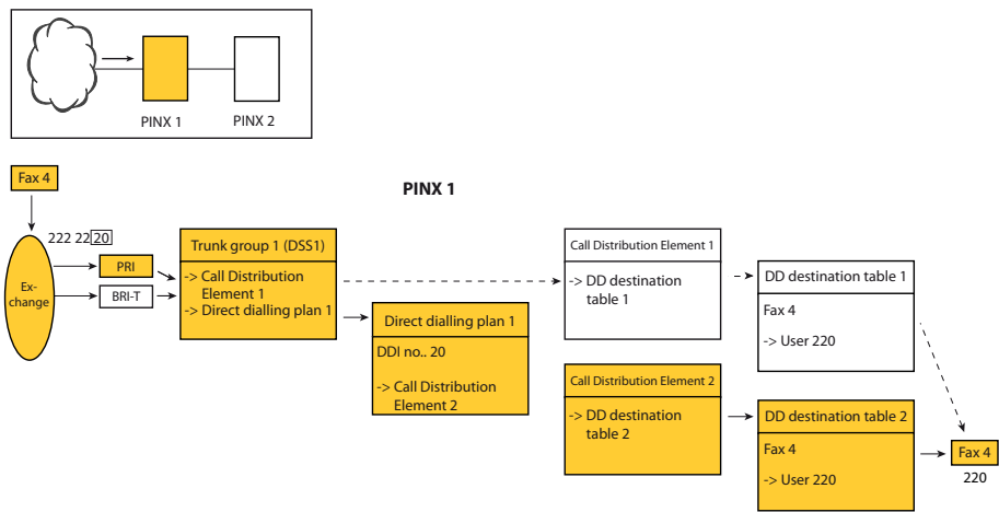
Fig. 127 Incoming data-service routing from the public network with direct dialling to a destination in the data-service destination table
