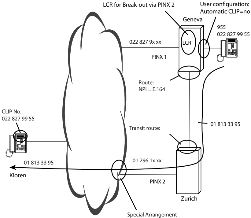
Fig. 126 Topology with important points
