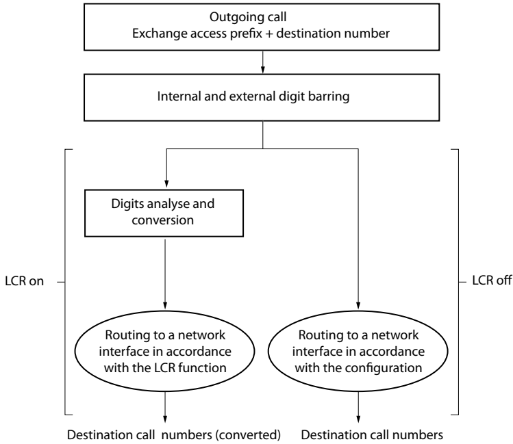
Fig. 102 Outgoing exchange traffic using LCR
