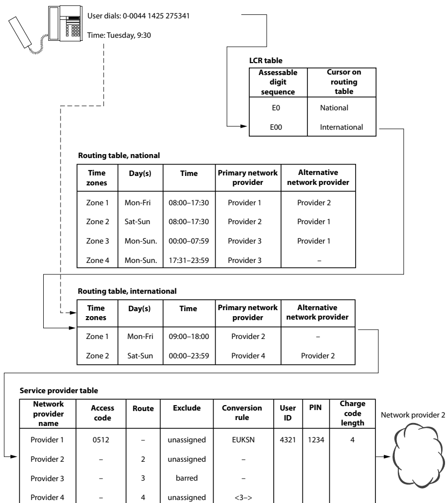
Fig. 103 Example of call routing using the LCR function
