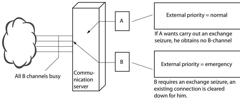
Fig. 96 Network access rights for users with and without Priority exchange allocation
