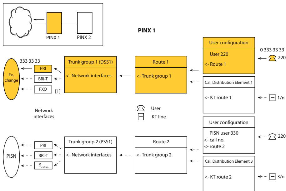
Fig. 93 Routing a call to the public network
