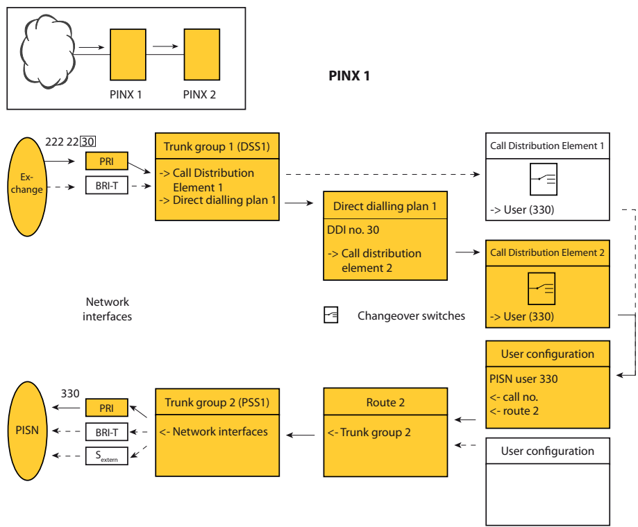
Fig. 116 Transit routing from the public network into the private leased-line network with direct dialling
