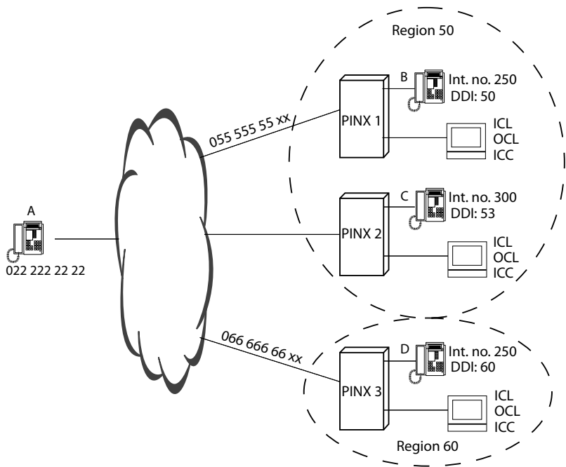
Fig. 168 PISN with two regions and shared numbering plan for Region 50
