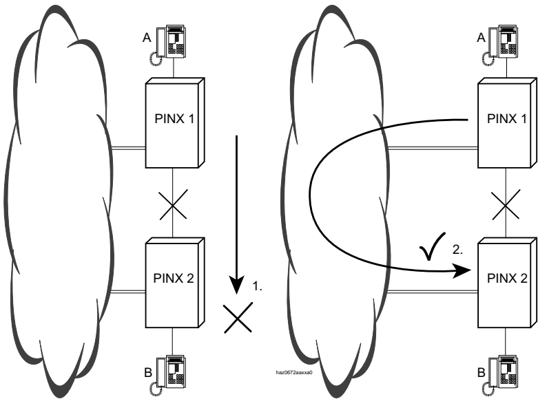
Fig. 123 Overflow via the public network -- the LCR function is used for this purpose
