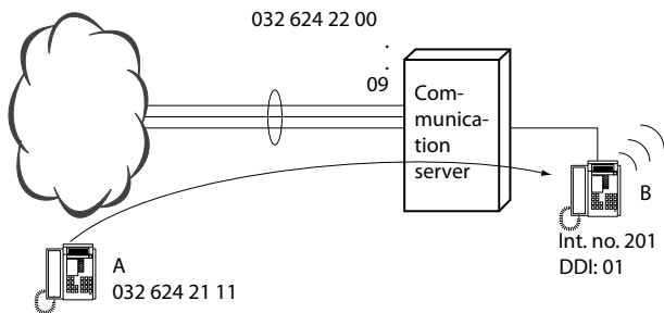
Fig. 162 Call to an absent user
