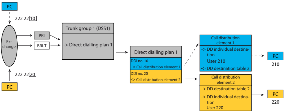
Fig. 129 Incoming data-service routing from the public network with direct dialling to a data-service individual destination but without entry in a data-service destination table
