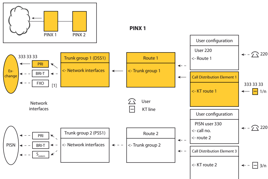
Fig. 94 Routing a call to the public network via a line key of a key telephone
