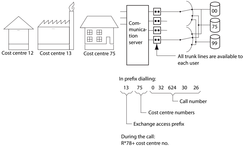
Fig. 150 Variable cost centre allocation
