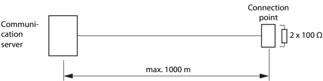
Fig. 49 S bus, point-to-point
