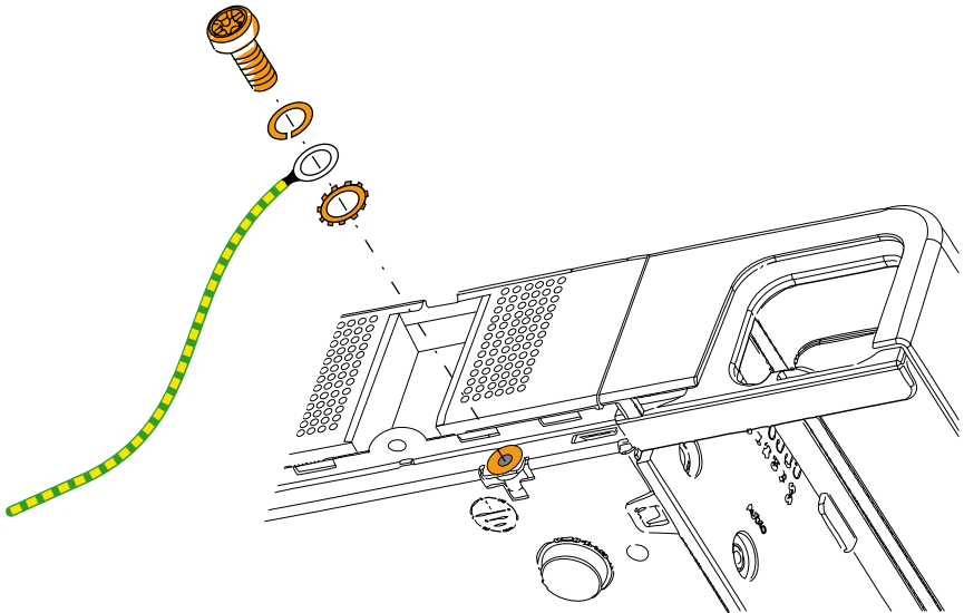
Fig. 19 Earthing connection
