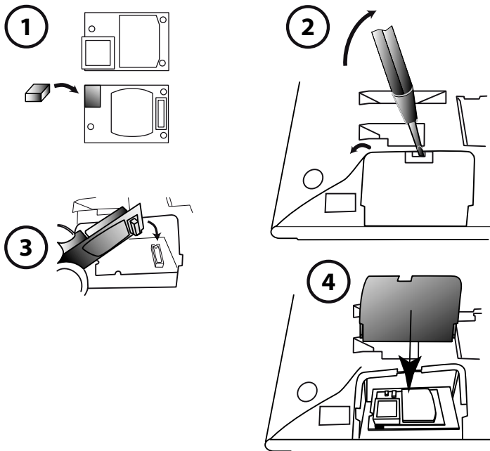
Fig. 68 Assembly of the Bluetooth module
