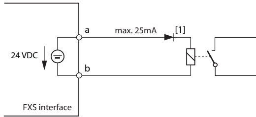
Fig. 55 Connection for FXS mode: Control output
