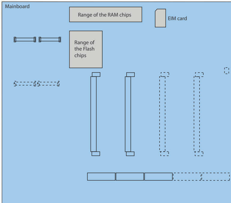
Fig. 79 Memories on the mainboard Mitel 415/430
