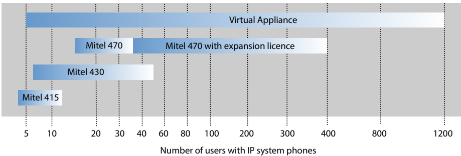
Fig. 3 MiVoice Office 400 communication servers and their expansion capacity
