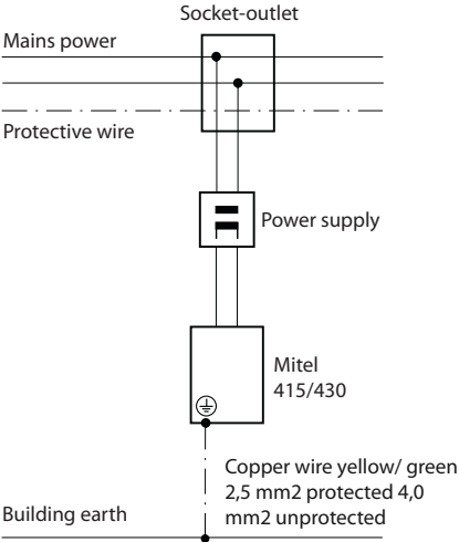
Fig. 20 Earthing of the communication server in the case of an indirect cabling and direct cabling
