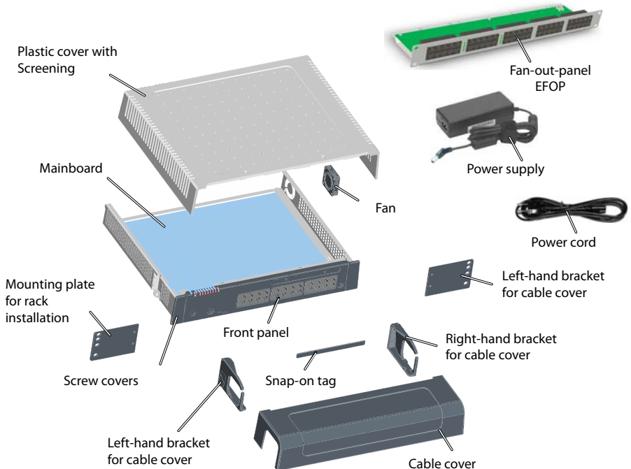
Fig. 11 System components with mounting options
