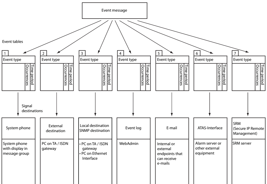
Fig. 84 Distribution principle for an event message
