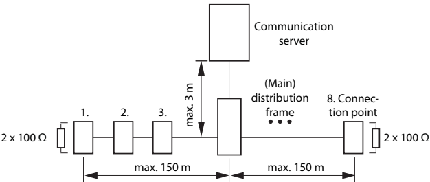
Fig. 47 S bus, short, V-shaped
