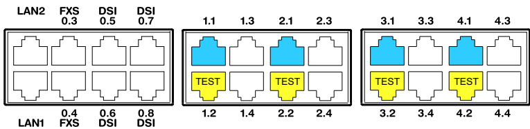
Fig. 35 Connection possibilities for PRI network interfaces
