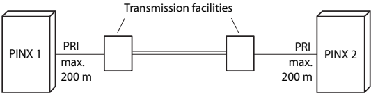
Fig. 38 Primary rate interface, networked with transmission equipment
