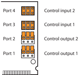
Fig. 65 Jumper configuration for control outputs and control inputs
