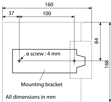
Fig. 71 Dimensional drawing for wall-mounting the mounting bracket
