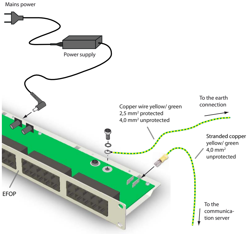
Fig. 61 Connection of an EFOP fan-out-panel
