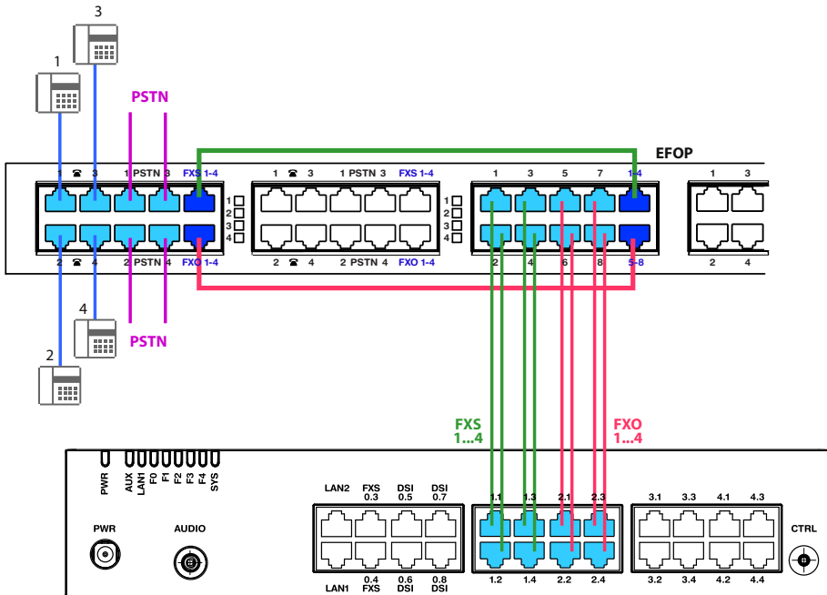
Fig. 60 Connection of EFOP fan-out-panel (example)
