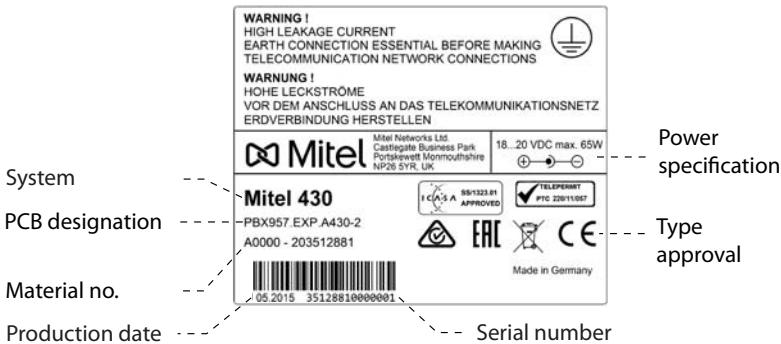
Fig. 86 Rating plate (example Mitel 430 communication server)
