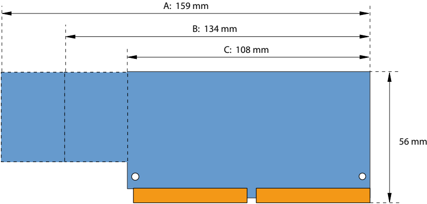
Fig. 88 Dimensions of interface cards (design A, B, C)
