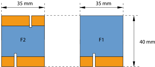
Fig. 90 Wiring adapter dimensions (design F)
