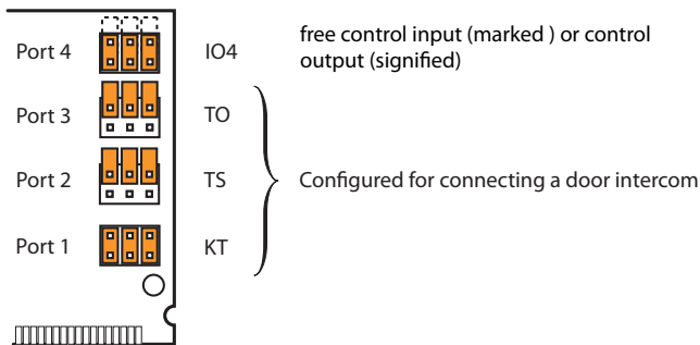
Fig. 63 Jumper configuration for connecting a door intercom
