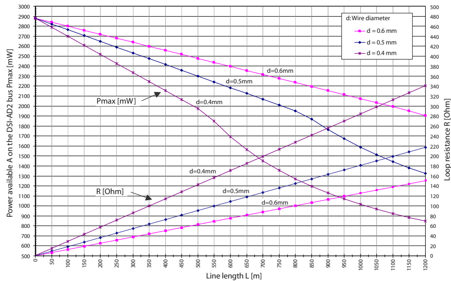
Fig. 43 Power available A on the DSI-AD2 bus
