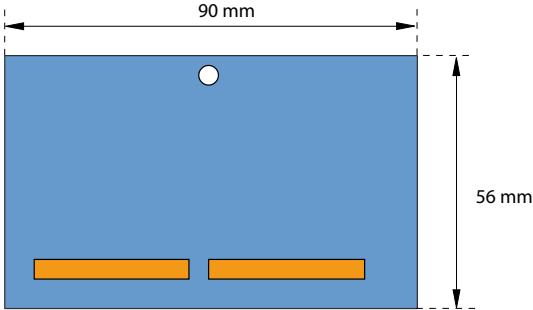
Fig. 89 Dimensions of system module (design D)
