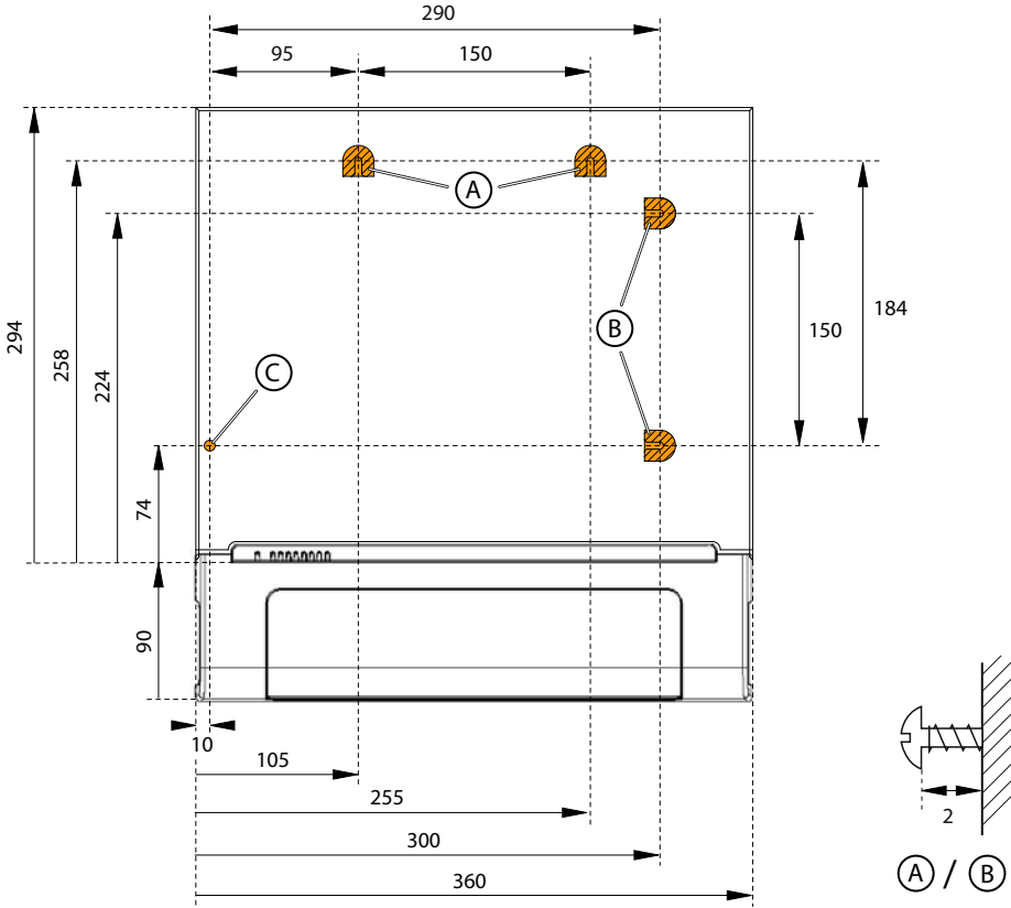
Fig. 14 Drilling plan for Mitel 415/430 wall mounting
