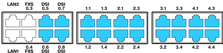
Fig. 41 Connection possibilities for DSI terminal interfaces
