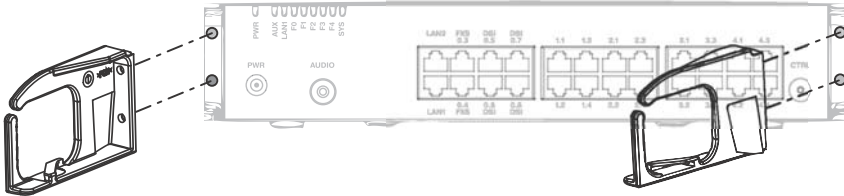
Fig. 18 Installing the brackets for the cable cover
