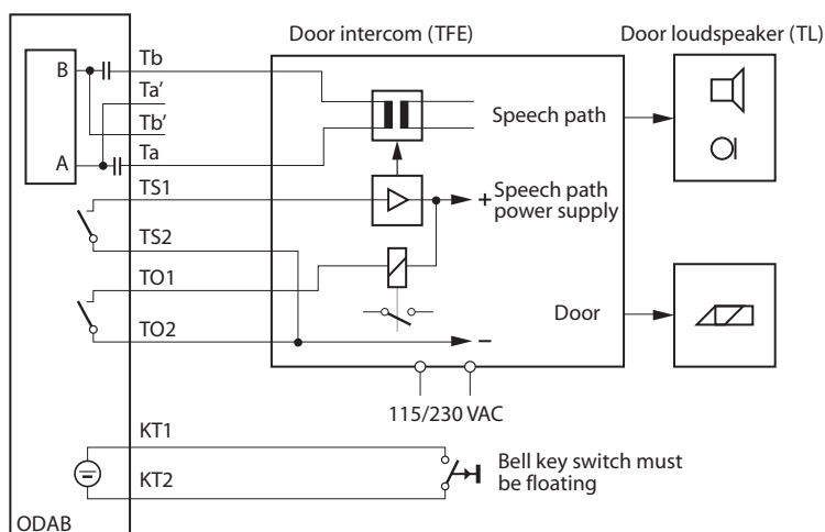
Fig. 64 Schematic circuit diagram
