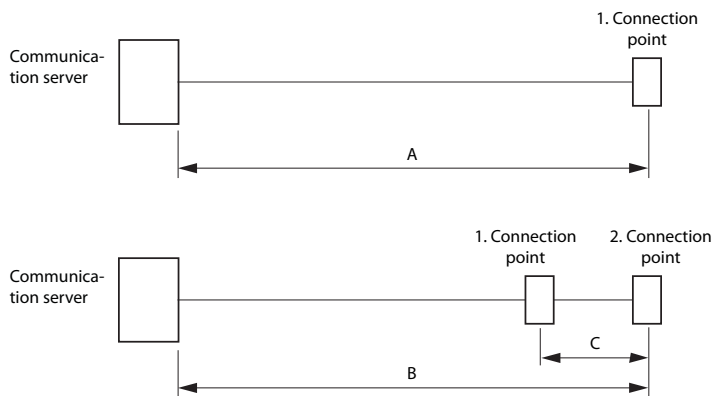
Fig. 42 DSI-AD2 bus
