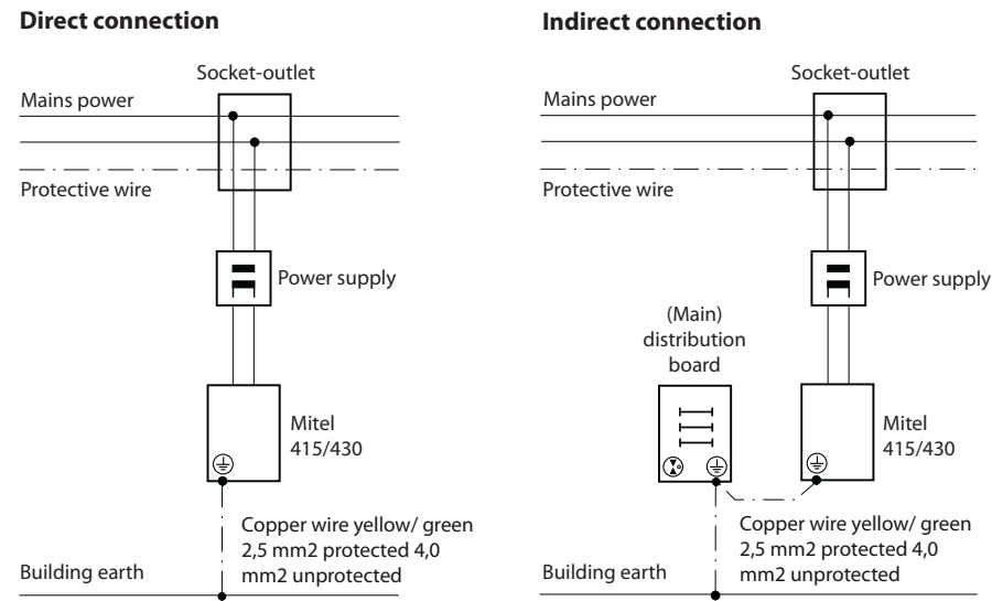
Fig. 20 Earthing of the communication server in the case of an indirect cabling and direct cabling
