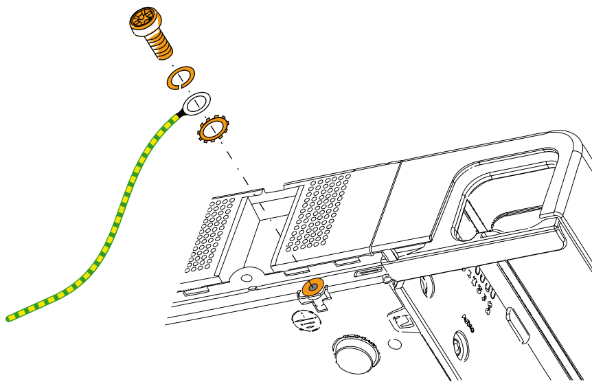
Fig. 19 Earthing connection
