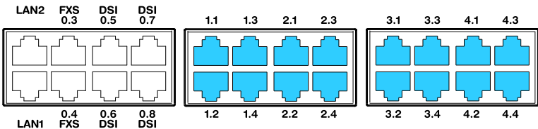
Fig. 31 Connection possibilities for BRI network interfaces
