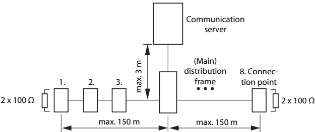
Fig. 47 S bus, short, V-shaped
