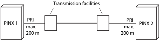
Fig. 38 Primary rate interface, networked with transmission equipment
