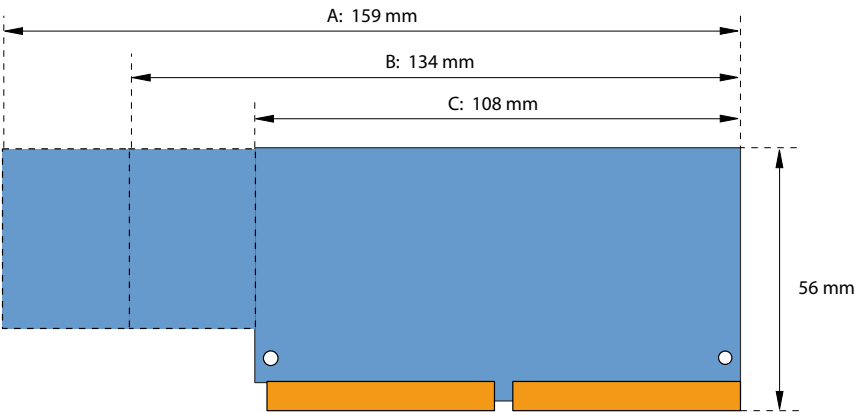
Fig. 84 Dimensions of interface cards (design A, B, C)
