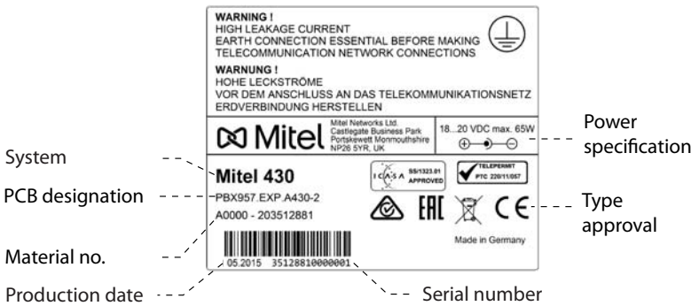
Fig. 82 Rating plate (example Mitel 430 communication server)
