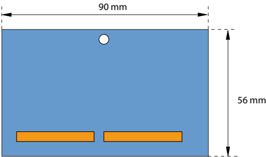
Fig. 85 Dimensions of system module (design D)
