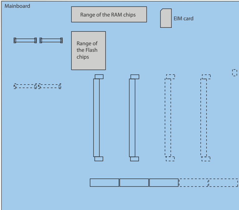
Fig. 75 Memories on the mainboard Mitel 415/430
