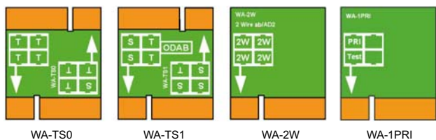
Fig. 10 Types of wiring adapters
