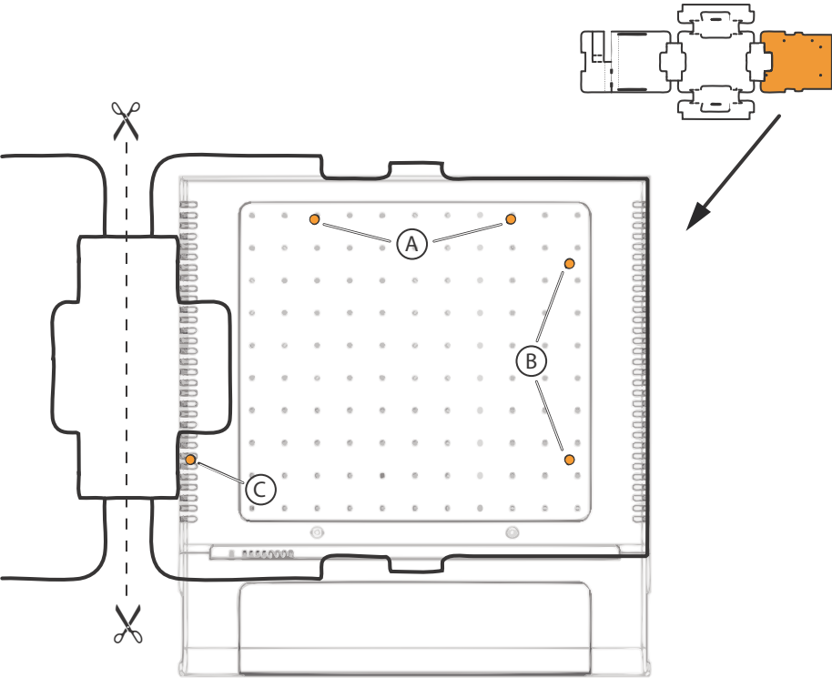
Fig. 15 Drilling template
