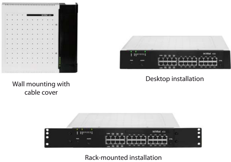
Fig. 2 Installation versions
