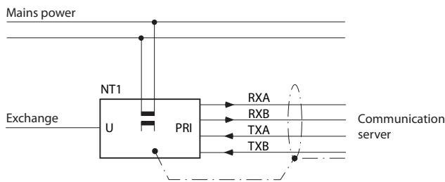
Fig. 36 PRI primary rate interface on NT1
