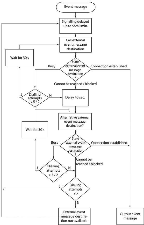
Fig. 81 Flowchart of the signalling of an event message to an external signal destination
