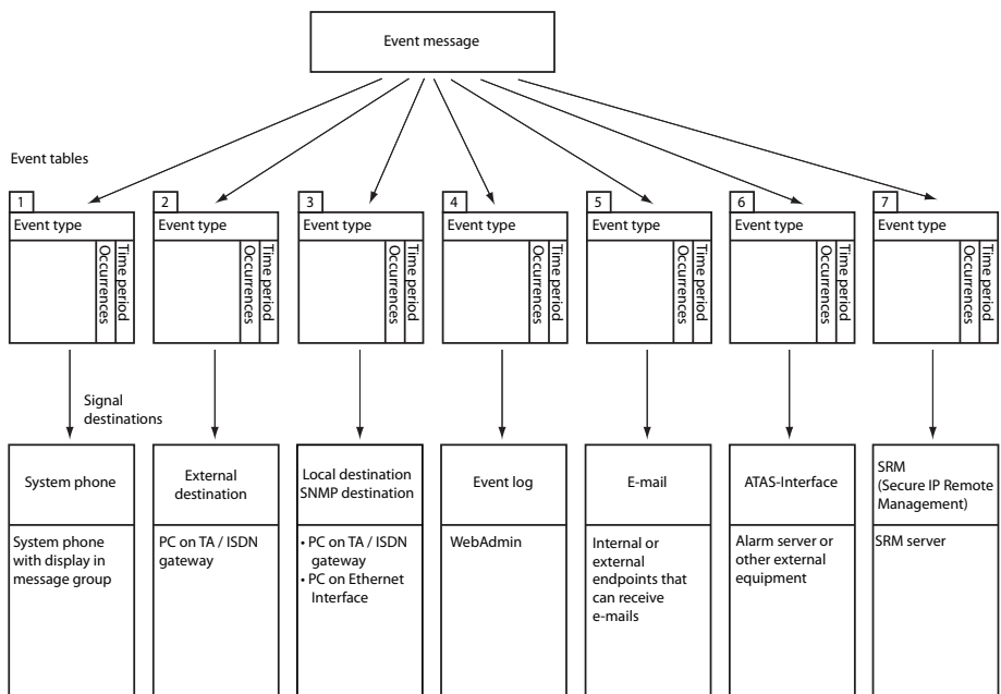
Fig. 80 Distribution principle for an event message
