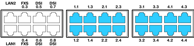
Fig. 40 Connection possibilities for FXO network interfaces
