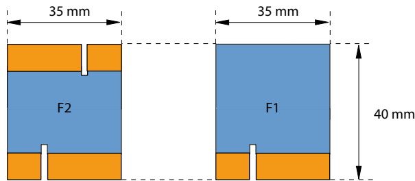
Fig. 86 Wiring adapter dimensions (design F)
