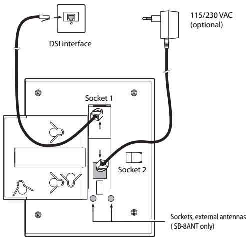
Fig. 74 Underside of the radio units with connection points
