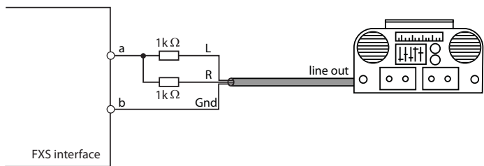
Fig. 60 Connection for FXS mode: External audio source
