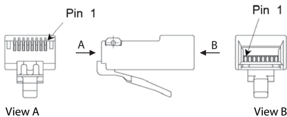
Fig. 31 Pin numbering, RJ45 connector
