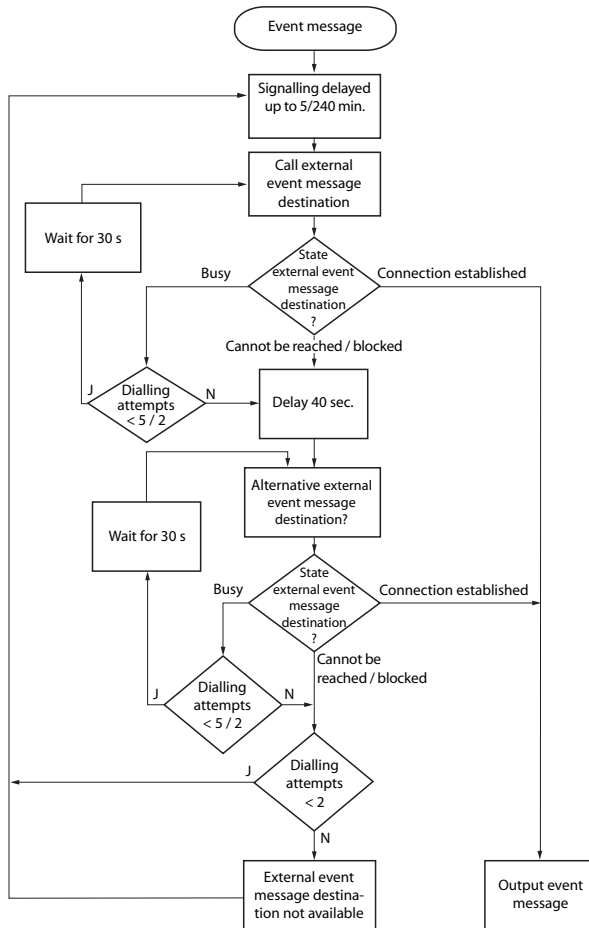
Fig. 88 Flowchart of the signalling of an event message to an external signal destination
