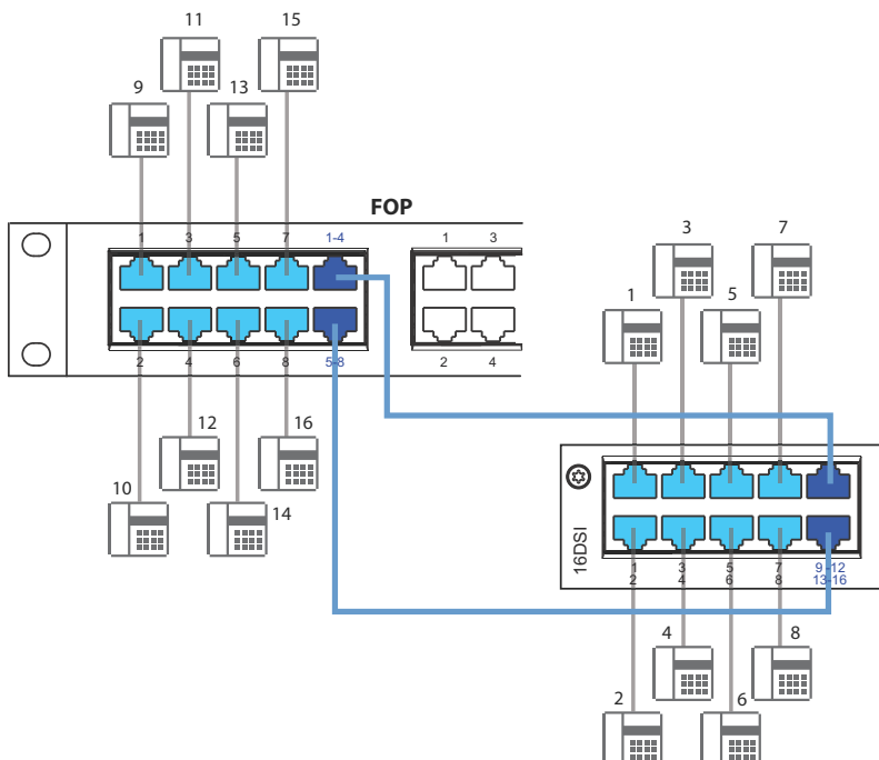
Fig. 65 Connection of four-fold assigned sockets via FOP connector strip
