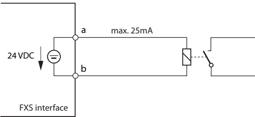
Fig. 61 Connection for FXS mode: Control output
