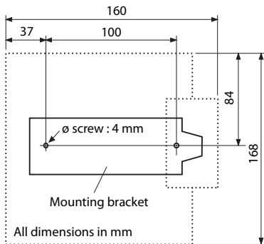
Fig. 72 Dimensional drawing for wall-mounting the mounting bracket
