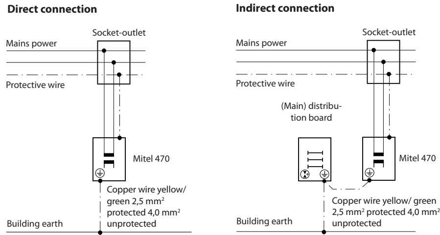
Fig. 22 Earthing of the communication server in the case of direct cabling and indirect cabling
