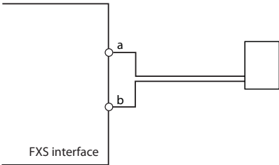
Fig. 59 Connection for FXS mode: 2-wire door
