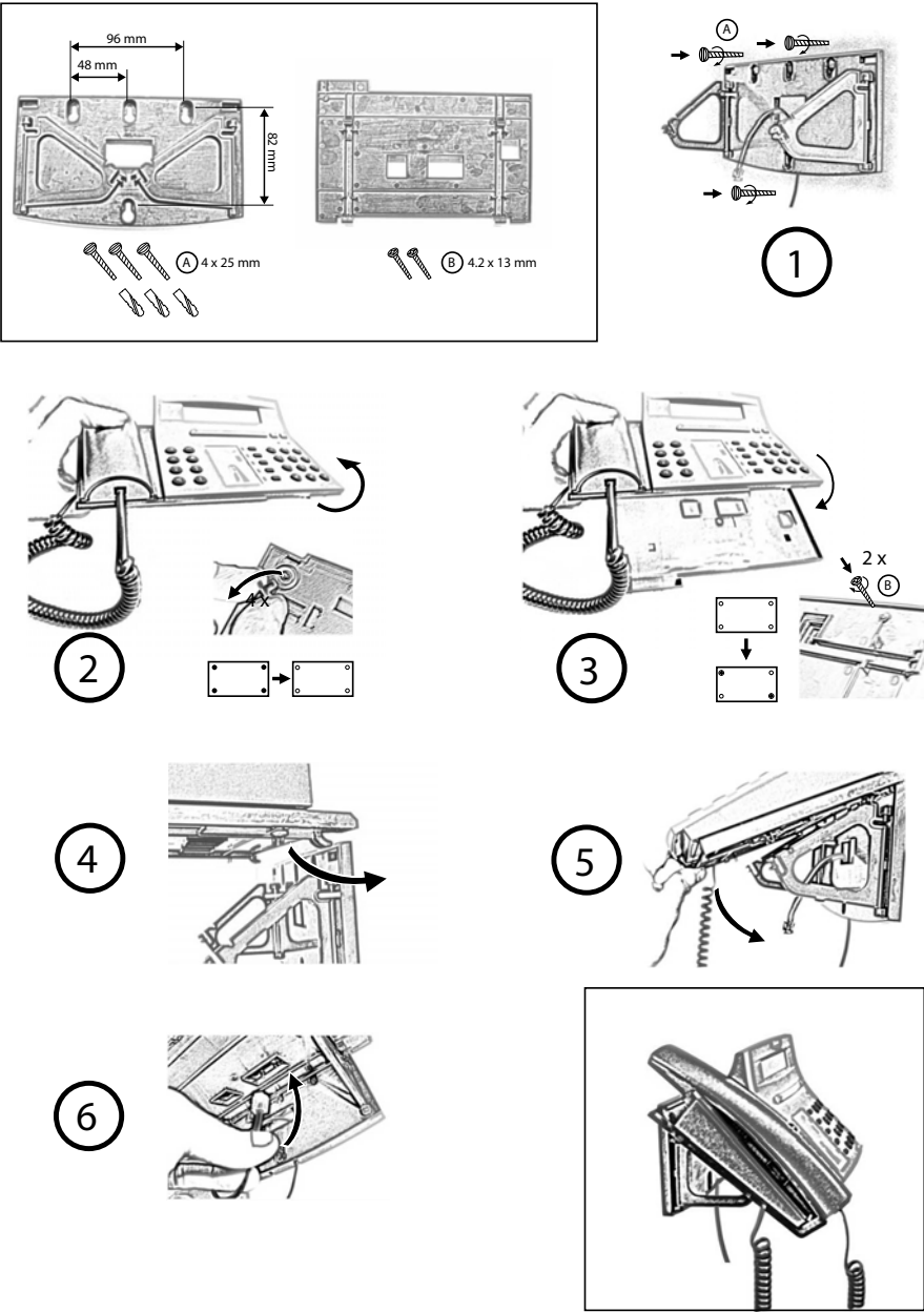
Fig. 70 Wall mounting of Office 25 and Office 35
