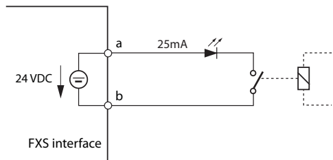
Fig. 62 Connection for FXS mode: Control input
