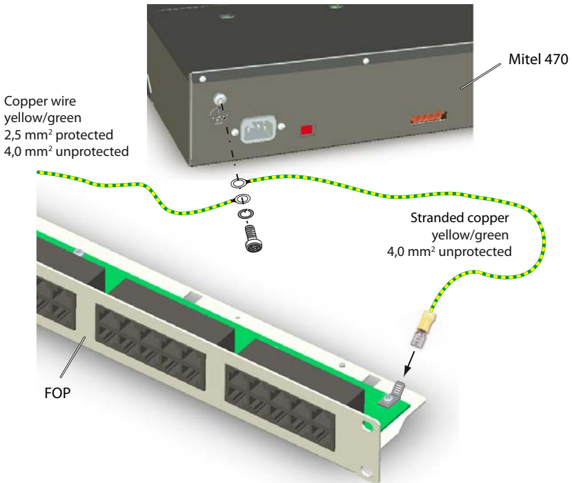
Fig. 66 Connection of the FOP fan-out-panel to the protective earth
