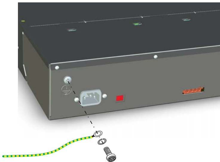
Fig. 21 Earthing connection
