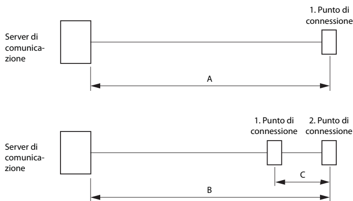
Fig. 42 Bus DSI-AD2
