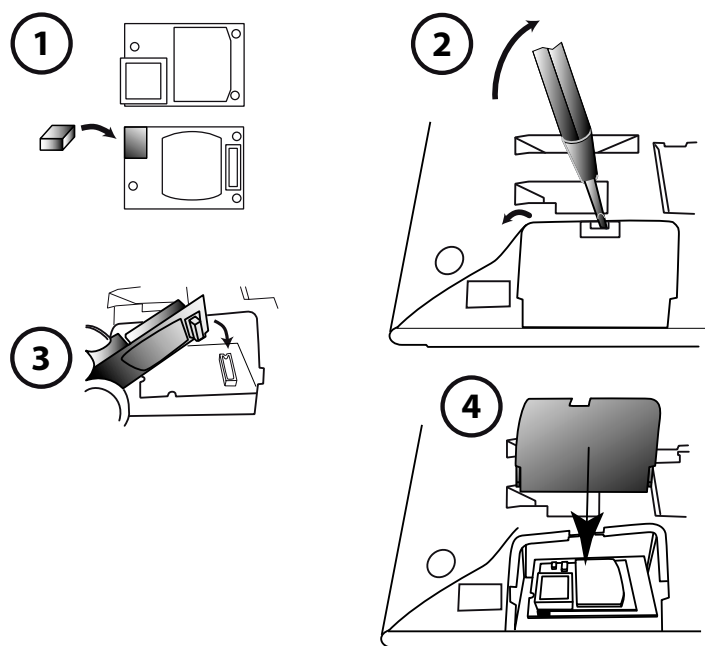
Fig. 64 Montage Bluetooth-Modul
