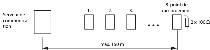
Fig. 50 Bus S court
