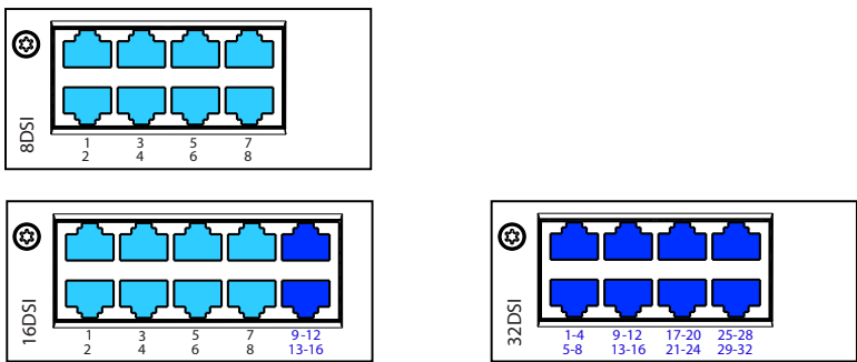
Fig. 45 Connection possibilities for DSI terminal interfaces
