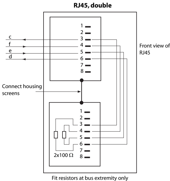
Fig. 55 RJ45 connection, double socket
