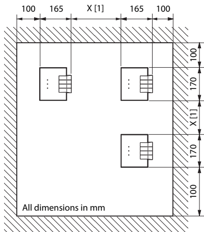
Fig. 70 Dimensional drawing for wall-mounting the mounting bracket
