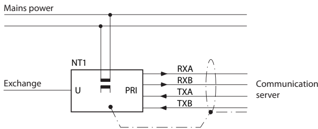
Fig. 40 PRI primary rate interface on NT1
