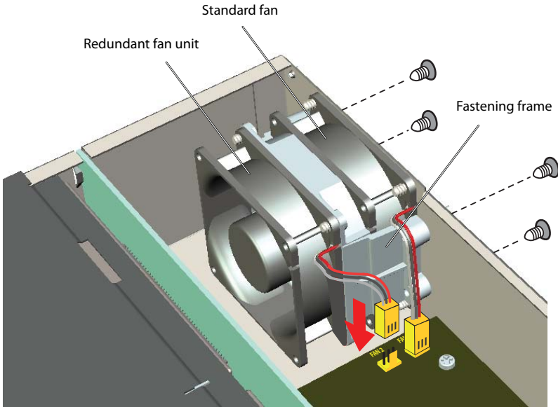
Fig. 19 Fitting the additional fan in Mitel 470
