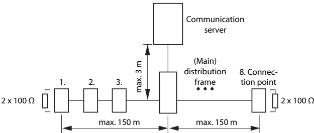
Fig. 51 S bus, short, V-shaped
