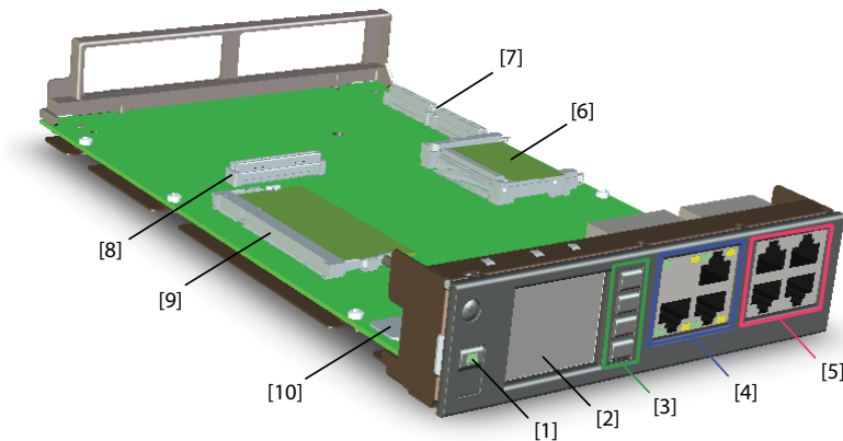
Fig. 9 Interfaces, display and control elements of the call manager card CPU1
