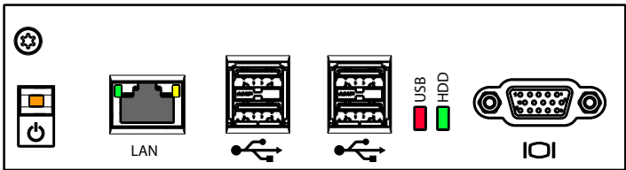
Fig. 84 Status LEDs on the applications server
