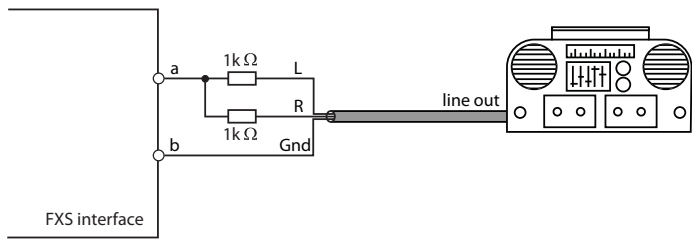
Fig. 61 Connection for FXS mode: External audio source
