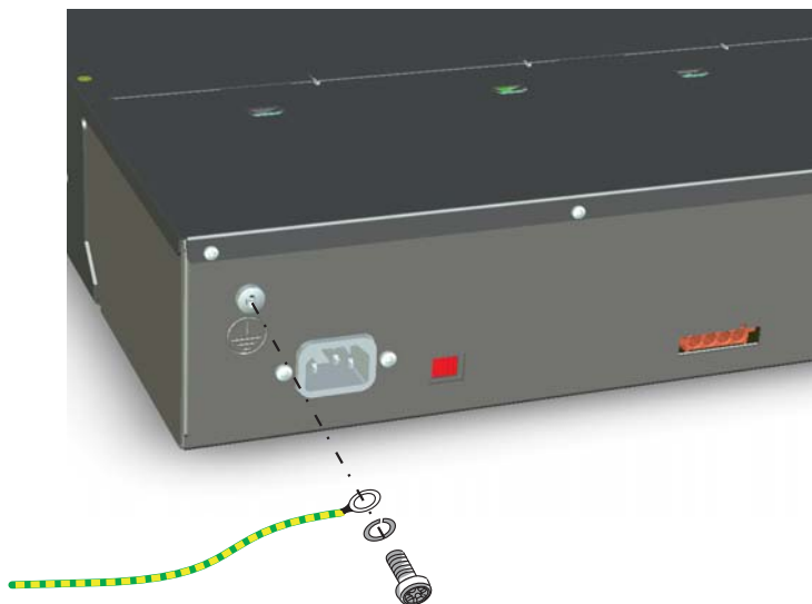
Fig. 21 Earthing connection
