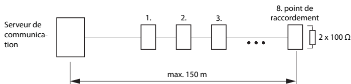
Fig. 46 Bus S court
