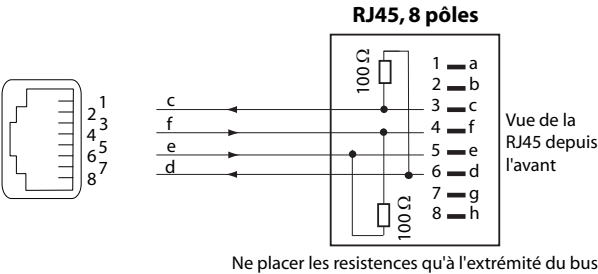
Fig. 50 Raccordement RJ45, prise simple
