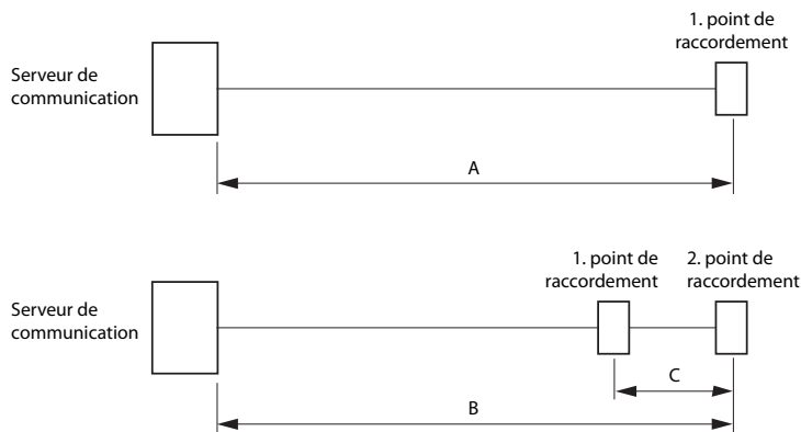
Fig. 42 Bus DSI-AD2
