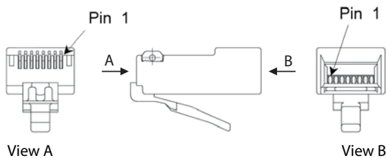
Fig. 31 Pin-nummering, RJ45 connector
