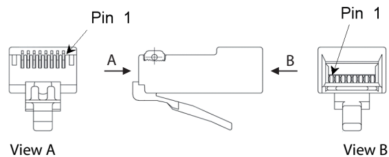
Fig. 25 Pin-nummering, RJ45 connector
