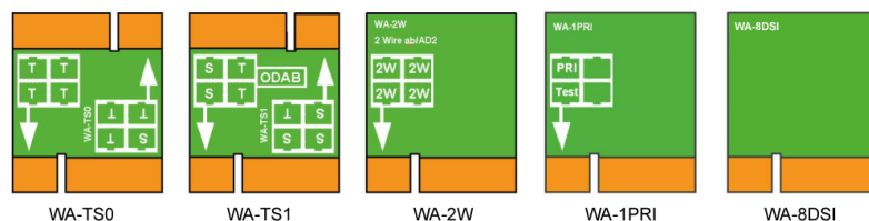
Fig. 10 Types bedradingsadapters
