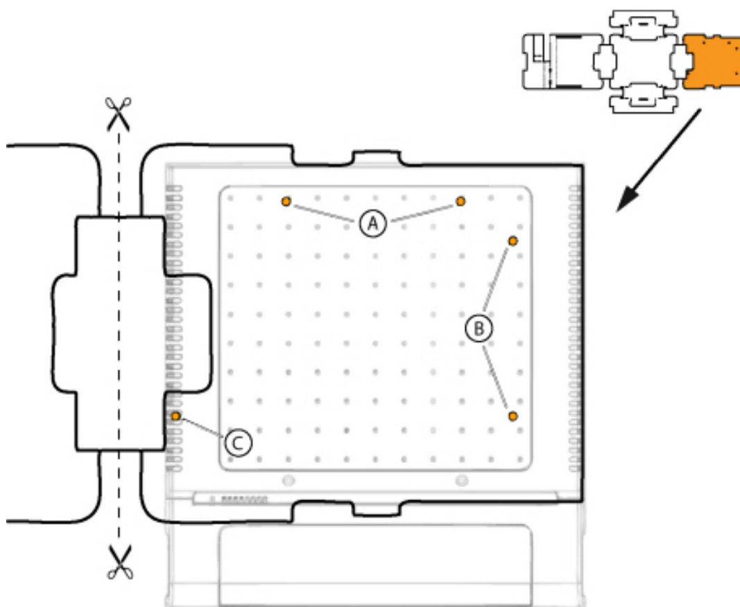
Figure 13: Boorsjabloon
