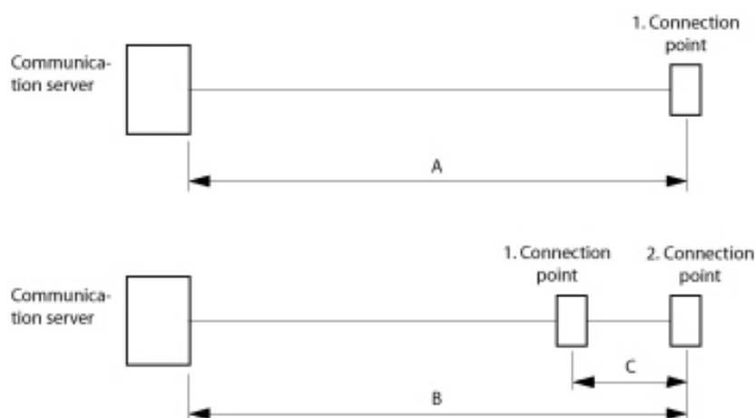
Figure 38: DSI-AD2 bus
