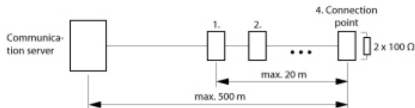
Figure 44: S-bus, lang
