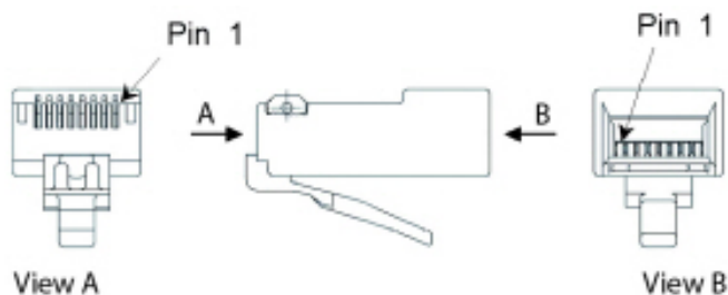
Figure 30: Pin-nummering, RJ45 connector
