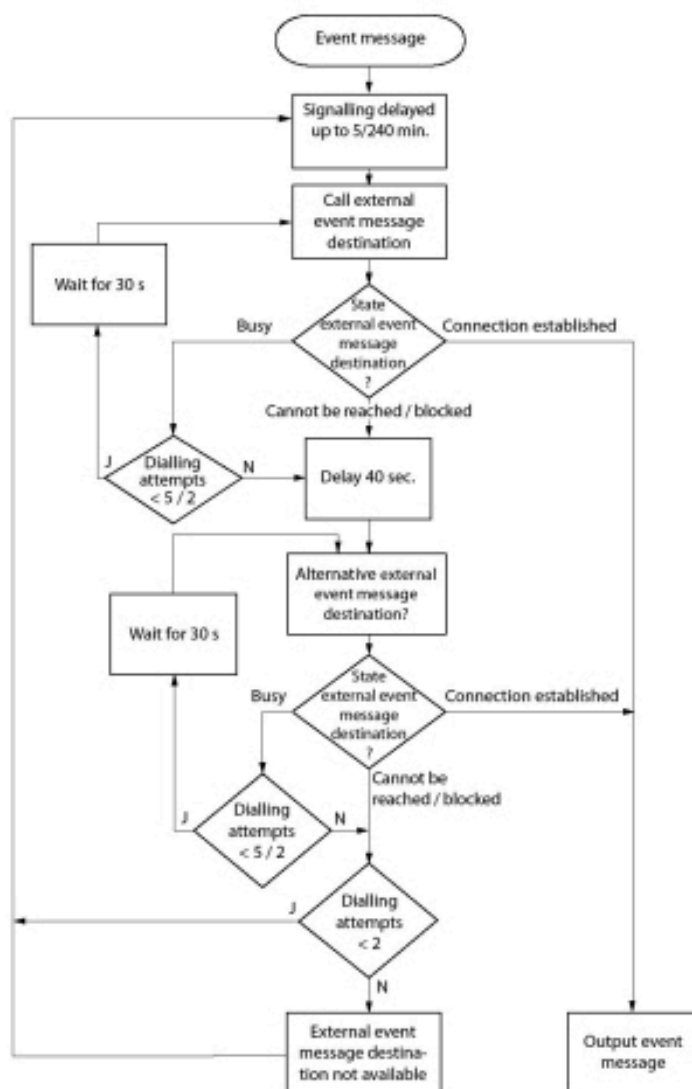
Figure 8: Flowchart of the signalling of an event message to an external signal destination
