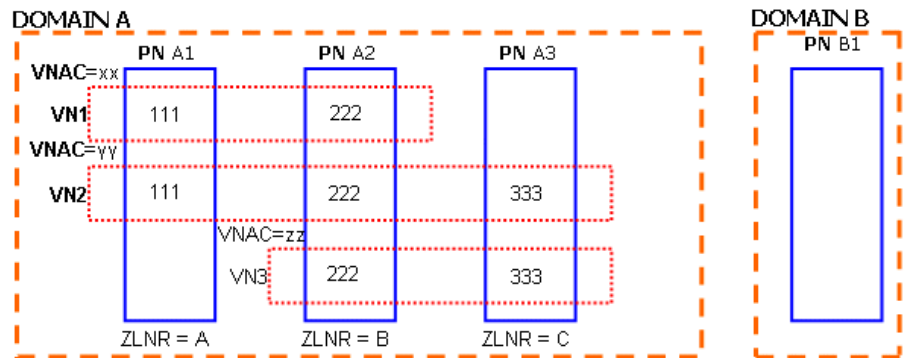
Figure 101: VNR Network
