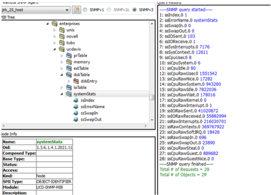
Figure 148: systemStats OID
