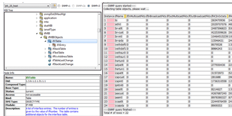
Figure 156: ifXTable
