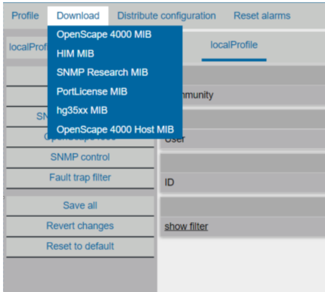
Figure 185: Download Menu
