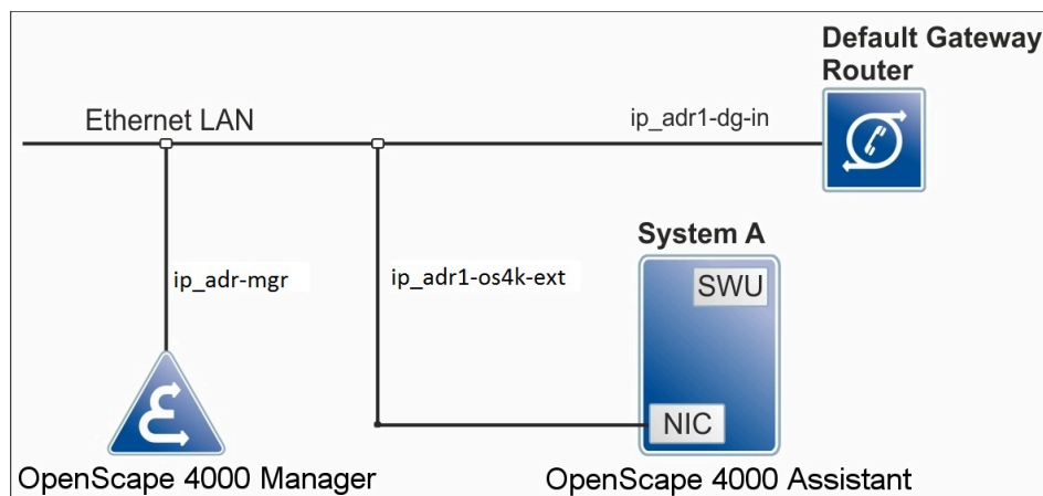
Figure 46: OpenScape 4000 Manager and OpenScape Assistant in the Same Network
