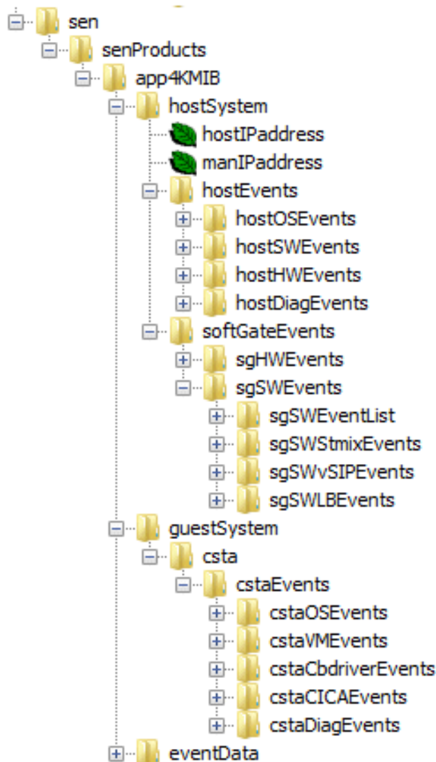
Figure 129: Host 4000 MIB Structure
