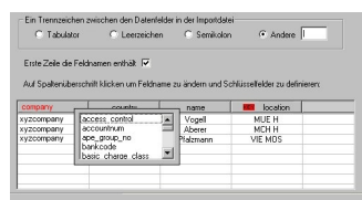
Abbildung 25: Editing Field Names in the Import Table
