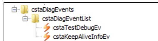
Figure 34 cstaDiagEvents
