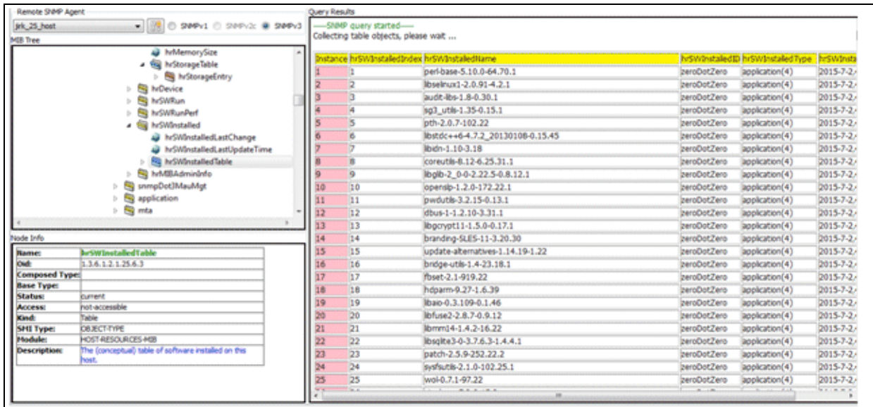
Figure 47 hrSWInstalled
