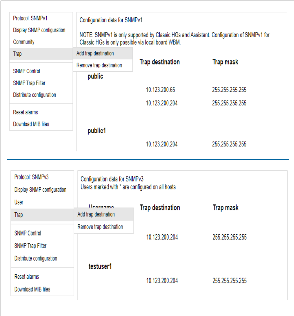
Figure 8 SNMPv1/v3 Configuration – Trap settings
