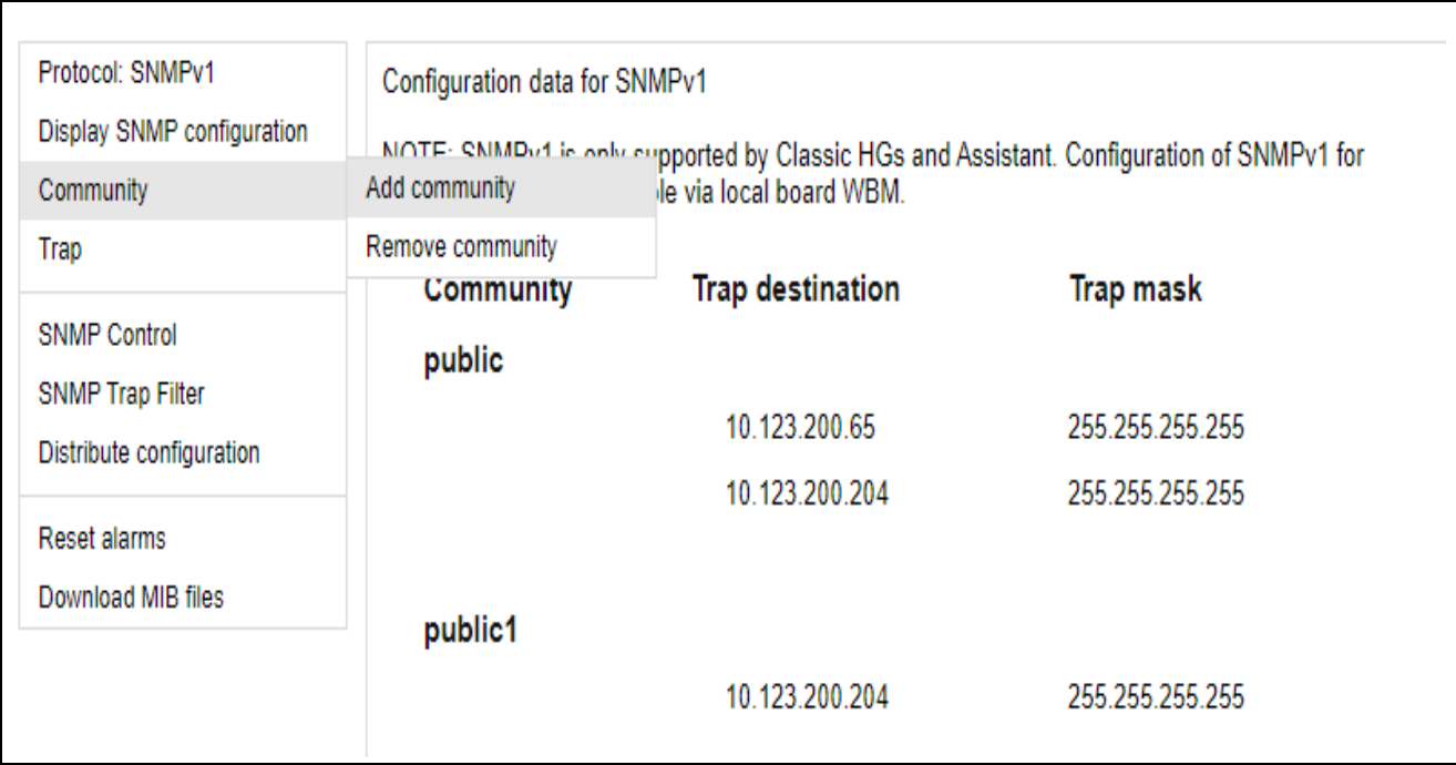
Figure 5 SNMPv1 Configuration – Community
