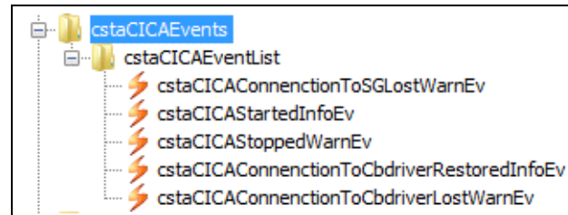
Figure 33 cstaCICAEvents
