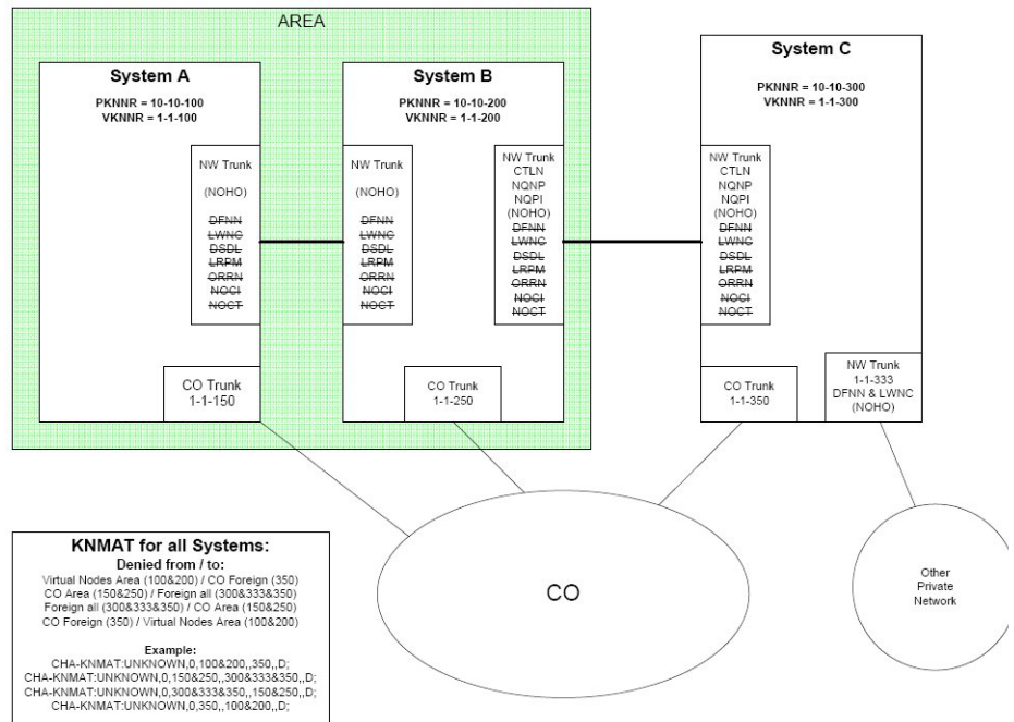
Figure 1 Network example for logical partitioning (IND)
