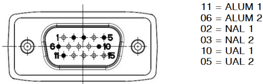
Figura 223: Pin-out de ALUM:
